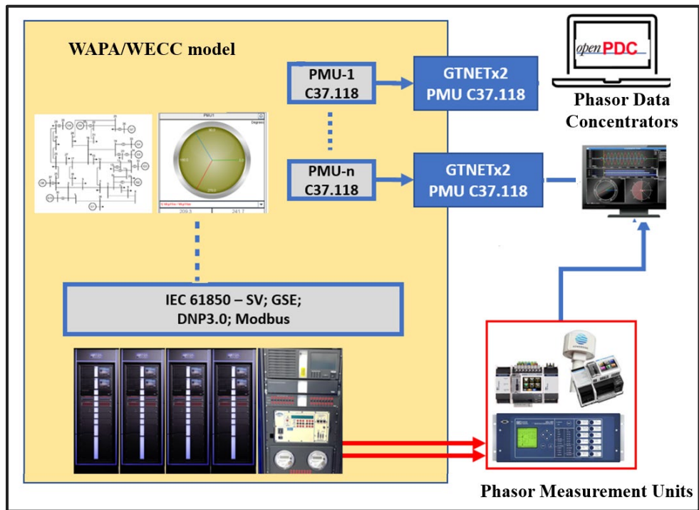
Figure 4-8. WECC reduced order model and CHIL interface of the PMUs.
