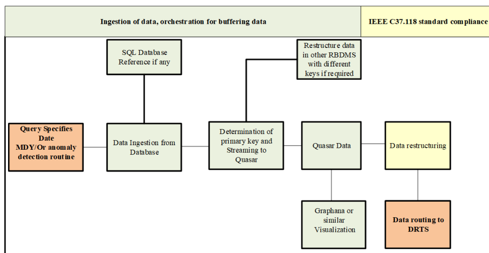
Figure 4-6. WAPA raw data streaming to DRTS – database management
