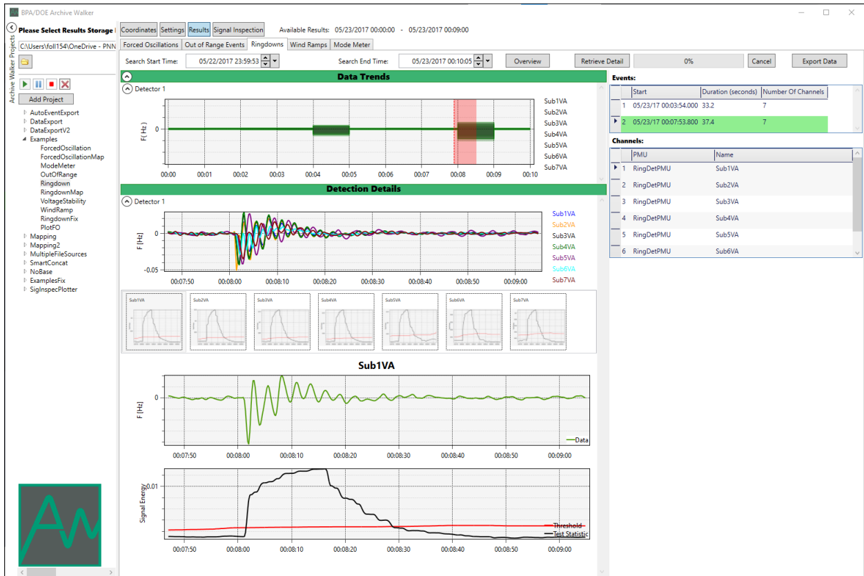
Figure 2-3. Screen capture of the Archive Walker user interface showing the detection of an oscillation in PMU measurements.
