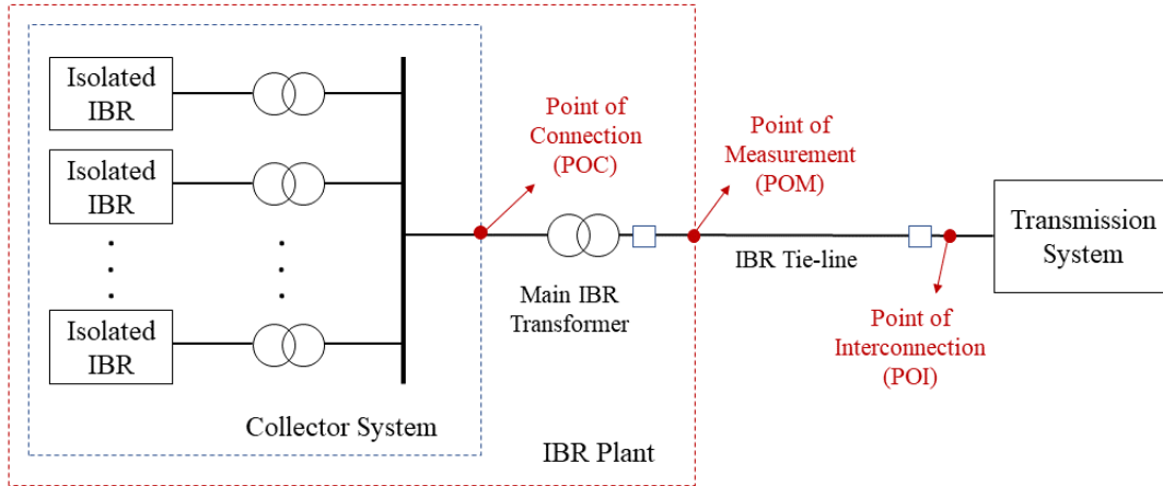
Figure 2-1. Conceptual diagram describing the terms POC, POM, POI. Adapted from IEEE 2800 Std (IEEE, 2022).
