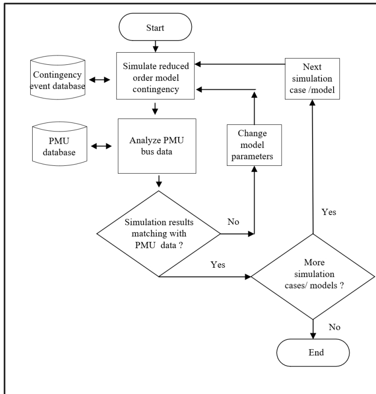
Figure 4-4. Typical model validation process
