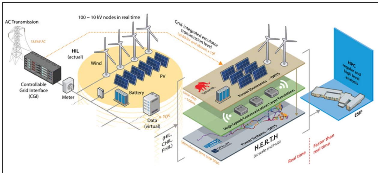
Figure 4-5. NREL's ARIES Facility
