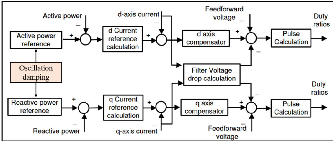
Figure 4-3. Notional IBR oscillation damping control architecture
