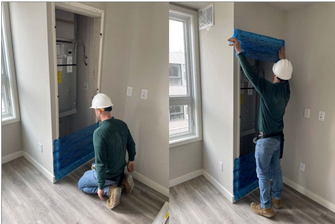
Figure 10. Supplemental test in modular unit 4 to determine air leakage through HVAC cabinet
