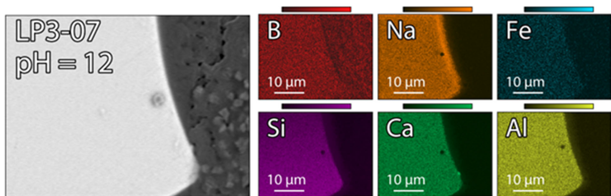
Figure C-7. LP3-07 glass after 2 Day EPA 1313 with pH = 12
