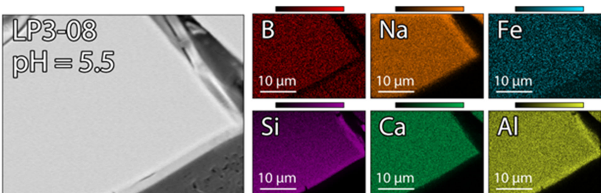
Figure C-9. LP3-08 glass after 2 Day EPA 1313 with pH = 5.5
