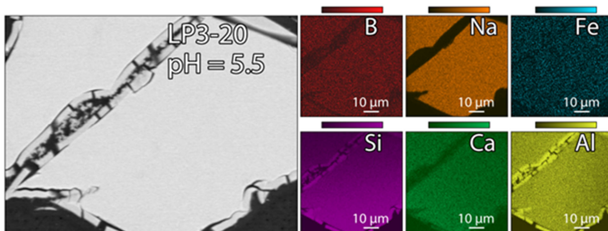
Figure C-17. LP3-20 after 2 Day EPA 1313 with pH = 5.5
