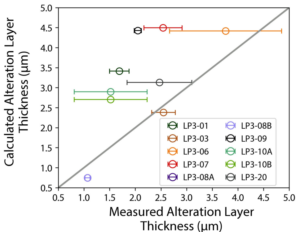
Figure B-3. Comparison of EPMA measured alteration layer thickness and calculated equivalent layer thicknesses for LAW glasses tested by EPA 1313 at pH = 5.5 \pm 1 based on the normalized release of B.
