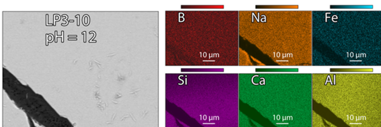
Figure C-16. LP3-10 glass after 2 Day EPA 1313 with pH = 12
