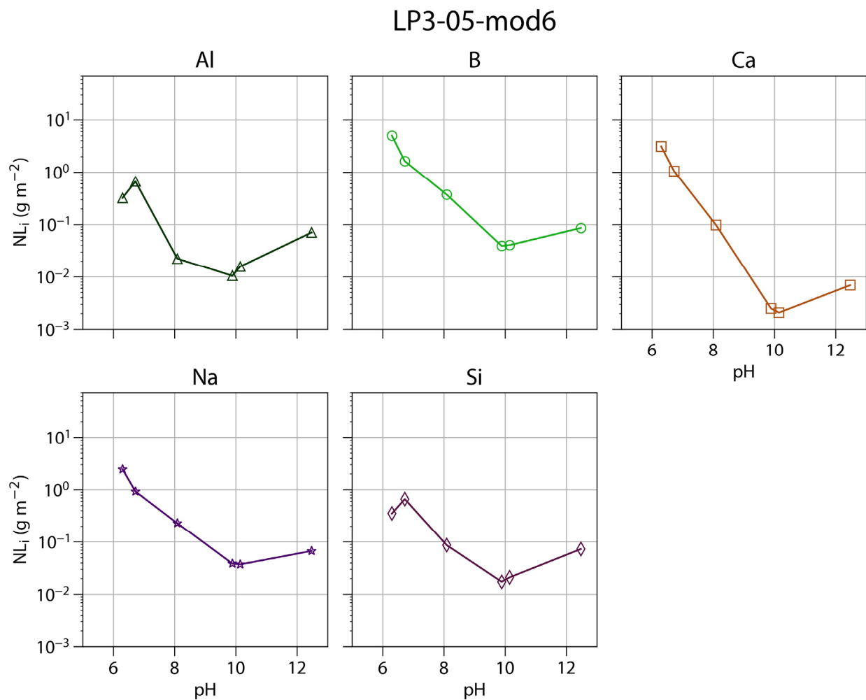
Figure B-19. EPA 1313 normalized elemental releases of Al, B, Ca, Na, and Si for LP3-05mod6
