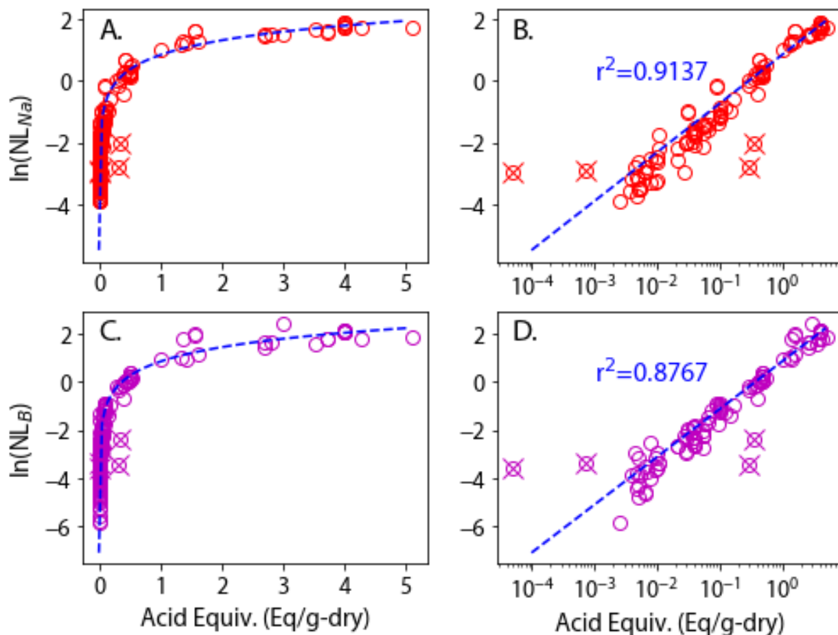
Figure 3-8. (A) \ln(NL_{Na}) values vs acid equivalents. (B) semilog plot of \ln(NL_{Na}) values versus the logarithm of acid addition. (C) \ln(NL_B) values vs acid equivalents. (D) semilog plot of \ln(NL_B) values versus the logarithm of acid addition. Outliers are shown with X's.
