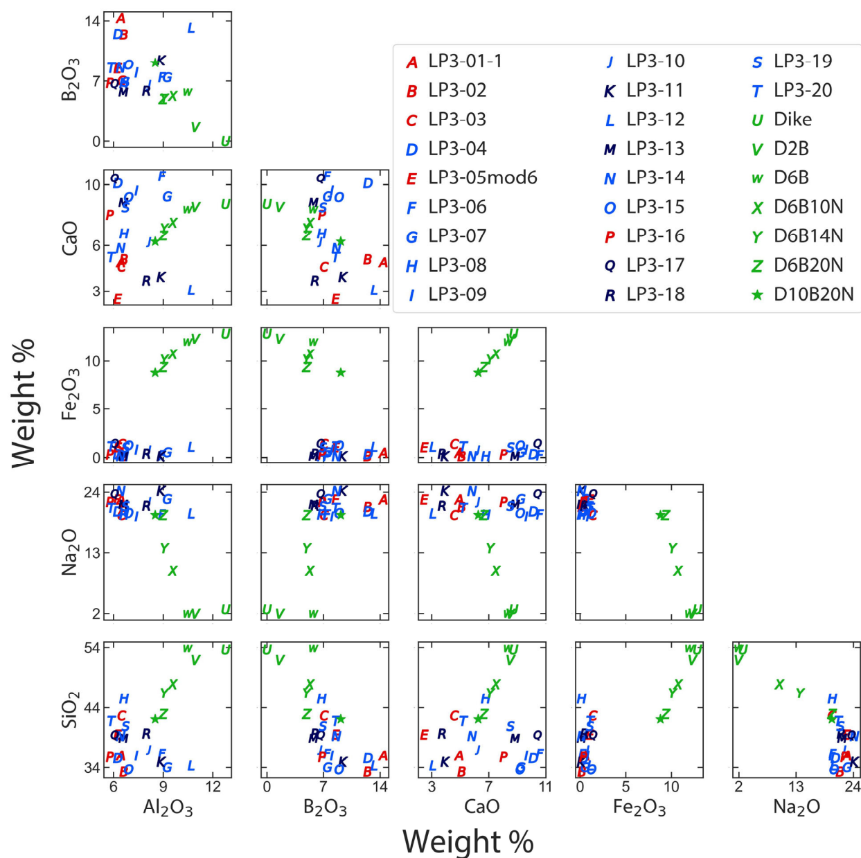
Figure 1-2. Scatterplot matrix of major elements in the LP3 compositional matrix with the “join” glasses. Glasses LP3-11, -13, -17, and -18 were not tested in the present study but compositions were taken from (Loneragan et al. 2020) are shown in dark blue. Blue symbols denote glasses are below the 2 g m -2 PCT response limit, red symbols denote glasses are above the PCT response limit, and green symbols denote join glasses
