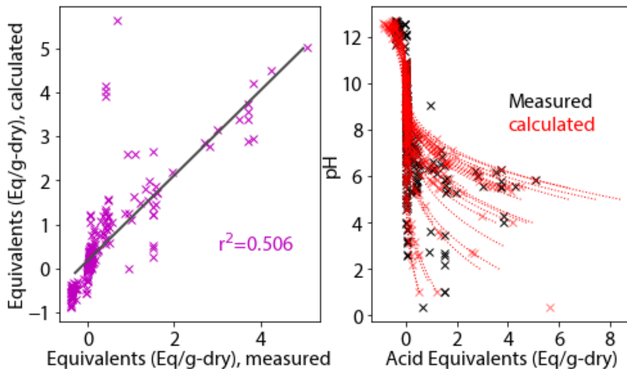
Figure A-4. (left) Comparison of measured acid equivalents to compositional ANN model #2 using a cubic fitting function and (right) titration curves for LP3 glasses and join glasses. The solid line on the left is the unity line.
