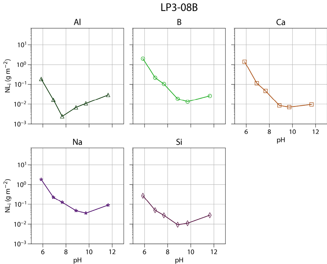
Figure B-23. EPA 1313 normalized elemental releases of Al, B, Ca, Na, and Si for LP3-08 (trial#2)
