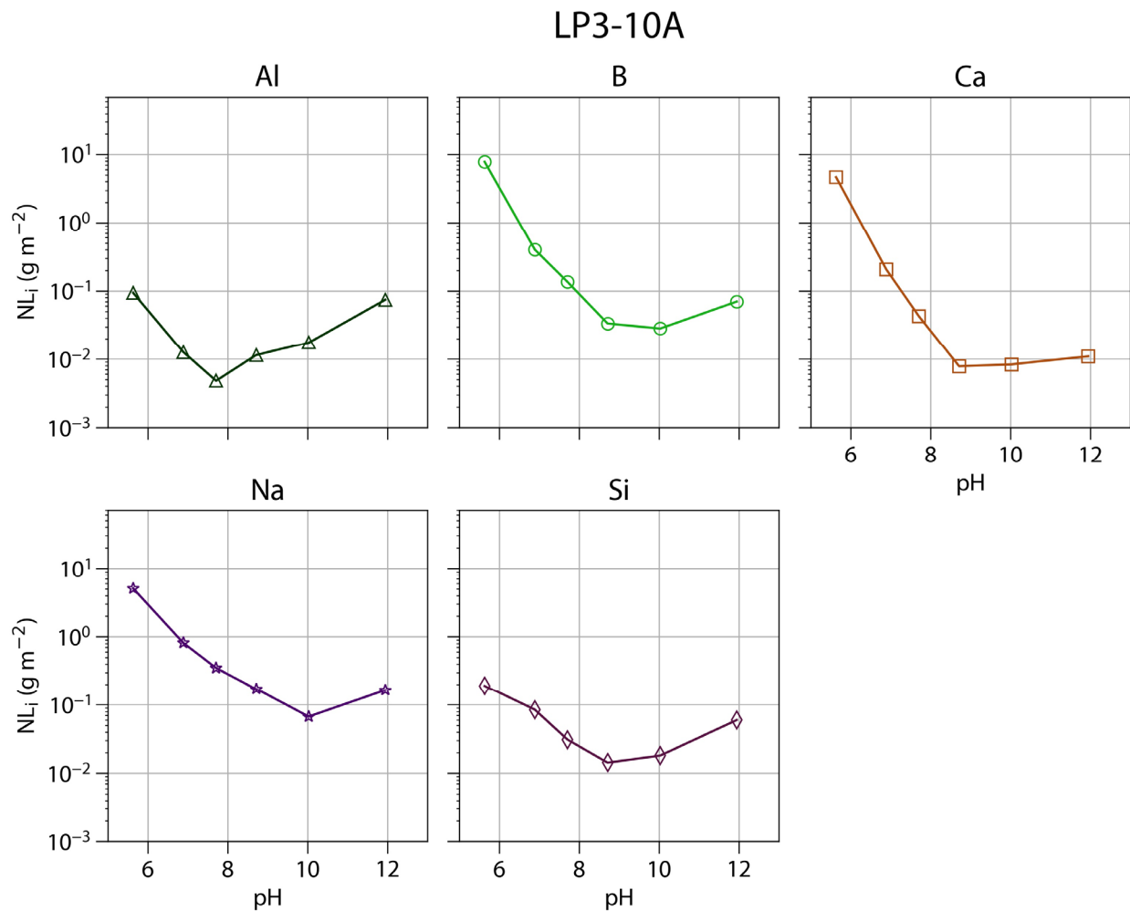
Figure B-25. EPA 1313 normalized elemental releases of Al, B, Ca, Na, and Si for LP3-10 (trial#1)
