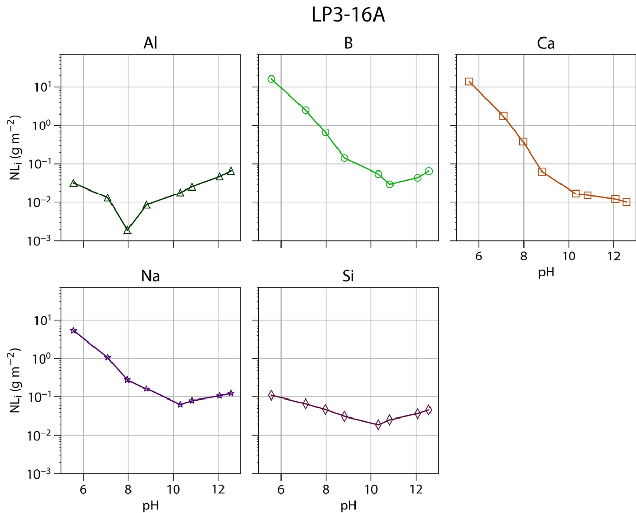
Figure B-31. EPA 1313 normalized elemental releases of Al, B, Ca, Na, and Si for LP3-16 (trial #1)
