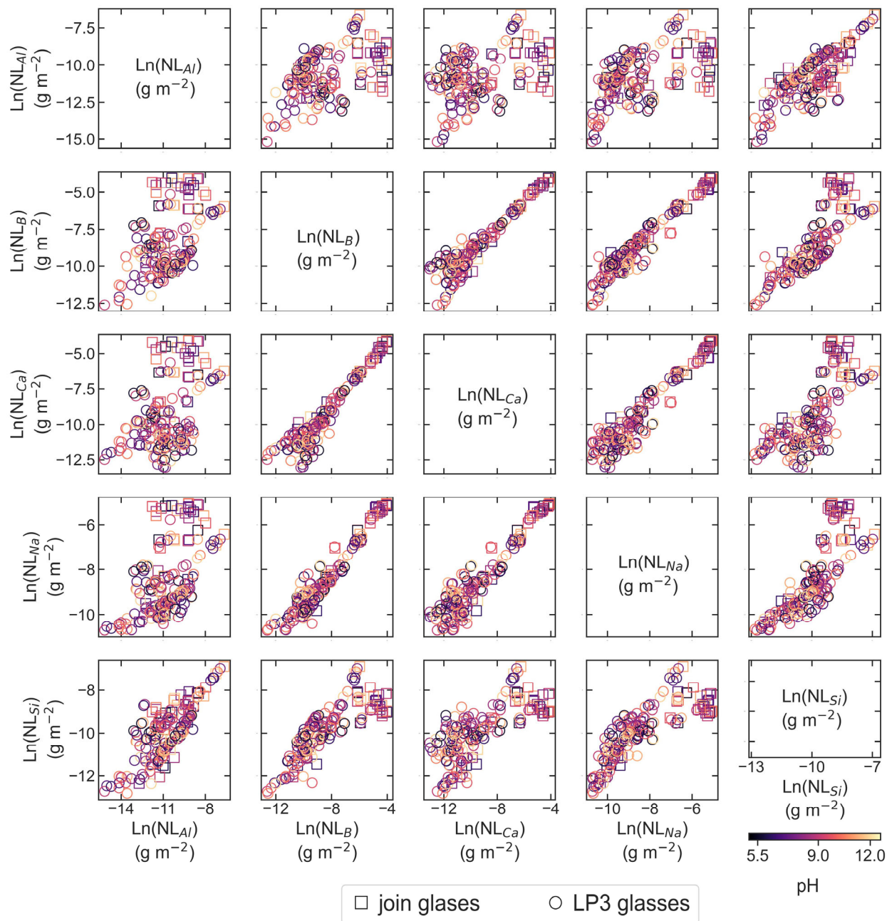
Figure 3-5. Pairwise distribution of the natural log of normalized elemental releases for LP3 and join glasses. In this figure, LP3 glasses are shown using circles and join glasses are shown using squares. The color of each data point represents the pH of the final solution, as indicated with the color bar on the bottom right
