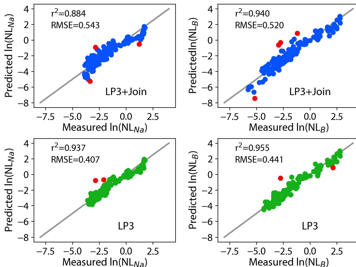
Figure 3-7. Comparison of measured versus calculated NL_{Na} values (left columns) and NL_B values (right columns) from EPA 1313 of LP3 glasses. The solid line represents the unity line. Outliers are shown in red
