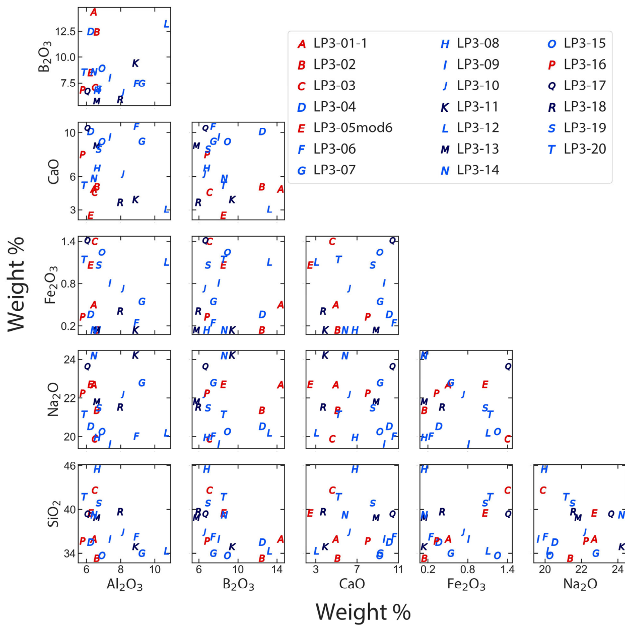
Figure 1-1. Scatterplot matrix of major elements in the LP3 compositional matrix. Glasses LP3-11, -13, -17, and -18 were not tested in the present study but compositions were taken from (Lonergan et al. 2020) are shown in dark blue. Blue symbols denote glasses are below the 2 g m -2 PCT response limit, red symbols denote glasses are above the PCT response limit.
