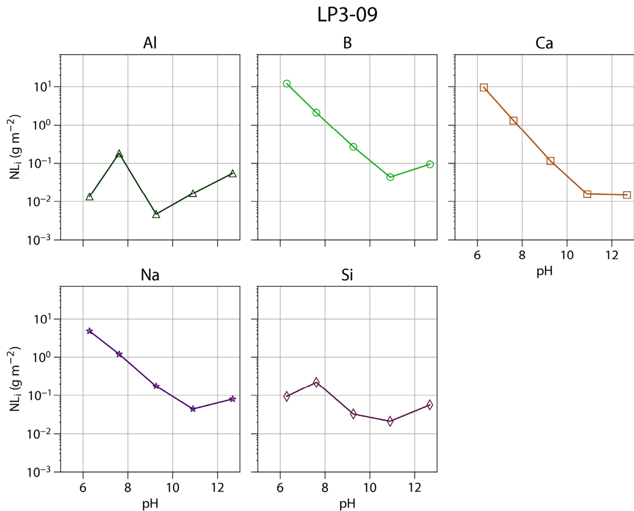
Figure B-24. EPA 1313 normalized elemental releases of Al, B, Ca, Na, and Si for LP3-09
