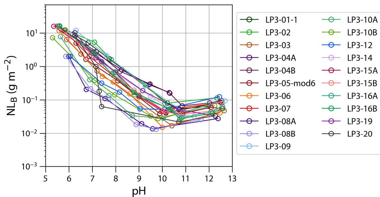
Figure B-10. EPA 1313 normalized elemental release of B for LP3 glasses
