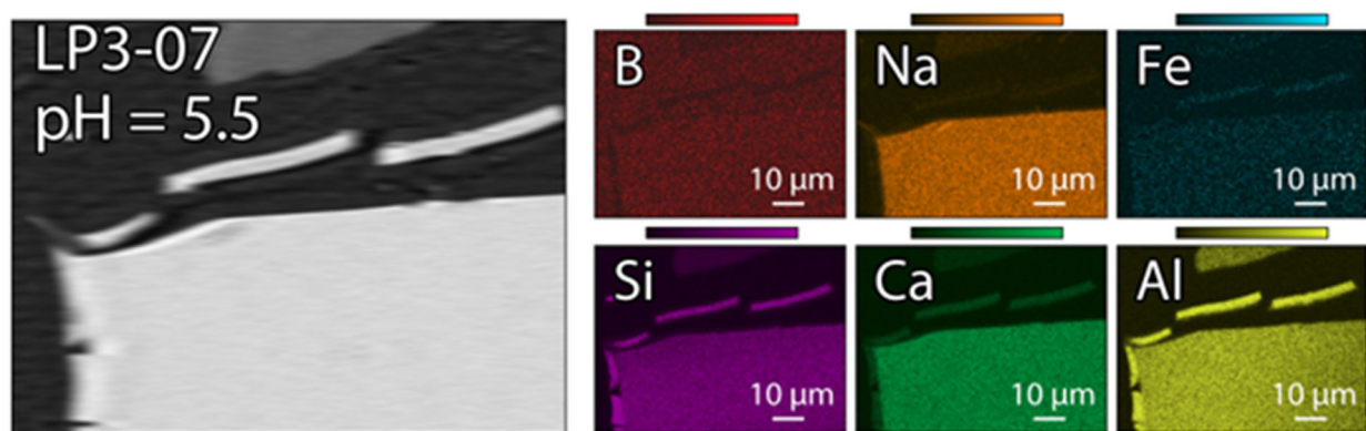
Figure C-5. LP3-07 after 2 Day EPA 1313 with pH = 5.5, map #1
