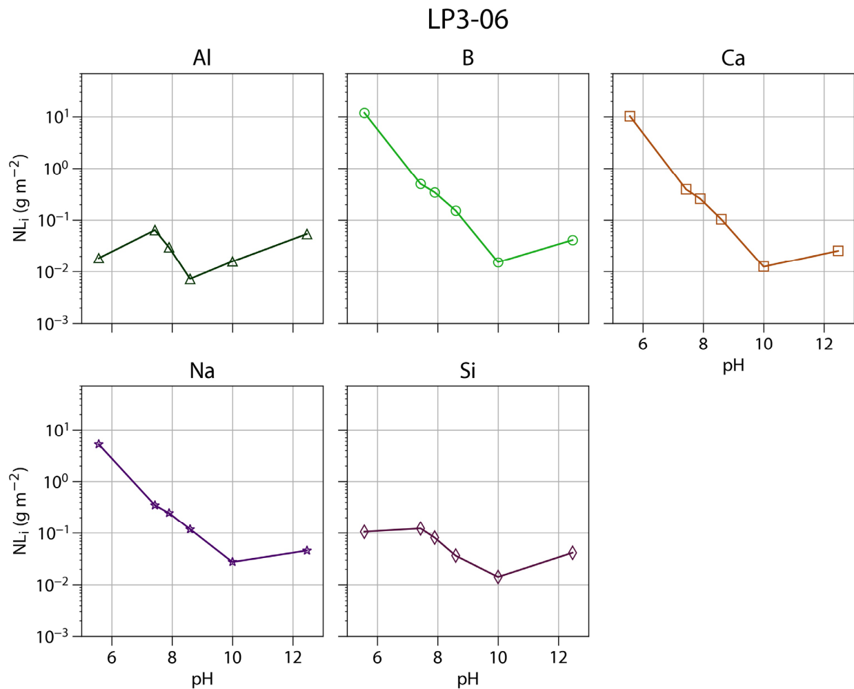
Figure B-20. EPA 1313 normalized elemental releases of Al, B, Ca, Na, and Si for LP3-06
