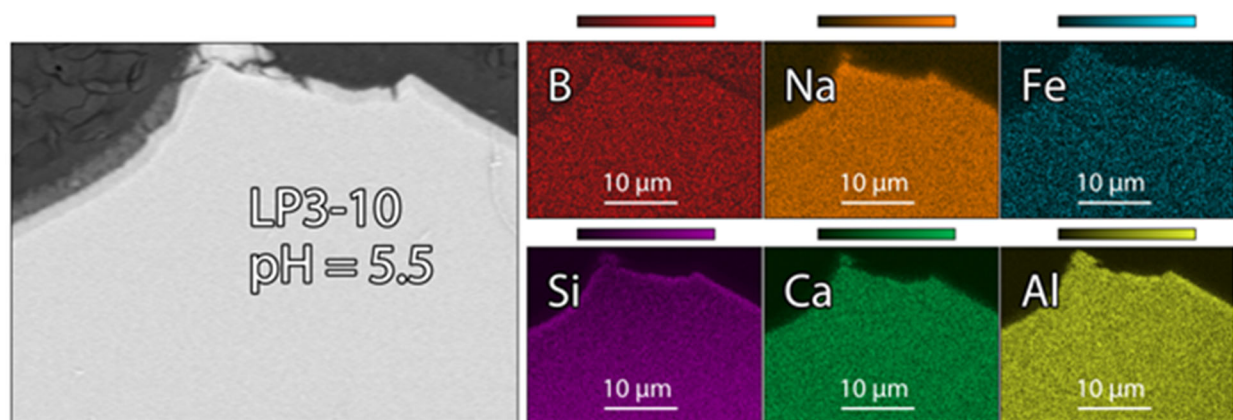
Figure C-13. LP3-10 glass after 2 Day EPA 1313 with pH = 5.5, map #1
