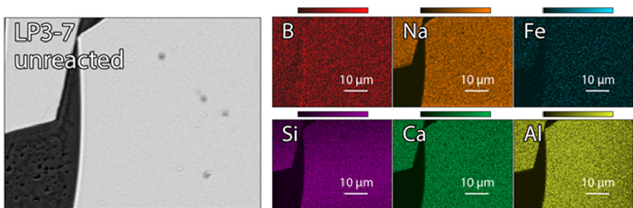
Figure C-4. LP3-07 unreacted glass
