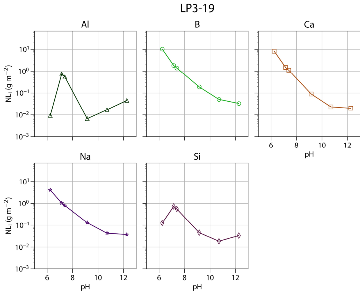
Figure B-33. EPA 1313 normalized elemental releases of Al, B, Ca, Na, and Si for LP3-19
