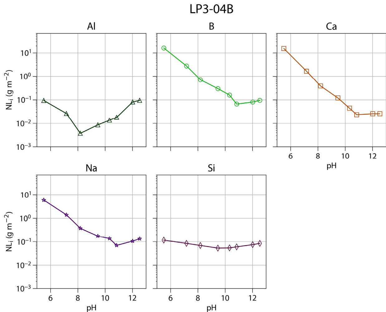
Figure B-18. EPA 1313 normalized elemental releases of Al, B, Ca, Na, and Si for LP3-04 (trial #2)
