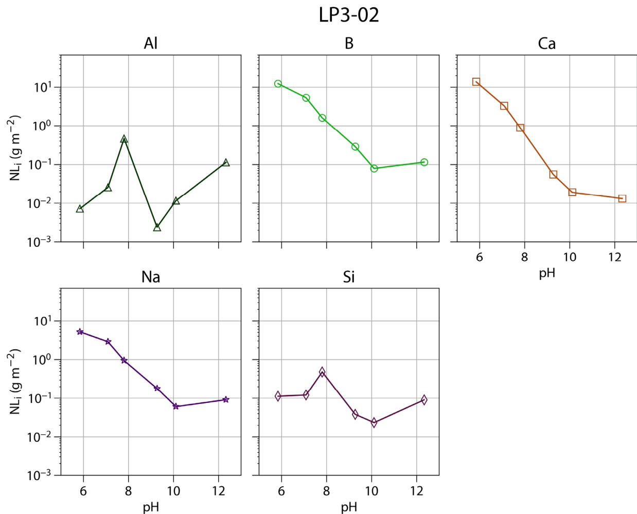
Figure B-15. EPA 1313 normalized elemental releases of Al, B, Ca, Na, and Si for LP3-02
