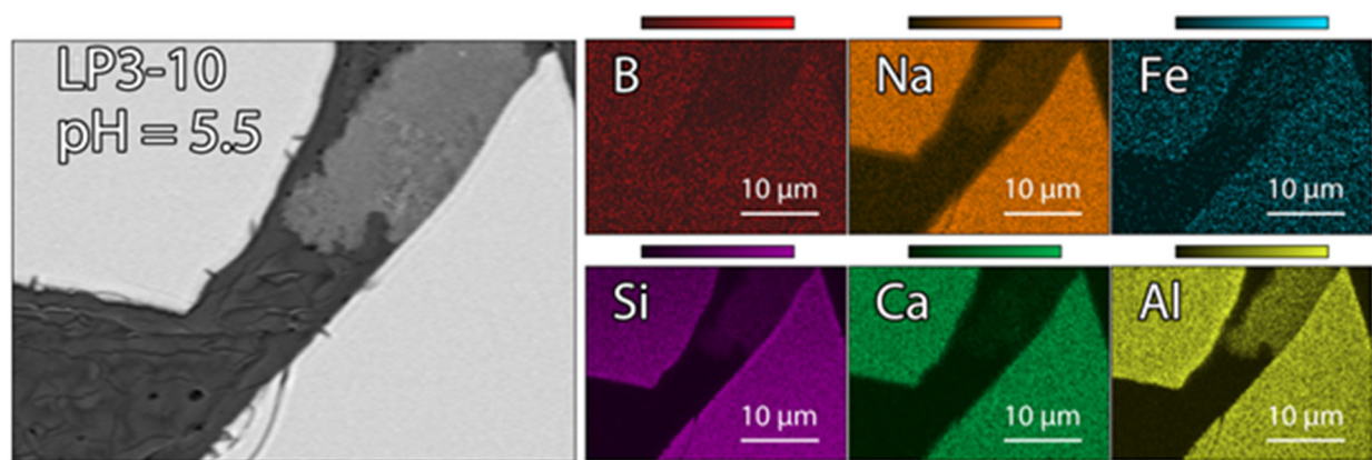
Figure C-14. LP3-10 glass after 2 Day EPA 1313 with pH = 5.5, map #2
