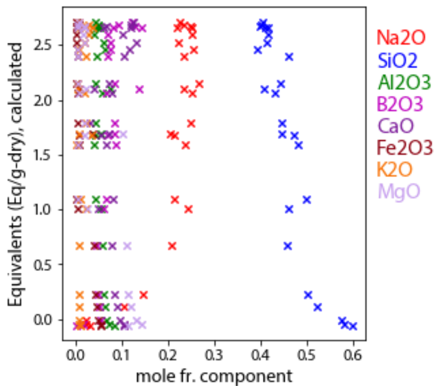
Figure A-3. Calculated acid equivalents as a function of mole fraction component for 8 oxides fit using ANN model #1
