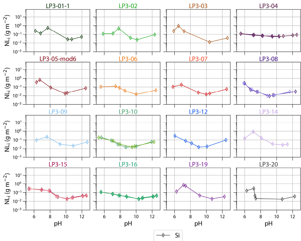
Figure B-8. EPA 1313 NL_{Si} for the 16 LP3 glasses
