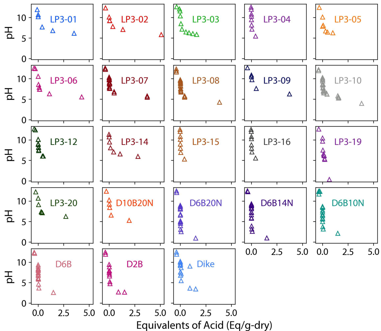
Figure A-1. Final eluate pH versus acid equivalents for the glasses tested in this study. Experimental details are provided in Section 2.6.
