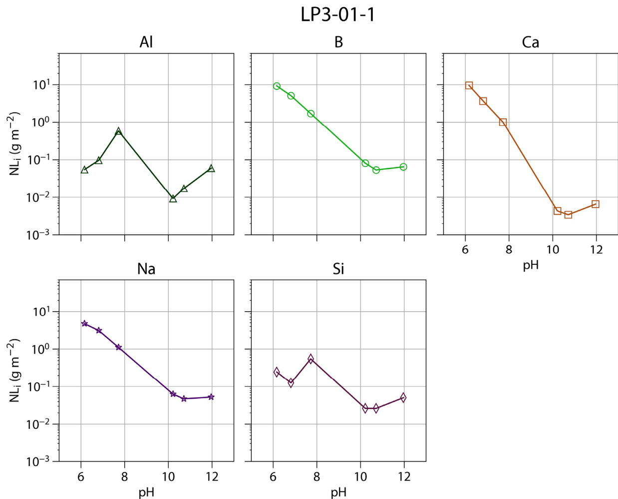
Figure B-14. EPA 1313 normalized elemental releases of Al, B, Ca, Na, and Si for LP3-01-1
