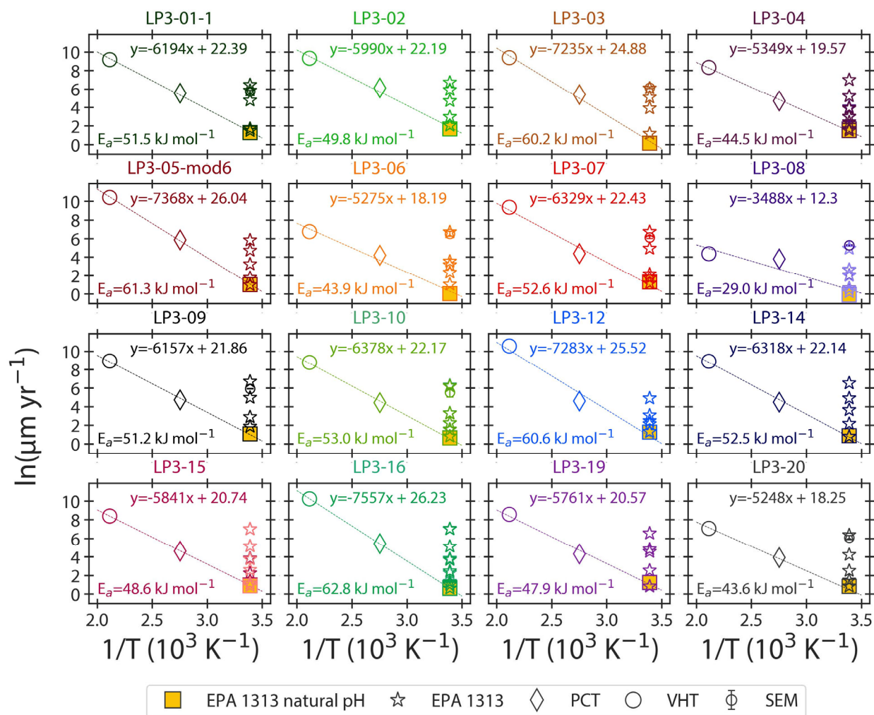
Figure 3-6. Comparison of alteration rates from PCT, VHT, and EPA 1313 of LP3 glasses (PCT and VHT were not performed on join glasses). In this figure the ‘natural pH’ refers to the alteration with no acid or base added (acid equivalents equal zero). A line was fit through the VHT data, PCT data, and natural pH point in the EPA 1313.
