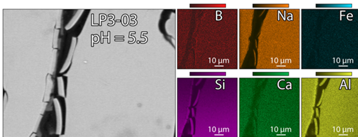
Figure C-2. LP3-03 after 2 Day EPA 1313 with pH = 5.5
