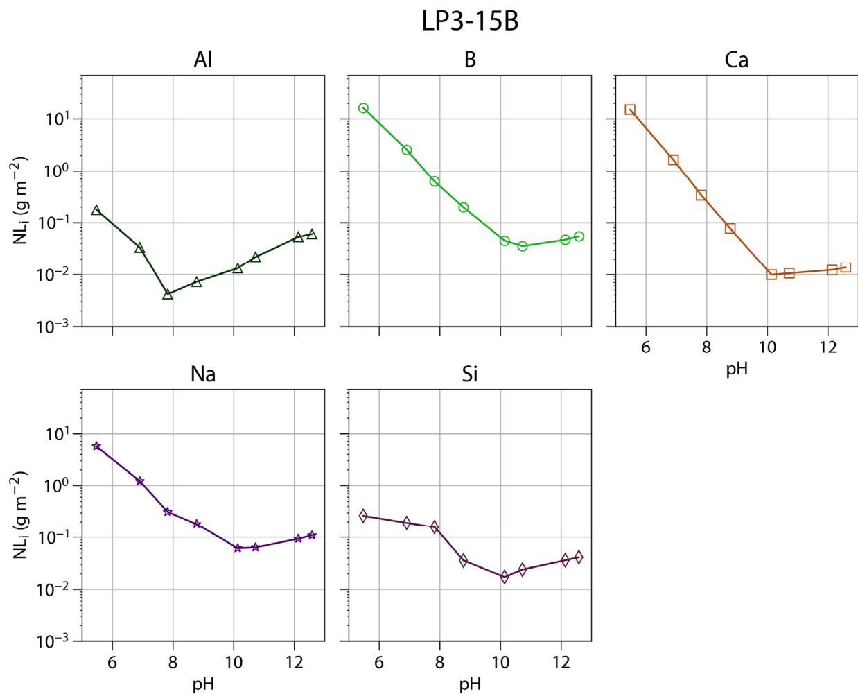
Figure B-30. EPA 1313 normalized elemental releases of Al, B, Ca, Na, and Si for LP3-15 (trial #2)
