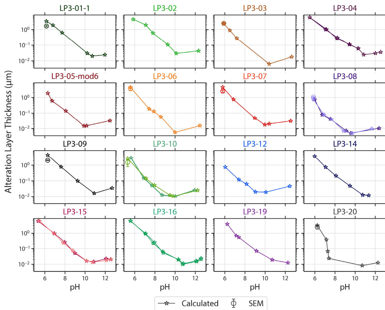
Figure B-1. Calculated alteration layer thickness, E_{th} , calculated using normalized release of B for 16 LP3 glasses
