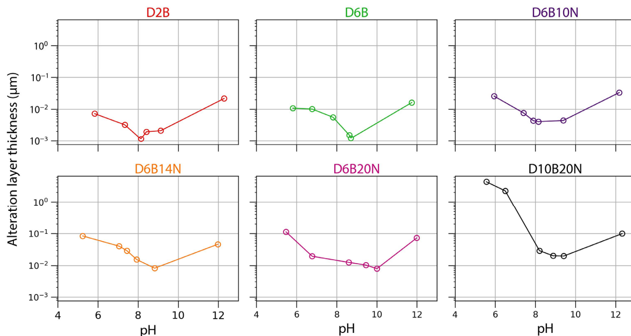
Figure B-2. Calculated alteration layer thickness ( E_{th} ) calculated using normalized release of B for 6 join glasses (note Dike glass is excluded as it did not contain boron)
