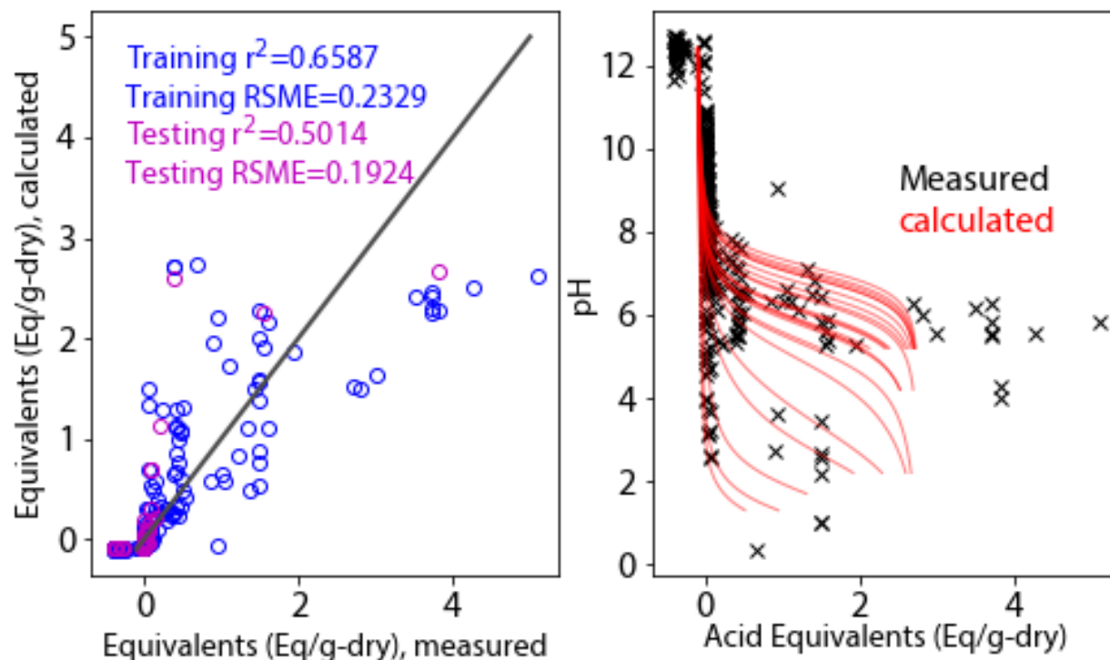
Figure A-2. (left) Comparison of measured acid equivalents to compositional ANN model #1 and (right) titration curves for LP3 glasses and join glasses. The solid line on the left is the unity line. On the left, the training dataset is shown in blue and the testing dataset is shown in magenta.
