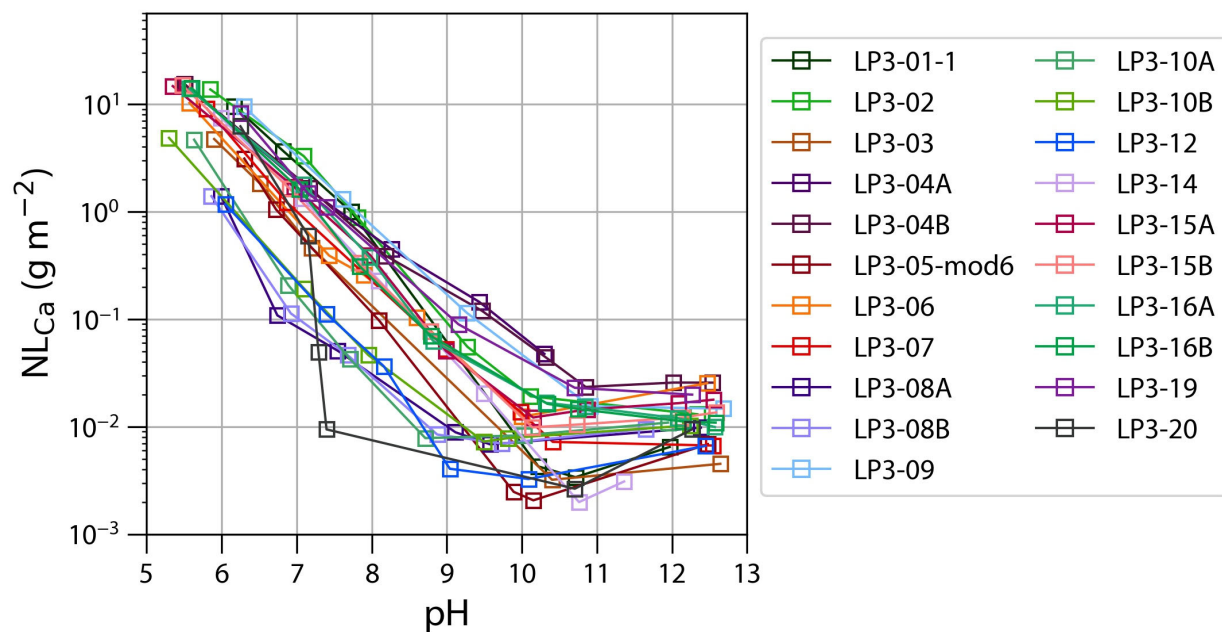
Figure B-11. EPA 1313 normalized elemental release of Ca for LP3 glasses
