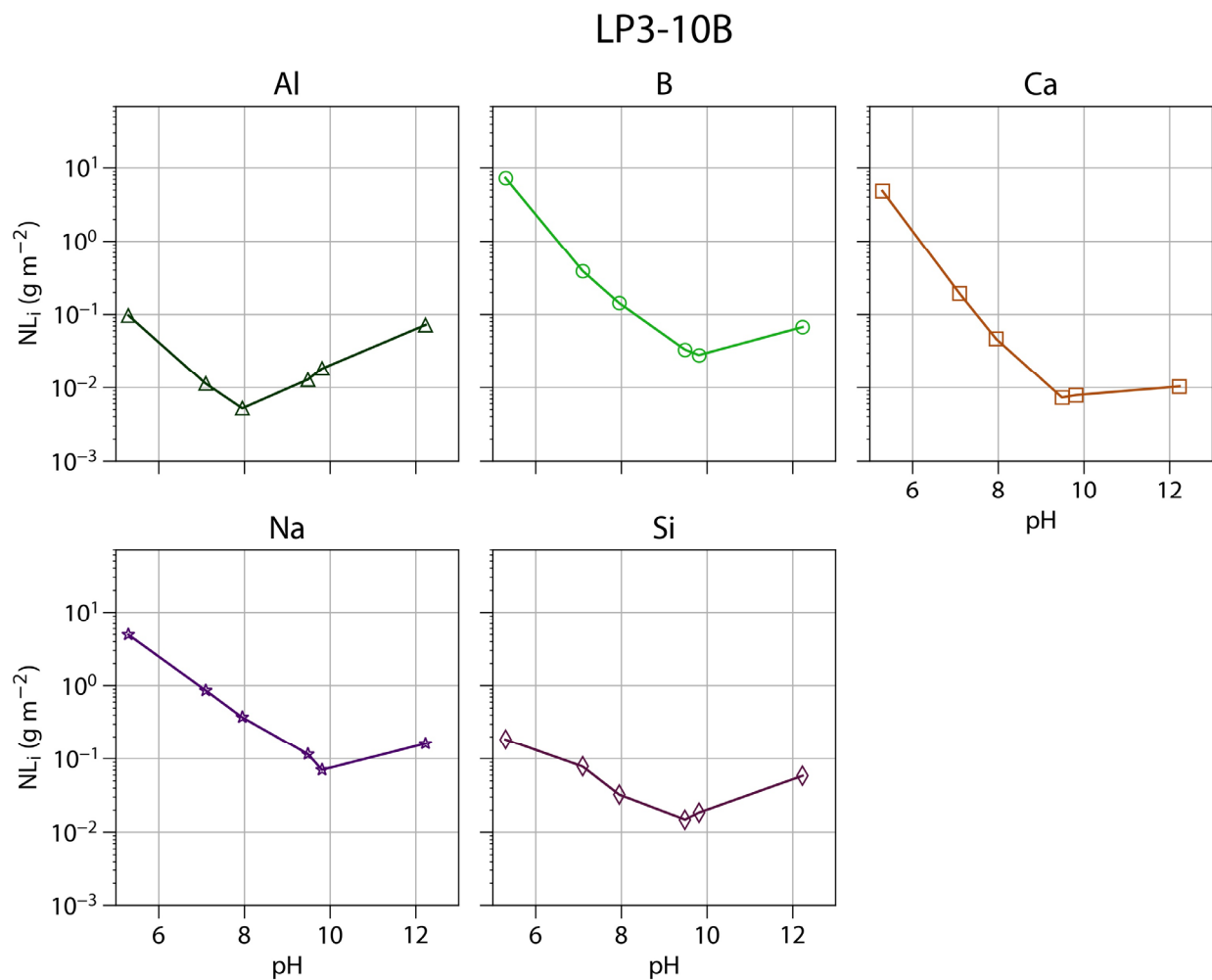
Figure B-26. EPA 1313 normalized elemental releases of Al, B, Ca, Na, and Si for LP3-10 (trial #2)
