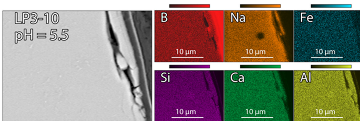
Figure C-15. LP3-10 glass after 2 Day EPA 1313 with pH = 5.5, map #3
