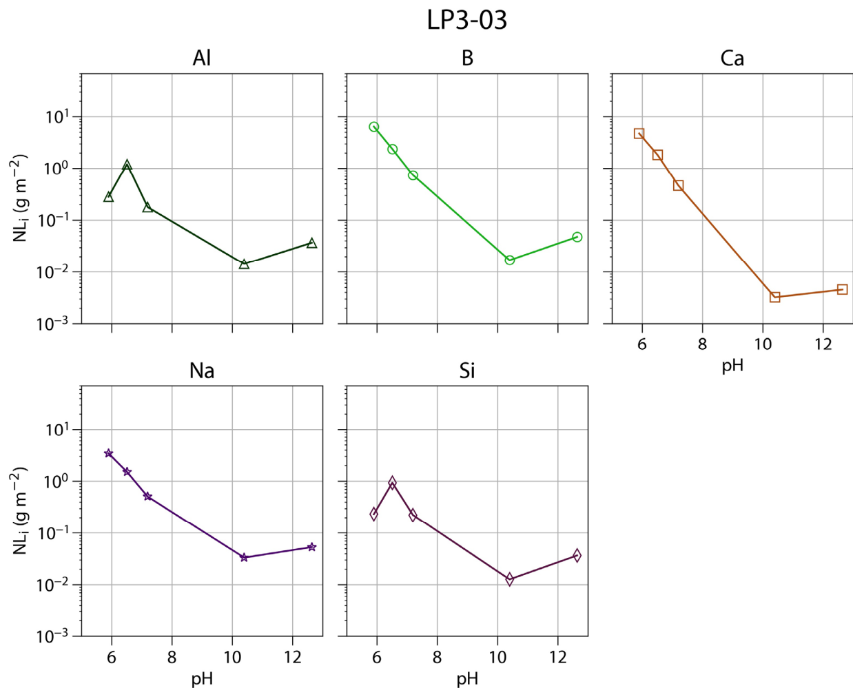
Figure B-16. EPA 1313 normalized elemental releases of Al, B, Ca, Na, and Si for LP3-03
