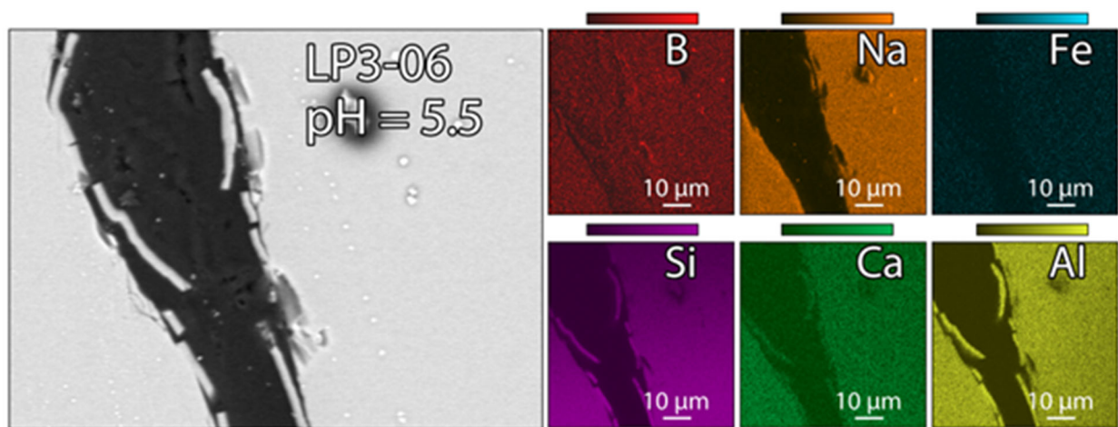
Figure C-3. LP3-06 after 2 Day EPA 1313 with pH = 5.5
