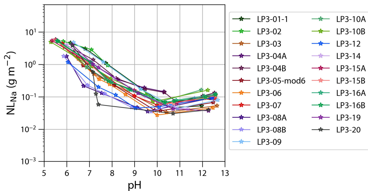
Figure B-12. EPA 1313 normalized elemental release of Na for LP3 glasses
