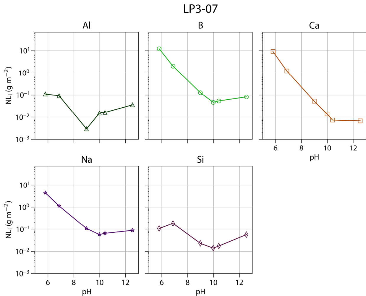
Figure B-21. EPA 1313 normalized elemental releases of Al, B, Ca, Na, and Si for LP3-07
