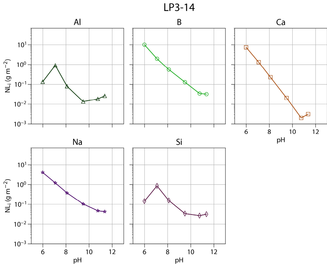
Figure B-28. EPA 1313 normalized elemental releases of Al, B, Ca, Na, and Si for LP3-14
