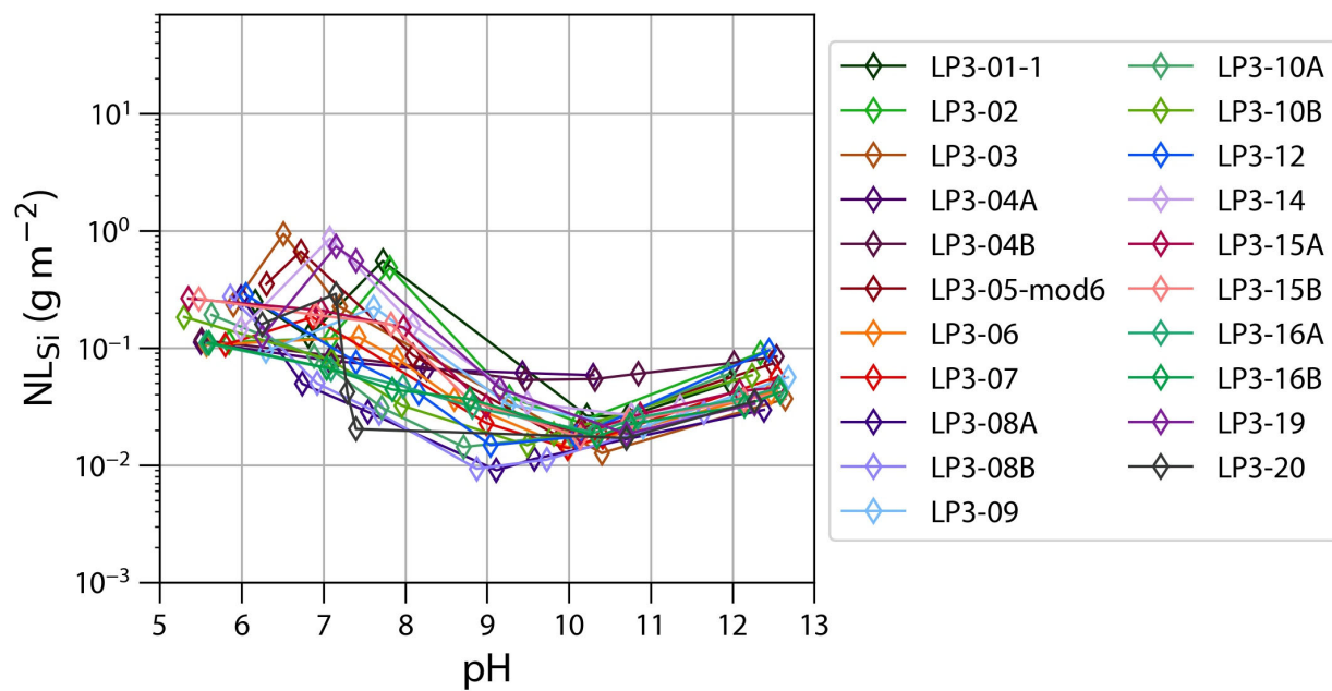
Figure B-13. EPA 1313 normalized elemental release of Si for LP3 glasses
