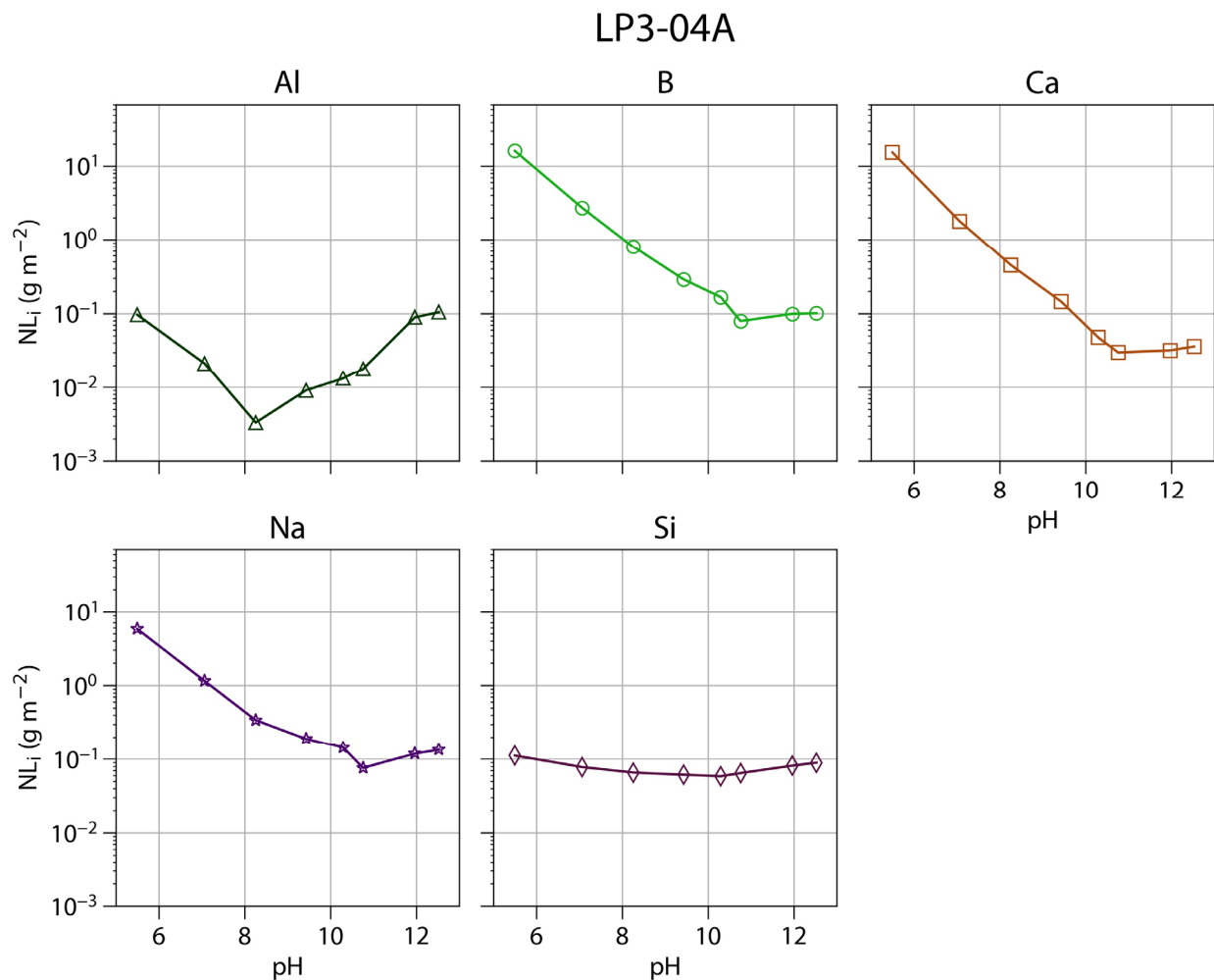
Figure B-17. EPA 1313 normalized elemental releases of Al, B, Ca, Na, and Si for LP3-04 (trial #1)
