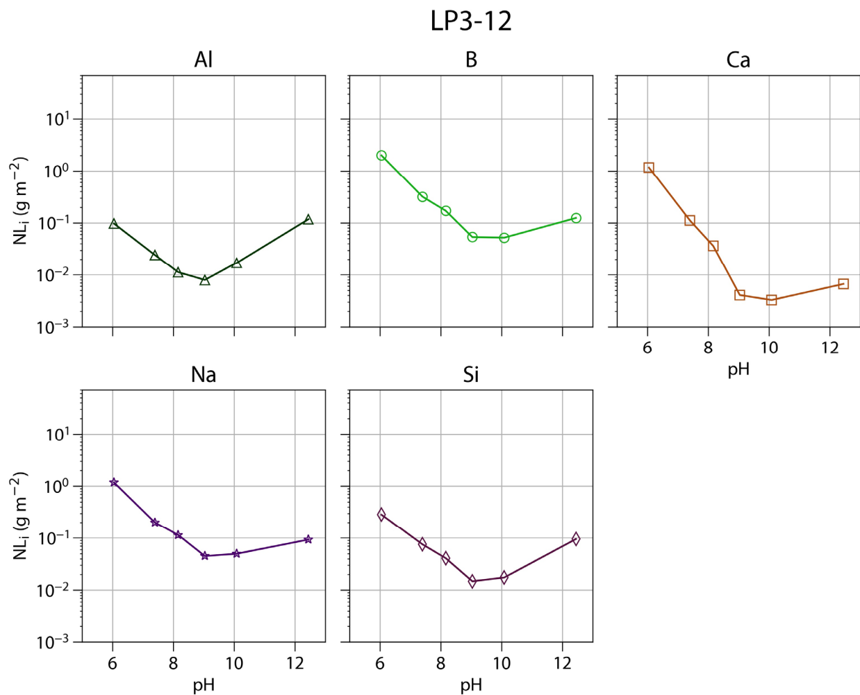
Figure B-27. EPA 1313 normalized elemental releases of Al, B, Ca, Na, and Si for LP3-12
