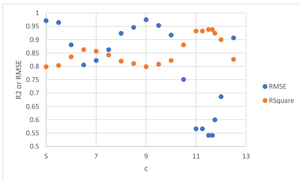
Figure D-1. Comparison of fitting parameter as a function of cutoff, c .
