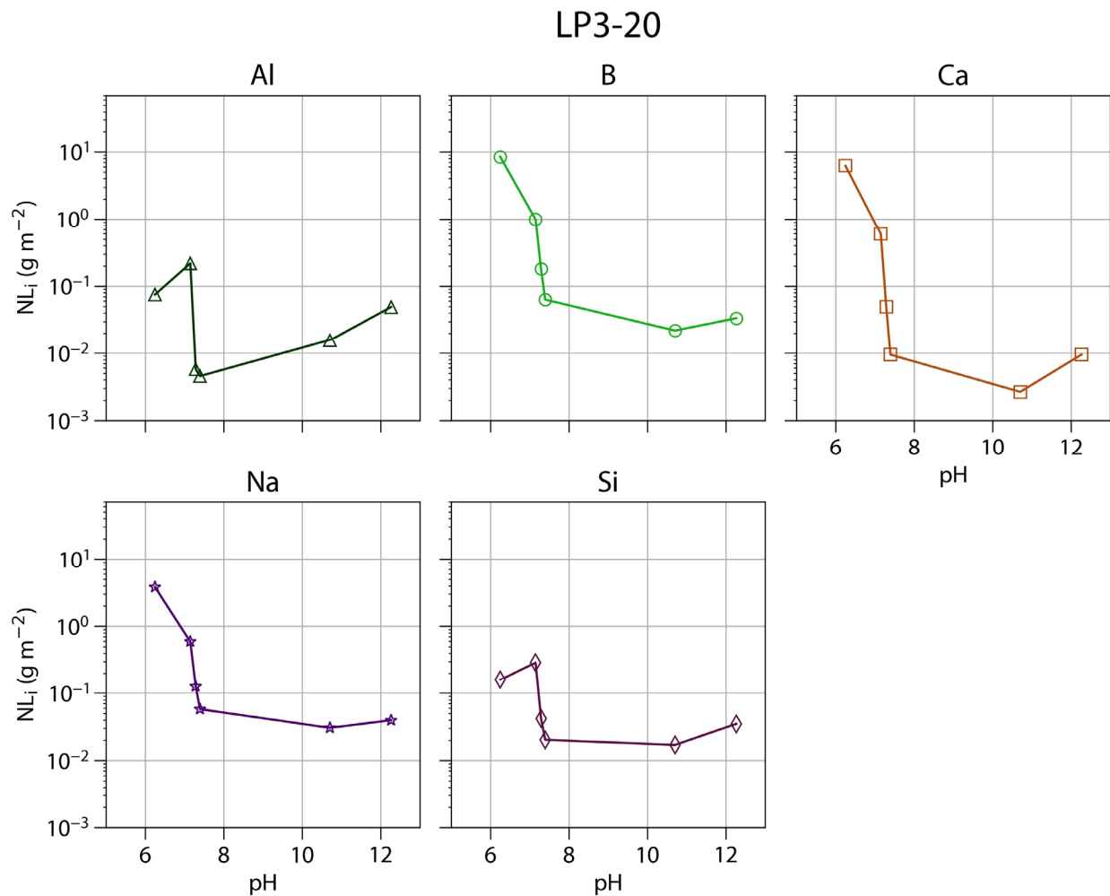
Figure B-34. EPA 1313 normalized elemental releases of Al, B, Ca, Na, and Si for LP3-20
