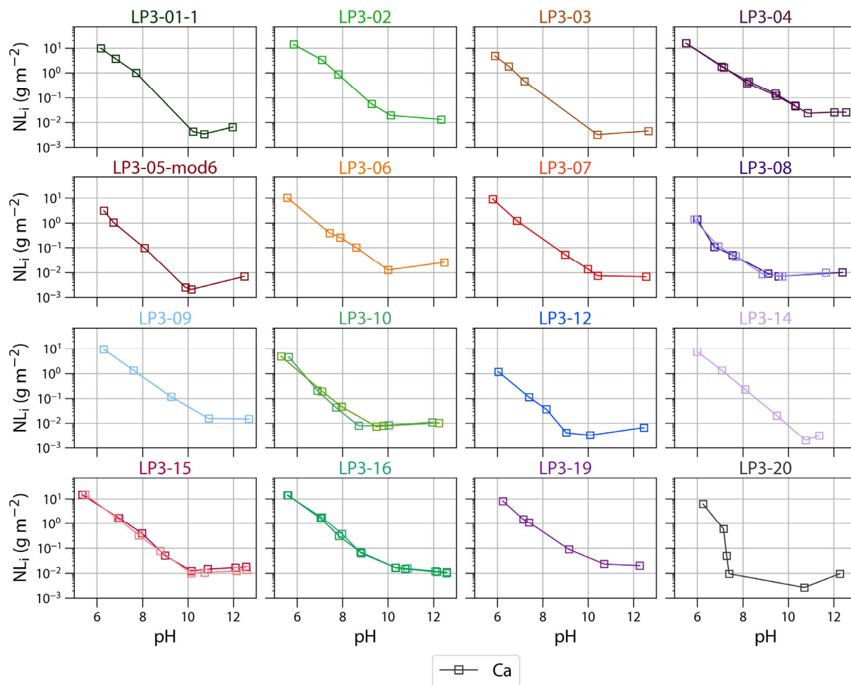
Figure B-6. EPA 1313 NL_{Ca} for the 16 LP3 glasses
