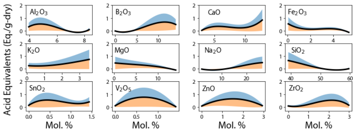
Figure 3-2. Trace plots demonstrating component effects on predicted acid equivalents. The 99% confidence interval (which combines the statistical variation of the standard deviation and the number of samples per data point, n=22 ) is shown as shaded areas above and below the lines.
