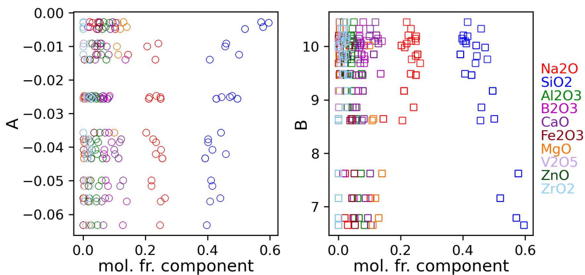
Figure A-5. Variation of model coefficients as a function of composition for ANN model #2
