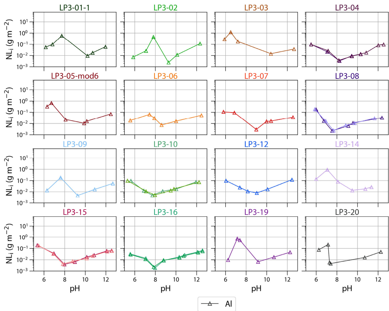
Figure B-4. EPA 1313 NL_{Al} for the 16 LP3 glasses
