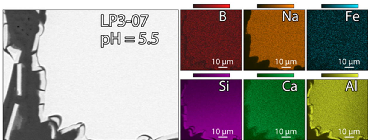
Figure C-6. LP3-07 after 2 Day EPA 1313 with pH = 5.5, map #2
