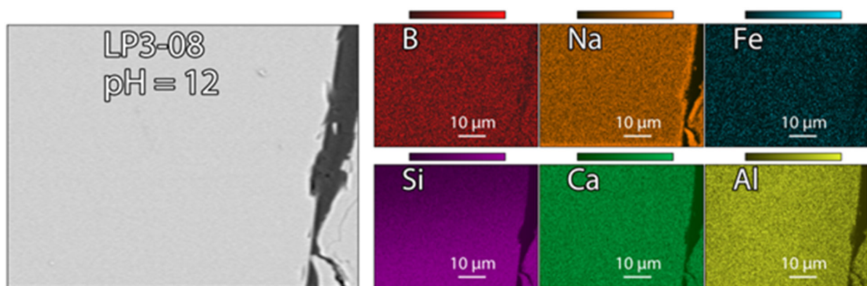
Figure C-10. LP3-08 glass after 2 Day EPA 1313 with pH = 12
