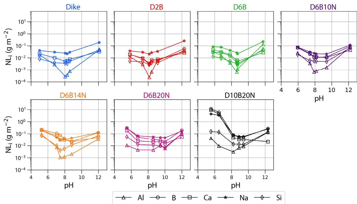
Figure 3-4. EPA 1313 normalized elemental releases for join glasses
