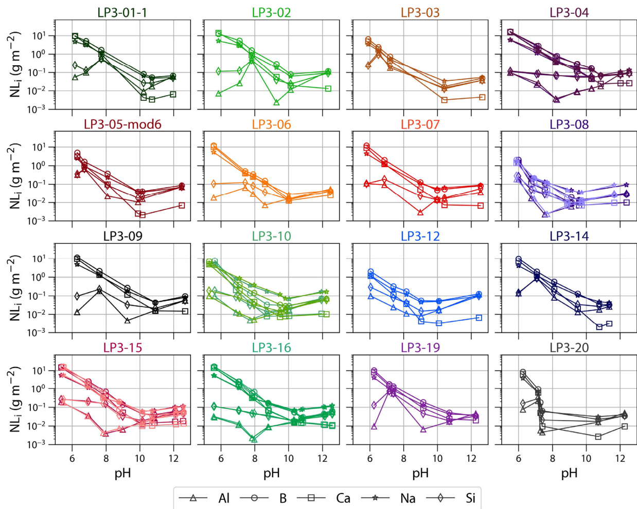
Figure 3-3. EPA 1313 normalized elemental releases for 16 LP3 glasses
