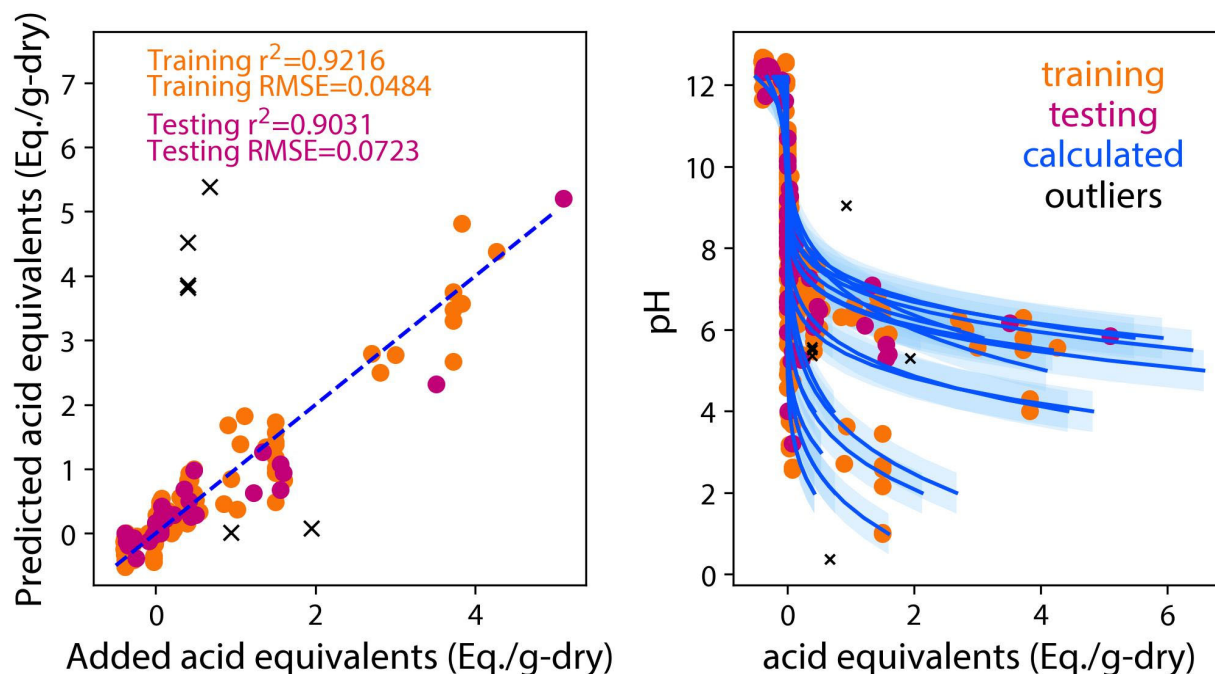
Figure 3-1. (left) comparison of measured acid equivalents to predicted acid equivalents from the mixed linear compositional model and (right) titration curves for LP3 and join glasses and join glasses, the shaded region shows the fit curve with a \pm 0.5 pH unit offset.
