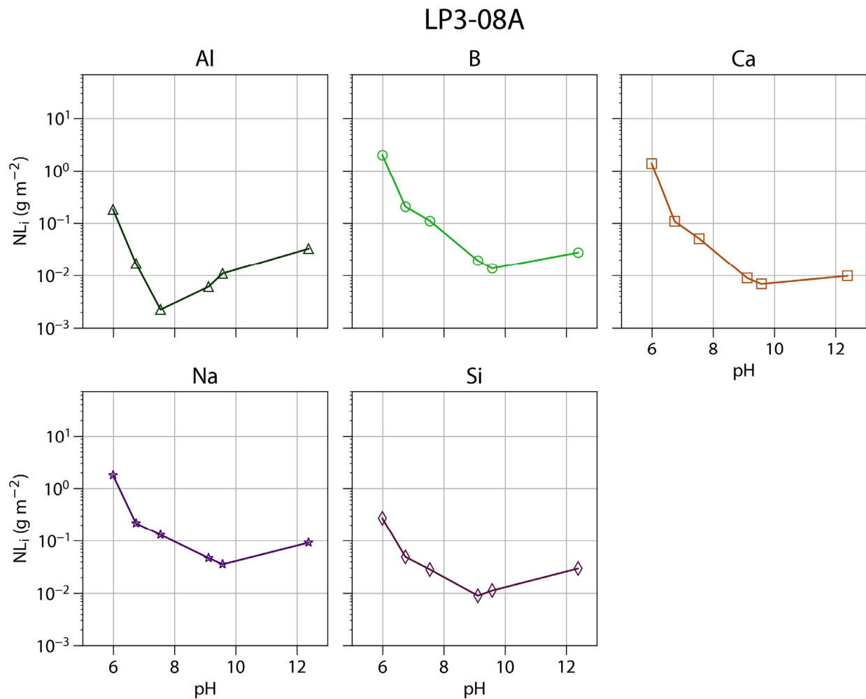
Figure B-22. EPA 1313 normalized elemental releases of Al, B, Ca, Na, and Si for LP3-08 (trial#1)
