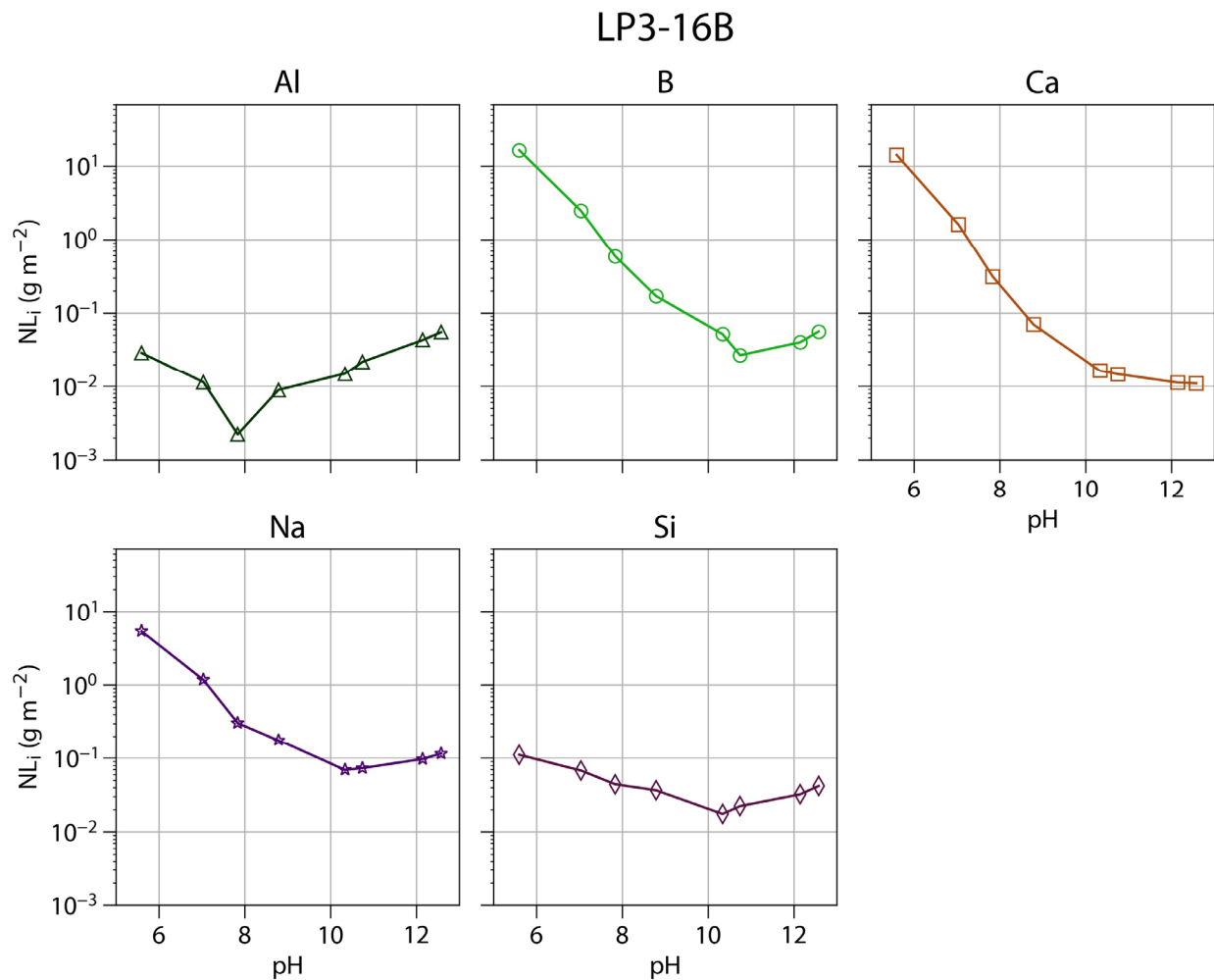
Figure B-32. EPA 1313 normalized elemental releases of Al, B, Ca, Na, and Si for LP3-16 (trial #2)
