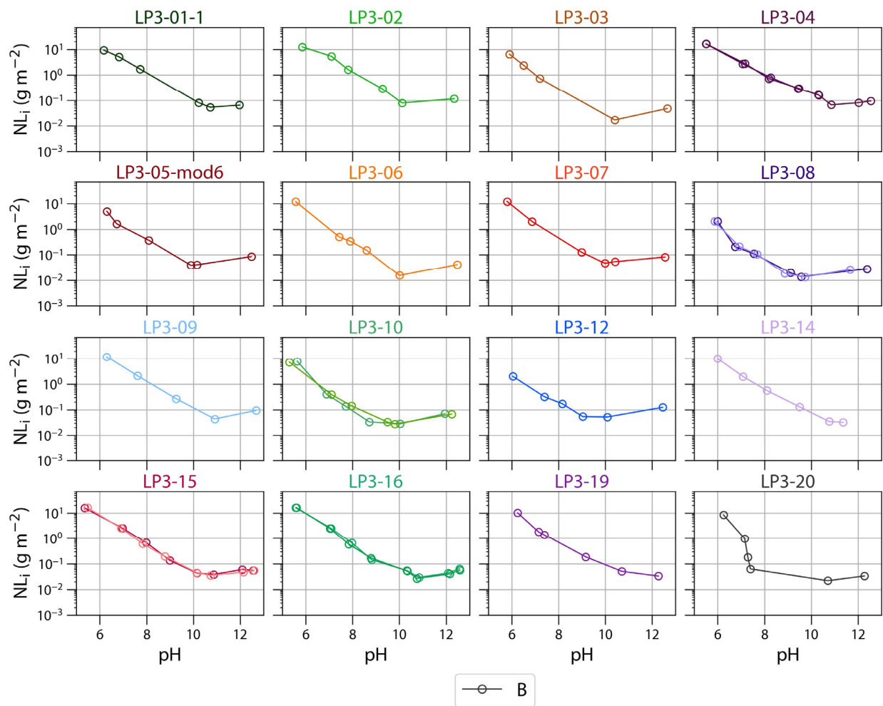
Figure B-5. EPA 1313 NL_B for the 16 LP3 glasses
