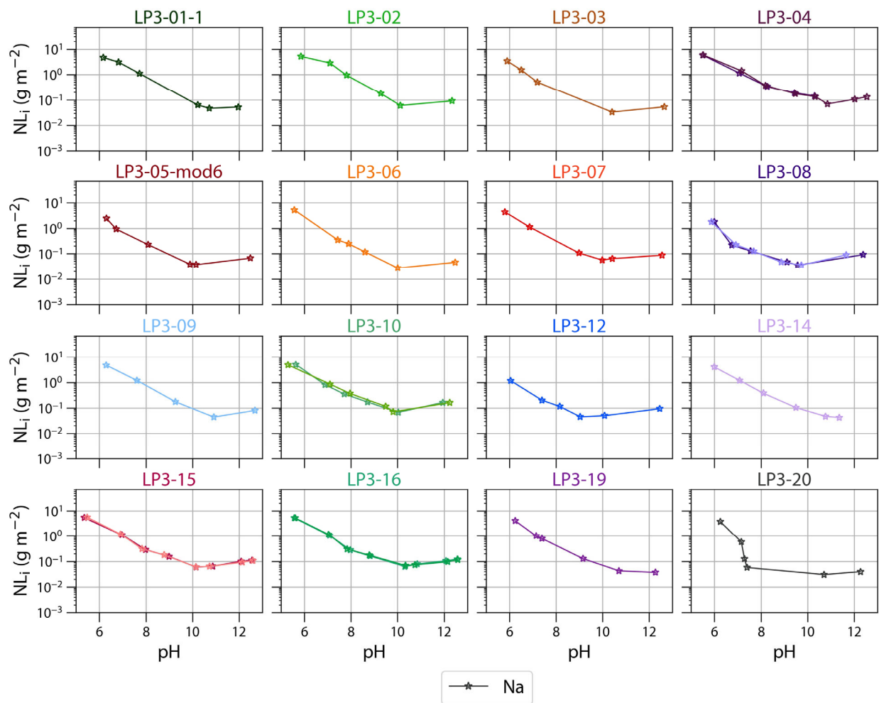
Figure B-7. EPA 1313 NL_{Na} for the 16 LP3 glasses
