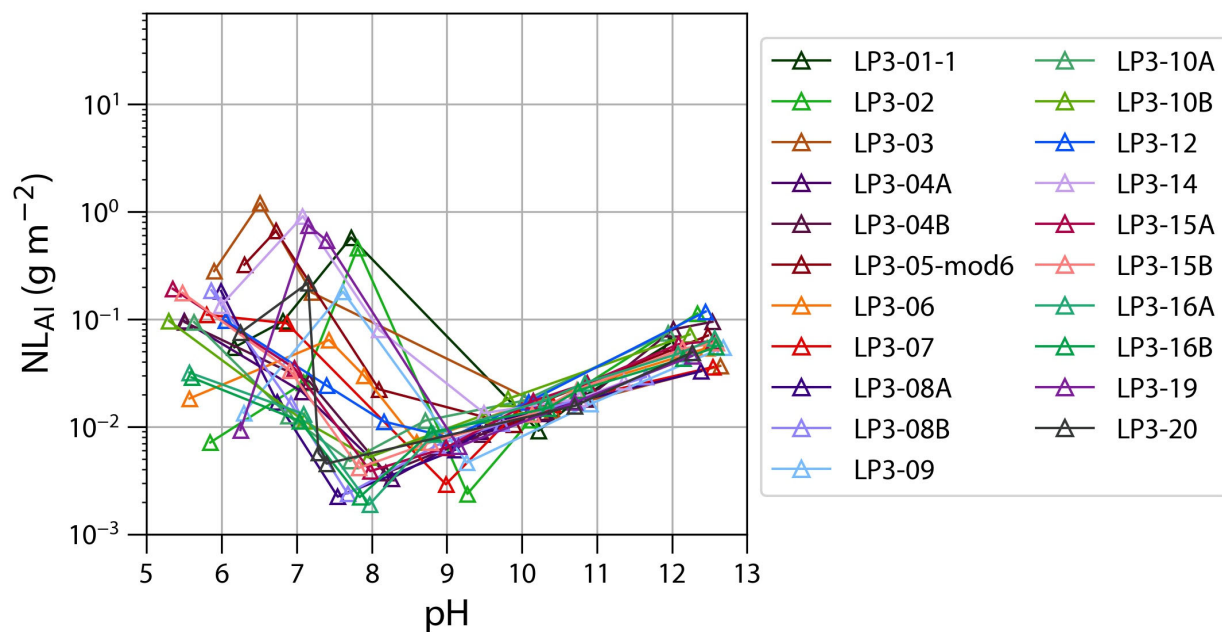
Figure B-9. EPA 1313 normalized elemental release of Al for LP3 glasses
