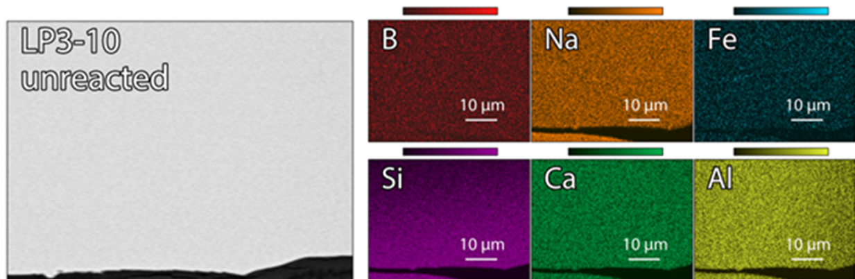
Figure C-12. LP3-10 unreacted glass
