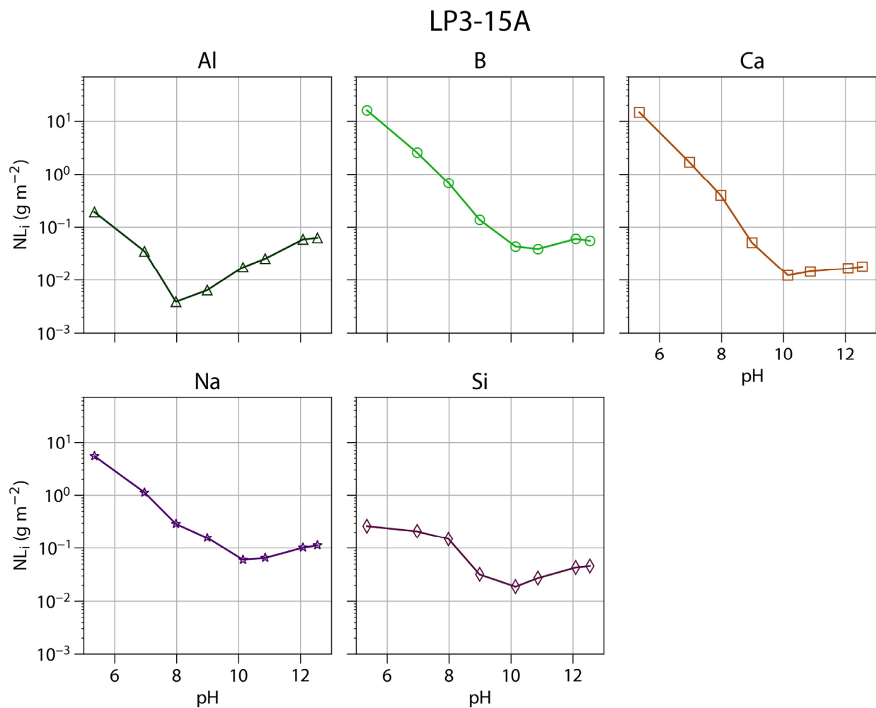
Figure B-29. EPA 1313 normalized elemental releases of Al, B, Ca, Na, and Si for LP3-15 (trial #1)
