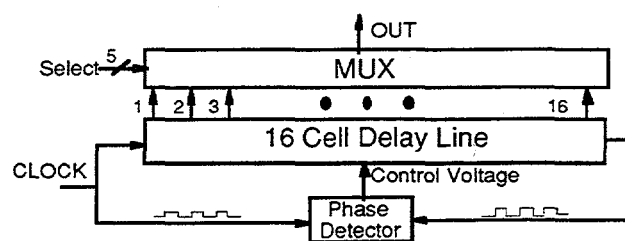
Fig. 1 Block diagram of the DLL chip
