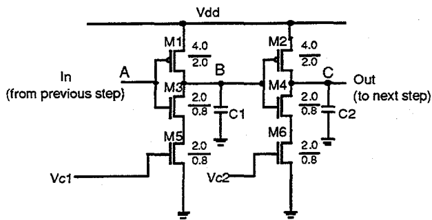
Fig. 2 Delay element unit cell.
