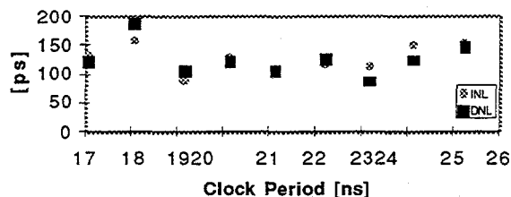
Fig. 7 Plot of TDC Integral and Differential Non-Linearity.
