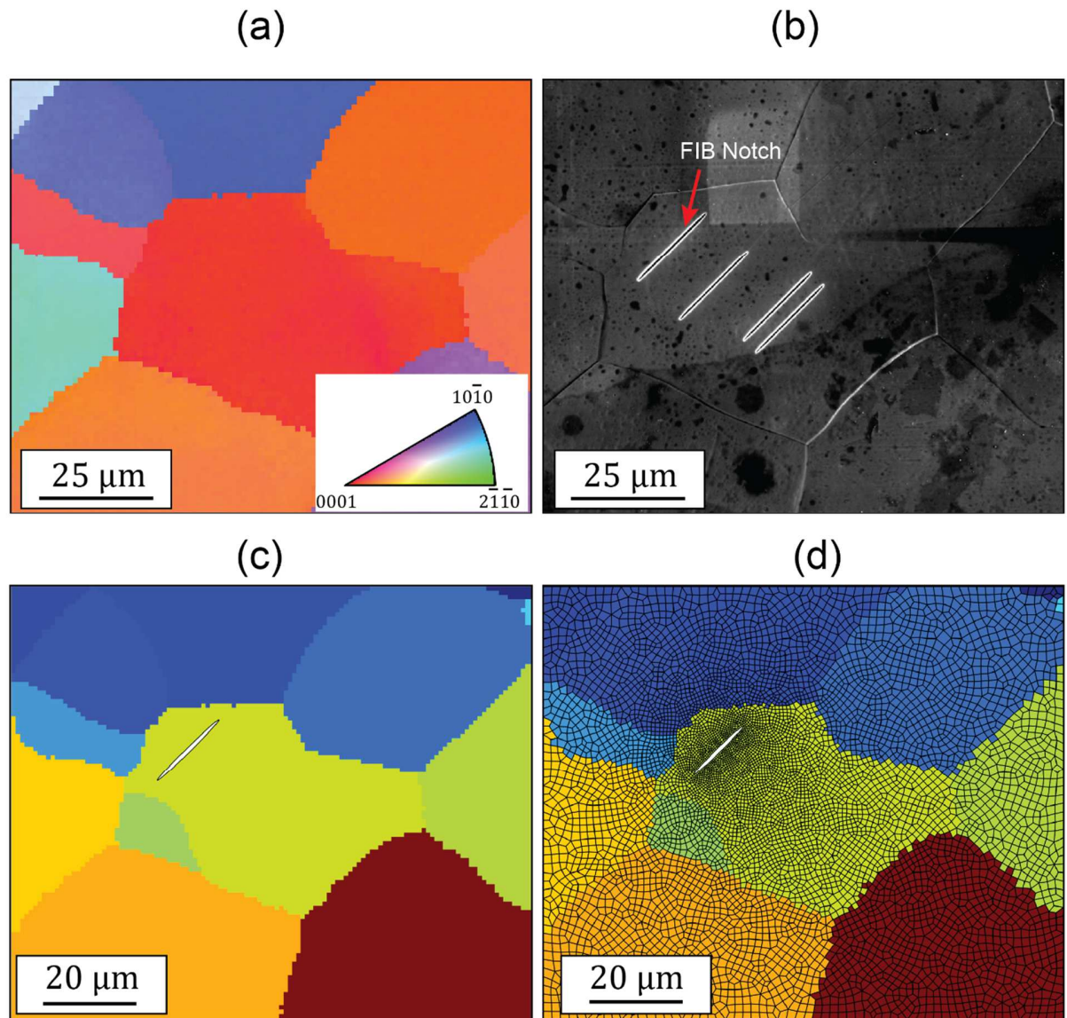
Figure 6: (a) EBSD section for the region around grain boundary, (b) Grain with notch generated using FIB, (c) Grain identifiers for microstructure section, and (d) Microstructure section meshed using Gmsh with 4-node quadrilateral elements with grain identifiers assigned.
