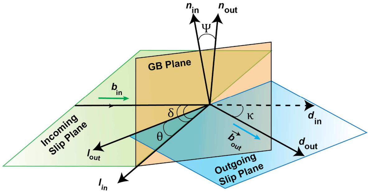
Figure 10. A schematic representative for slip transmission through a GB. \vec{b}_{in} : Burgers vector of the incoming slip system, \vec{b}_{out} : Burgers vector of the outgoing slip system, \vec{n}_{in} : Slip plane normal of the incoming slip system, \vec{n}_{out} : Slip plane normal of the outgoing slip system, \vec{l}_{in} :
