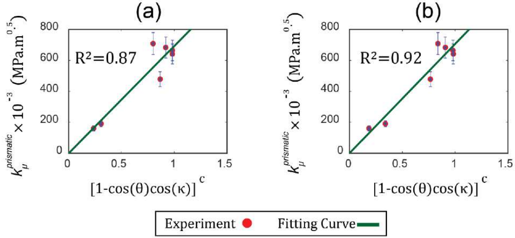
Figure 17: k_{\mu}^{prismatic} values against (1 - \cos(\theta)\cos(\kappa))^c based on (a) BC#1 and (b) BC#2.
