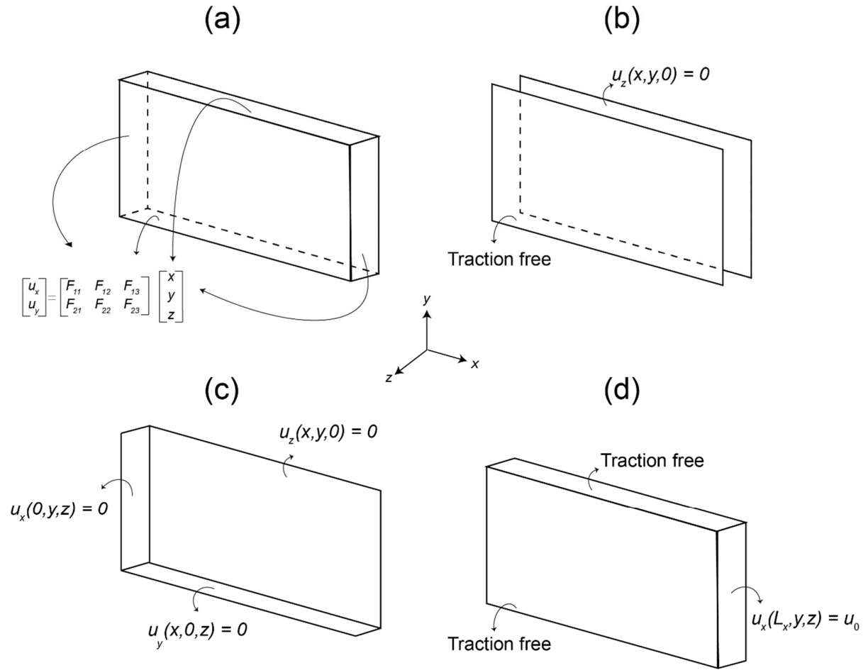
Figure 7: Boundary condition 1 (BC#1): (a) x and y displacement components set on lateral surfaces, (b) x - y plane constrained along z -direction, Boundary condition 2 (BC#2): (c), (d) denote symmetry boundary conditions similar to the boundary condition enforced in the calibration section for scenario 1.
