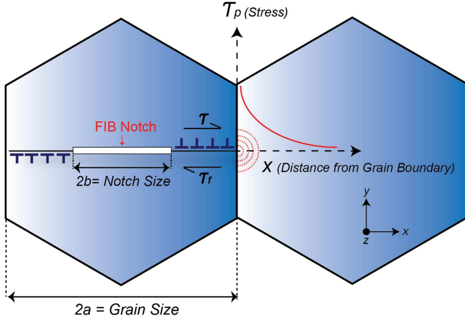
Figure 4: Notch and slip band idealized as a continuous distribution of parallel edge dislocations.
