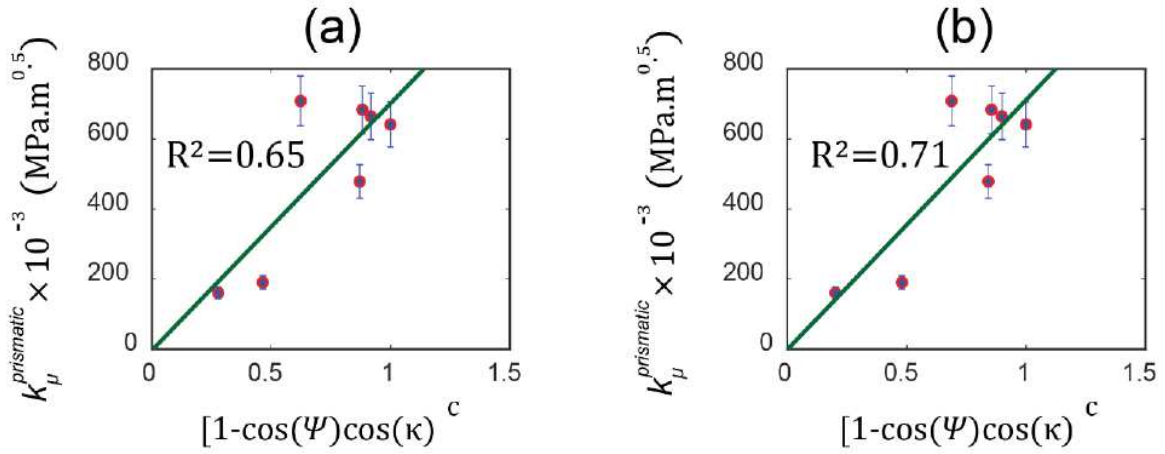
Figure 18: The prismatic slip system micro-Hall-Petch coefficients ( k_{\mu}^{prismatic} ) for the seven-cases are plotted against the factor (1 - \cos(\psi)\cos(\kappa))^c based on (a) BC#1 and (b) BC#2.
