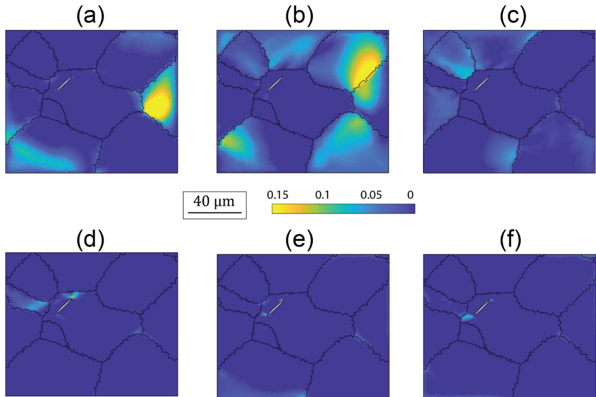
Figure 12. Boundary Condition 1: (a) Accumulated slip for Basal 1, (b) Accumulated slip for Basal 2, (c) Accumulated slip for Basal 3, (d) Accumulated slip for Prismatic 1, (e) Accumulated slip for Prismatic 2, and (f) Accumulated slip for Prismatic 3. It can be observed that prismatic slip is particularly dominant in the neighborhood of the notches on either side.
