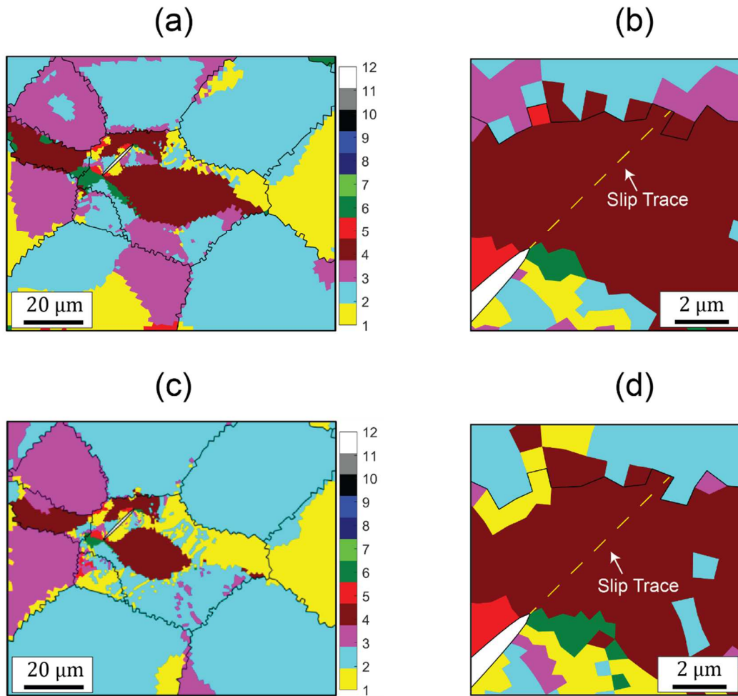
Figure 14: Visualization of most active slip system for all elements of the microstructure, corresponding to GB ID 3, included in Table 7. The numbers in the color bar correspond to the slip system IDs in Table 6. The most active slip system in every element is recognized as the one with the highest accumulated slip within the element. The basal and prismatic \langle a \rangle slip systems dominate in slip activity for both boundary conditions considered. (a) BC#1 – Most active slip system map (b) Close-up with prismatic slip trace superposed, (c) BC#2 – Most active slip system map (d) Close-up with prismatic slip trace superposed. For both BC#1 and BC#2, the incoming slip system is (10\bar{1}0)[1\bar{2}10] and the potential outgoing slip system is (0001)[\bar{2}110] .
