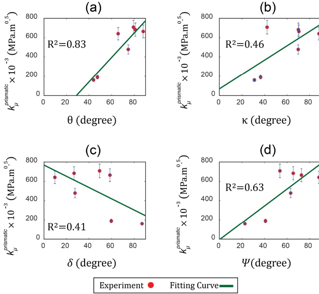
Figure 15: The prismatic micro-Hall-Petch coefficient values relevant angles ( \theta , \kappa , \psi , \delta ) calculated based on BC#1. (a) k_{\mu}^{prismatic} vs the angle between the two slip plane intersections with the GB ( \theta ). (b) k_{\mu}^{prismatic} vs the Angle between incoming and outgoing slip directions ( \kappa ). (c) k_{\mu}^{prismatic} vs the angle between slip plane normal ( \psi ). (d) k_{\mu}^{prismatic} vs the angle between the incoming slip direction and the incoming slip plane trace on the GB plane ( \delta ).
