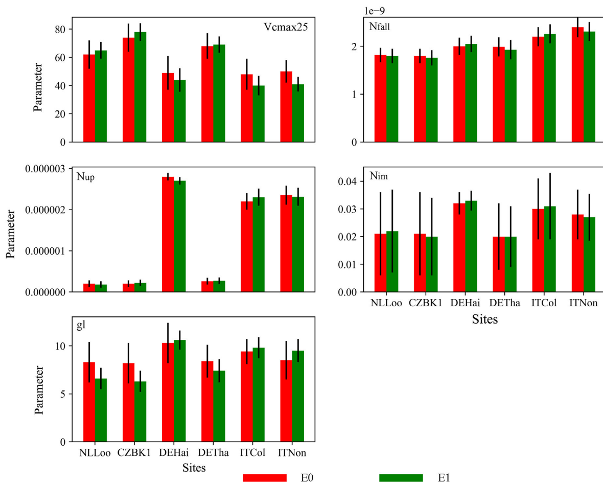
Fig. 1. Comparison of data-conditioned parameters from the two model-data fusion experiments (E0 and E1) at six forest sites. E0 used GPP and NEE observations as constraint, while E1 used GPP, NEE and \delta^{13}\text{C}_f observations as constraint. More details on the parameter description in the figure refer to Table 2.
