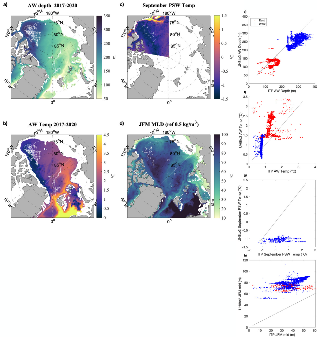
Fig. 9. Comparison of four-year averaged UH8to2 and ITP-observed quantities. (a) UH8to2 Atlantic Water depth (m) from 2017–2020, (b) UH8to2 maximum Atlantic Water temperature ( ^{\circ}\text{C} ) from 2017–2020, (c) UH8to2 Pacific Summer Water temperature ( ^{\circ}\text{C} ) in September of 2017–2020, and (d) UH8to2 winter (January, February, and March) mixed layer depths (m) from 2017–2020. (e) through (h) show comparisons of ITP-observed values of each quantity with the UH8to2 value in the 0.25^{\circ} interpolated grid, where eastern deployments are in red and western in blue. ITP transects are shown as white lines in (a) through (d).
