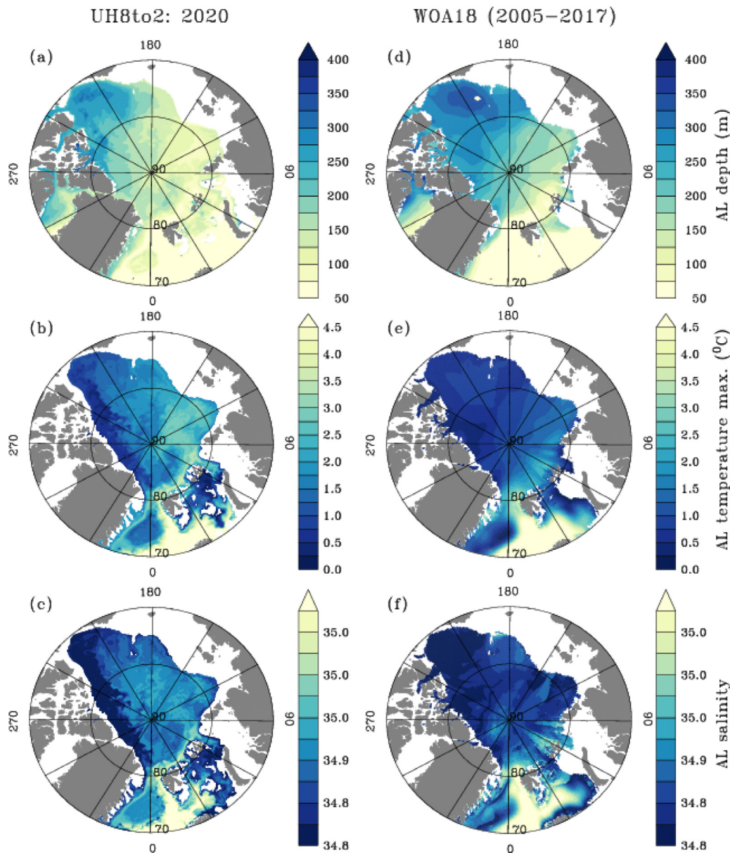
Fig. 11. Atlantic layer characteristics in the UH8to2 (year 2020) and WOA18 (data from 2005–2017). Top: depth (m), defined as the upper-most depth in the water column below 50 m of the 0 °C isotherm for (a) UH8to2 (2020) and (d) WOA18. Middle: maximum temperature (°C) in the Atlantic layer located between the subsurface 0 °C isotherms where salinities are greater than 34.8 for (b) UH8to2 and (e) WOA18. Bottom: salinity at the depth of the temperature maximum from (c) UH8to2 and (f) WOA18.
