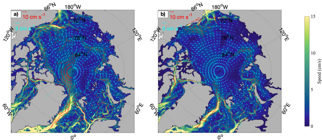
Fig. 4. 2017 Arctic surface velocities ( \text{cm s}^{-1} ) from (a) the UH8to2 model and (b) the ASTE estimate (Nguyen et al., 2021). The ASTE estimate was interpolated onto a 0.3 degree grid in latitude and longitude for this comparison.
