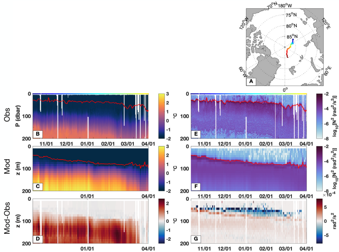
Fig. 14. ITP #111 section in the eastern Arctic. (a) Overhead map of ITP deployment, (b) observed temperature ( ^{\circ}\text{C} ), (c) modeled temperature ( ^{\circ}\text{C} ) along ITP deployment, (d) model-observed temperature difference ( ^{\circ}\text{C} ), (e) observed buoyancy frequency ( \text{rad}^2 \text{s}^{-2} ), (f) modeled buoyancy frequency ( \text{rad}^2 \text{s}^{-2} ), (g) model-observed buoyancy frequency difference ( \text{rad}^2 \text{s}^{-2} ). The mixed layer depth is shown as a red line in panels b,c,e, and f. Colors corresponding to locations in panel (a) are plotted across the tops of (b) and (e) (note that the profiler stopped collecting data partway through deployment).
