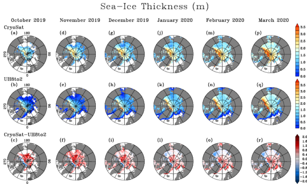
Fig. 7. Sea ice thickness (m) for CryoSat-2 (top), UH8to2 (middle), and their difference (bottom) in October 2019 through March 2020 (left to right).
