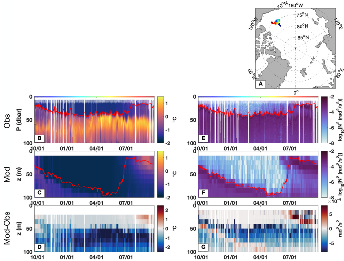
Fig. 15. ITP #114 section in the western Arctic (as in Fig. 14). (a) Overhead map of ITP deployment, (b) observed temperature ( ^{\circ}\text{C} ), (c) modeled temperature along deployment ( ^{\circ}\text{C} ), (d) model-observed temperature difference ( ^{\circ}\text{C} ), (e) observed buoyancy frequency ( \text{rad}^2 \text{s}^{-2} ), (f) modeled buoyancy frequency ( \text{rad}^2 \text{s}^{-2} ), (g) model-observed buoyancy frequency difference ( \text{rad}^2 \text{s}^{-2} ). The mixed layer depth is shown as a red line in panels b,c,e, and f. Colors corresponding to locations in panel (a) are plotted across the tops of (b) and (e).
