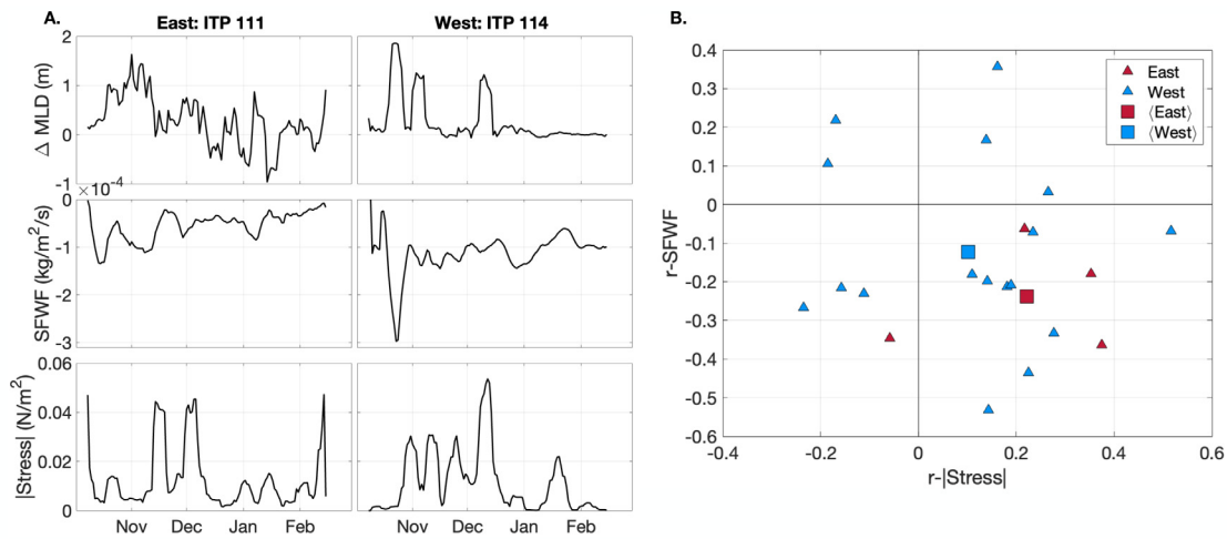
Fig. 17. A. 7-day smoothed time series of the change in mixed layer depth (m; top), net surface freshwater flux ( \text{kg m}^{-2} \text{s}^{-1} ; middle), and ice-ocean stress magnitude ( \text{N m}^{-2} ; bottom) in the eastern (left) and western (right) Arctic example ITP deployments. All quantities are for the synthetic UH8to2 ITP deployments. B. Partial correlations (triangles) of the winter change in mixed layer depth with net surface freshwater flux and ice-ocean stress magnitude for each synthetic ITP deployment that had at least 20 profiles between October and March of the following year. Partial correlations are calculated from the 7-day smoothed time series. Mean partial correlations for the eastern and western Arctic are shown as squares.
