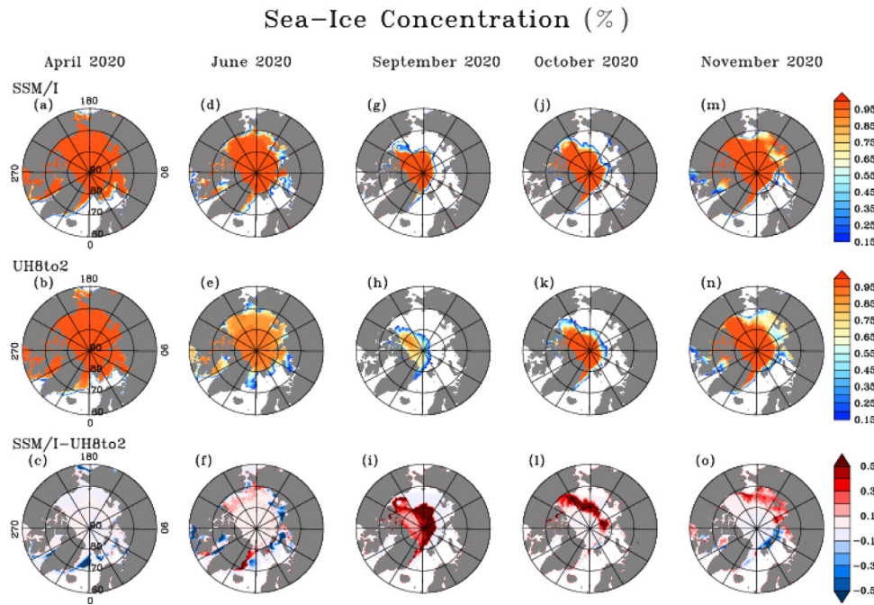
Fig. 6. Fractional sea ice concentration over areas with at least 15% ice concentration from SSM/I (top) and UH8to2 (bottom) in April (a and b), June (d and e), September (g and h), October (j and k), and November (m and n) of 2020. Differences between SSM/I and UH8to2 values are shown in panels c, f, i, l, and o.
