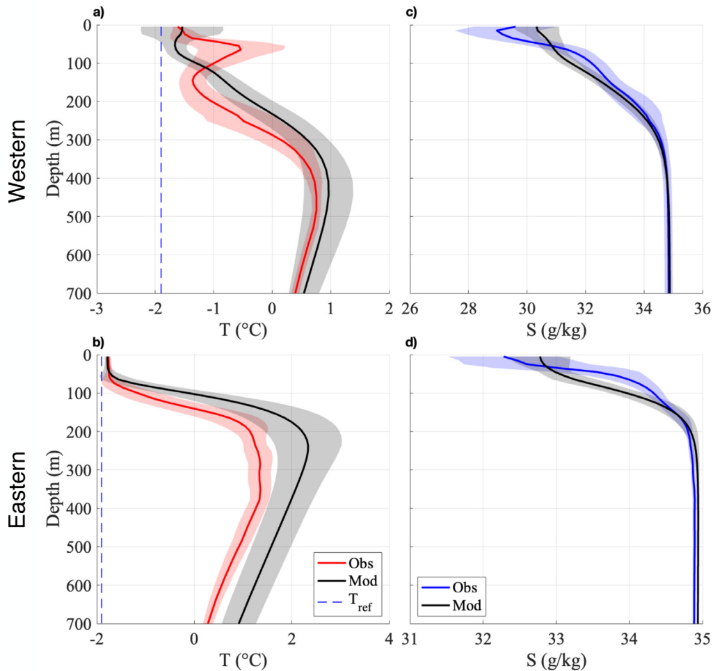
Fig. 10. Comparison of mean ITP-observed profiles (red and blue) and matched synoptic model profiles (black) of (a) temperature (°C) in the western Arctic (latitudes between 0 and 180 °W), (b) temperature (°C) in the eastern Arctic (latitudes between 0 and 180 °E), (c) salinity (g kg -1 ) in the western Arctic (latitudes between 0 and 180 °W), and (d) salinity (g kg -1 ) in the eastern Arctic (latitudes between 0 and 180 °E). Shaded regions represent a standard deviation around the mean. T_{ref} is the reference freezing temperature of -1.9 °C. In total the ITP record includes 4218 profiles in the east and 35724 profiles in the west.
