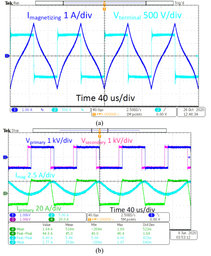
Fig. 1. The current waveform with ferrite gap: (a) balanced flux, (b) unbalanced flux.
