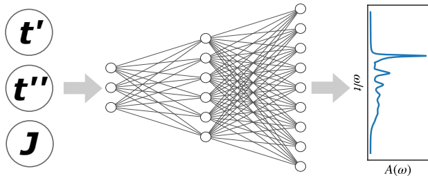
FIG. 2. A fully connected neural network, applied to the forward problem of predicting a DOS given t' , t'' , J . The neural network takes in a 3 dimensional vector representing t' , t'' , J , and outputs a 301 dimensional vector representing the predicted DOS.
