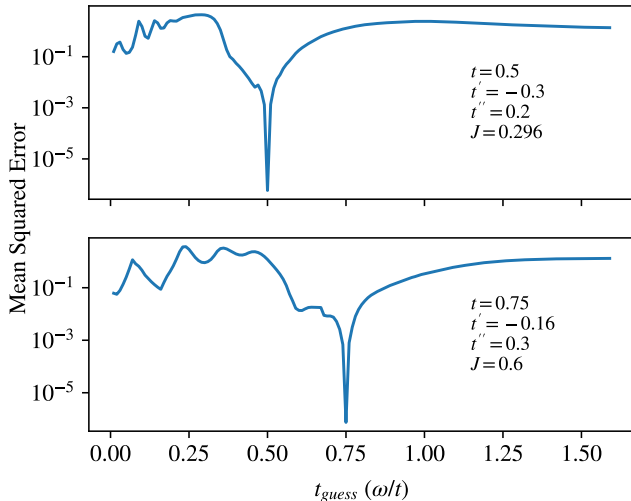
FIG. 7. The mean squared error when rescaling a mock “experimental” DOS in units of t_{\text{guess}} , and running FFNN to predict the ground truth t' , t'' , and J .
