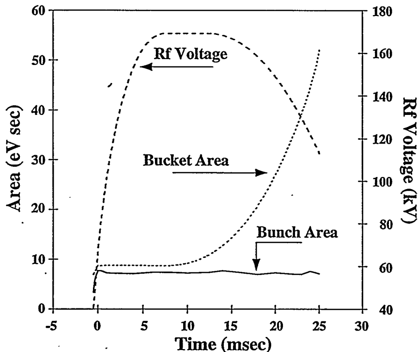
Figure 5: The Rf Voltage Program, Showing Bunch and Bucket Areas Over the Complete Cycle.
