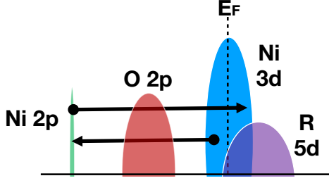
FIG. 1. Illustration of L edge RIXS for the nickelates in the approximation used in this paper. The upper arrow denotes excitation from the Ni 2p core electrons to the unoccupied Ni 3d states, the lower arrow denotes de-excitation from an occupied Ni 3d state that fills the Ni 2p core hole left from the first process. The analogous XAS process only involves the upper arrow. Here, E_F denotes the Fermi energy.
