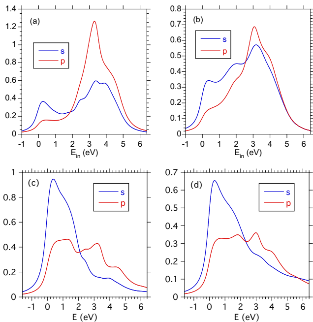
FIG. 5. Integration of RIXS spectra for RNiO_2 from 4-6 eV loss from DFT (a, R=La from Fig. 4(c-d)) and from DFT+DMFT (b, R=Nd from Fig. 4(e-f)). XAS for RNiO_2 from DFT (c, R=La ) and from DFT+DMFT (d, R=Nd ) with \theta=15^\circ .
