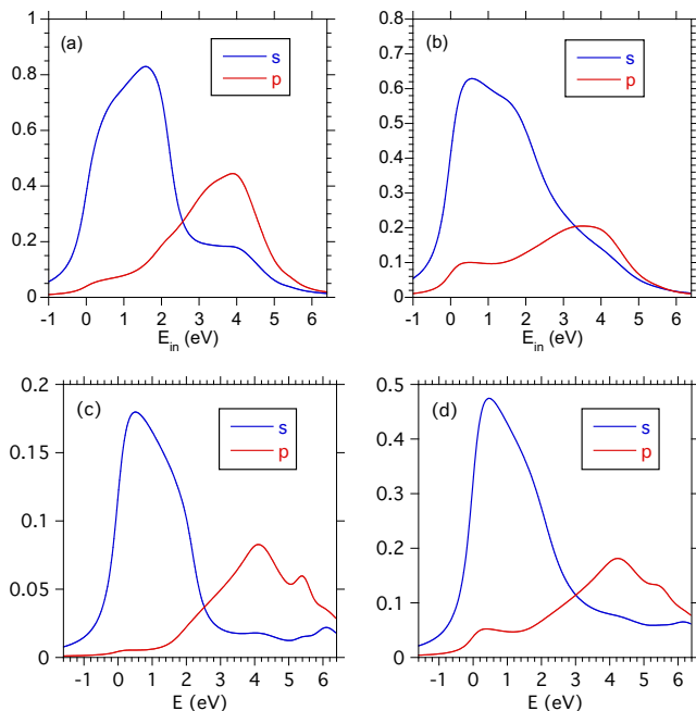
FIG. 7. Integration of RIXS spectra for \text{CaCuO}_2 from 4-6 eV loss from DFT (a, from Fig. 6(c-d)) and from DFT+DMFT (b, from Fig. 6(e-f)). XAS for \text{CaCuO}_2 from DFT (c) and from DFT+DMFT (d) with \theta=15^\circ .
