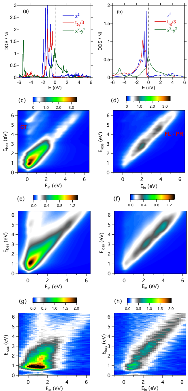
FIG. 2. Density of states for R_4\text{Ni}_3\text{O}_8 for the outer Ni planes from (a) DFT ( R=\text{La} ) and (b) DFT+DMFT ( R=\text{Pr} ). The ones for the inner Ni planes are similar. RIXS spectra for \text{La}_4\text{Ni}_3\text{O}_8 from DFT for s polarization (c) and p polarization (d). CT denotes the charge transfer feature, FL-PR the polarization reversal of the fluorescence line. RIXS spectra for \text{Pr}_4\text{Ni}_3\text{O}_8 from DFT+DMFT for s polarization (e) and p polarization (f). RIXS data for \text{La}_4\text{Ni}_3\text{O}_8 for s polarization (g) and p polarization (h) from Ref. 6, replotted as described in the text. For (c-h), \theta=15^\circ and 2\Theta_{sc}=153^\circ .
