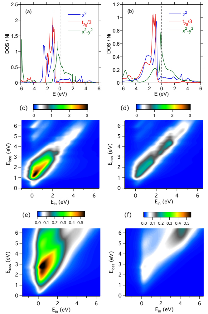
FIG. 4. Density of states for R\text{NiO}_2 from DFT (a, R=\text{La} ) and DFT+DMFT (b, R=\text{Nd} ). RIXS spectra for \text{LaNiO}_2 from DFT for s polarization (c) and p polarization (d). RIXS spectra for \text{NdNiO}_2 from DFT+DMFT for s polarization (e) and p polarization (f). For (c-f), \theta=15^\circ and 2\Theta_{sc}=153^\circ .
