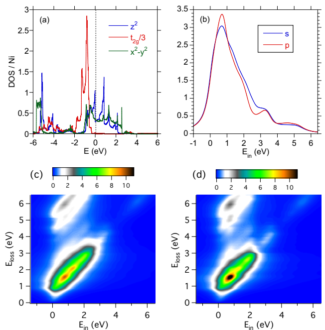
FIG. 8. Density of states for \text{La}_4\text{Ni}_3\text{O}_{10} from DFT (a). Integration of RIXS spectra for \text{La}_4\text{Ni}_3\text{O}_{10} from 4-6 eV loss from DFT (b). RIXS spectra for \text{La}_4\text{Ni}_3\text{O}_{10} from DFT for s polarization (c) and p polarization (d) with \theta=15^\circ and 2\Theta_{sc}=153^\circ .
