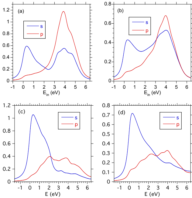
FIG. 3. Integration of RIXS spectra for R_4\text{Ni}_3\text{O}_8 from 4-6 eV loss from DFT (a, R=\text{La} from Fig. 2(c-d)) and from DFT+DMFT (b, R=\text{Pr} from Fig. 2(e-f)). XAS for R_4\text{Ni}_3\text{O}_8 from DFT (c, R=\text{La} ) and from DFT+DMFT (d, R=\text{Pr} ) with \theta=15^\circ .
