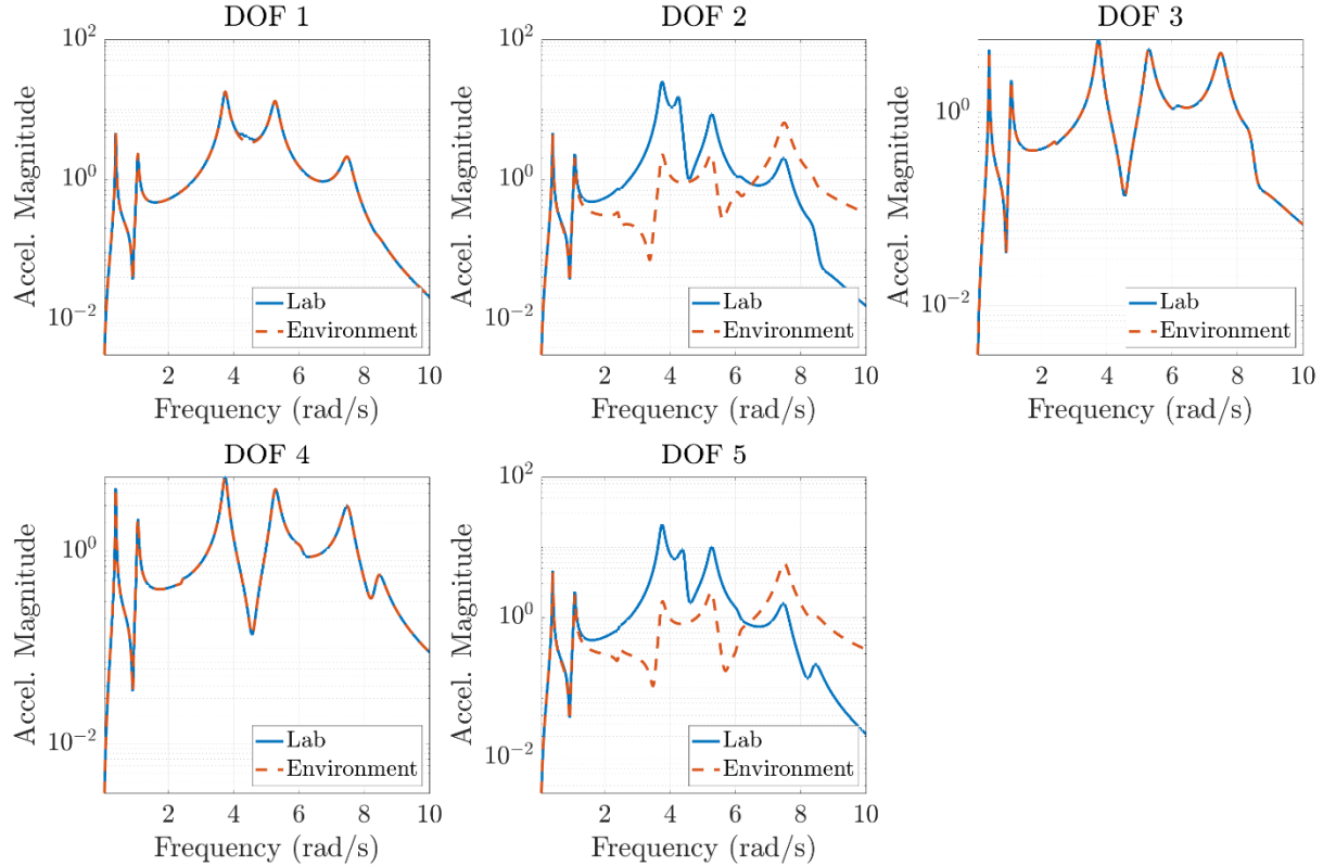
Figure 6: Response of subcomponent and TS for Case Study 1
