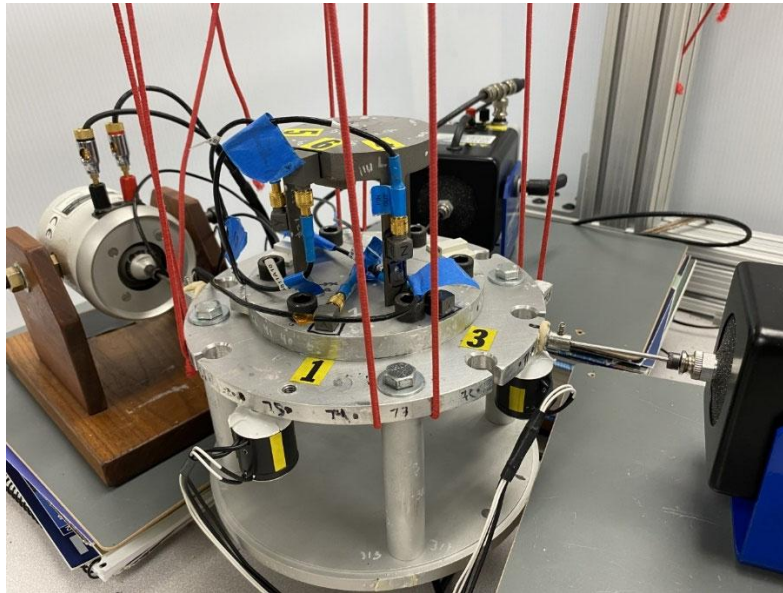
Figure 15. Test Setup on Configuration C with Shakers Attached to Interface Plate
