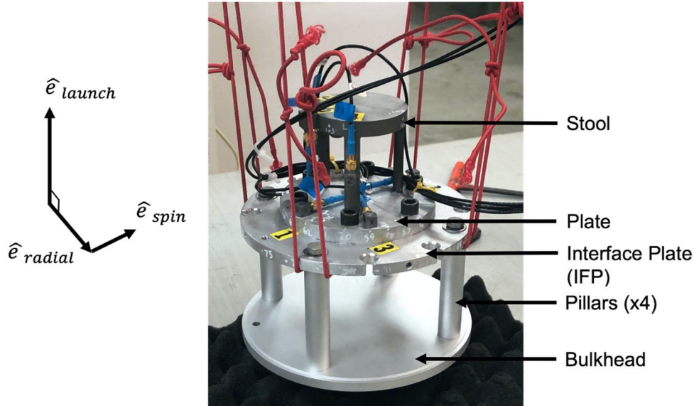
Figure 9: The instrumented next-level assembly
