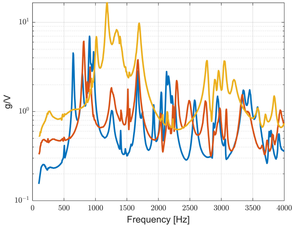
Figure 13: Composite of the Frequency Response Functions measured on each of the configurations: (yellow) Configuration A, (red) Configuration B, (blue) Configuration C
