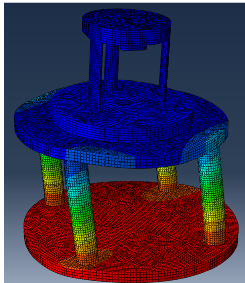
Figure 14. 2 nd Fixed Plate Mode of Configuration C, 451 Hz
