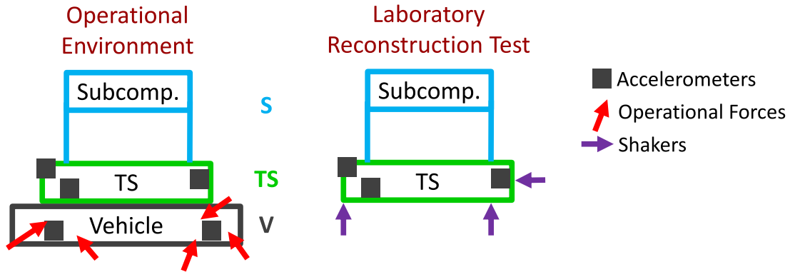
Figure 3: Schematic of a TS-IMMAT response reconstruction problem in which a subcomponent of interest ( S ) is connected to a vehicle ( V ) through a fixture called a Transmission Simulator ( TS ). In the laboratory, we seek to reconstruct the measured operational environment using shakers.
