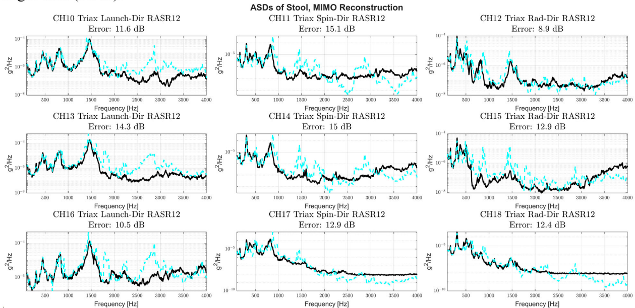
Figure 12: Measured ASDs of the uncontrolled accelerometers on the stool (cyan) along with the environment ASDs (black) for Configuration C
