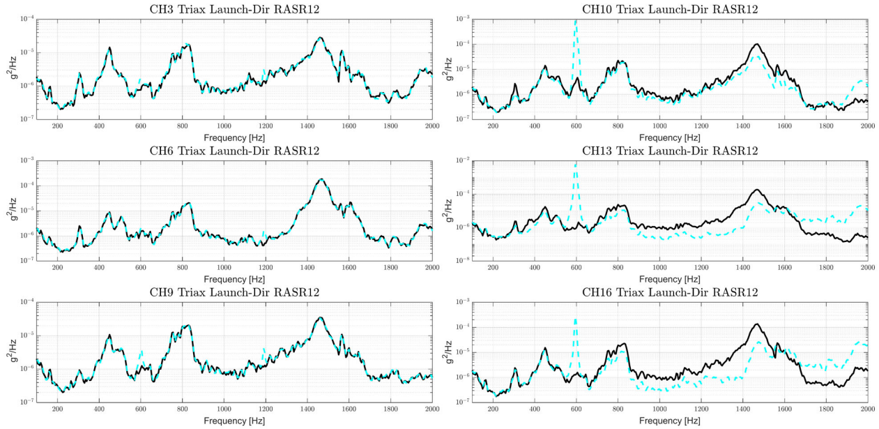
Figure 17: Response of the stool on plate system in the launch direction, with Plate accelerometers (CH3, CH6 and CH9) and Stool accelerometers (CH10, CH13 and CH16)
