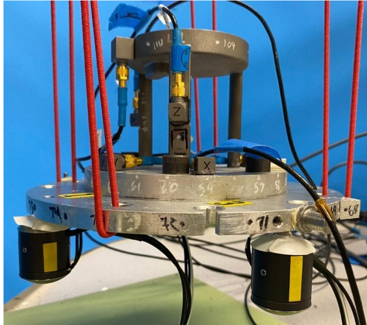
Figure 16: Photo of test setup for Configuration B-2 with three shakers in the launch direction and all others removed.
