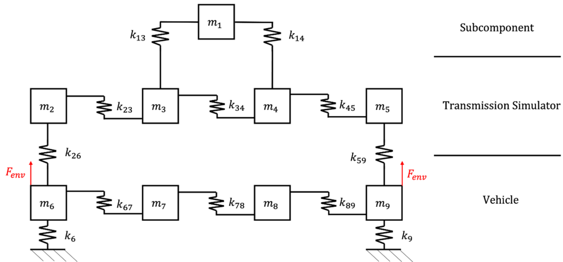
Figure 4: Mass-spring system representing a vehicle (V), transmission simulator (TS), and subcomponent (S). This corresponds to the actual operating configuration of the system.
