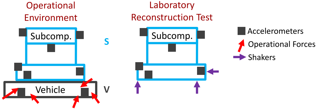
Figure 2: Schematic of a traditional environment response reconstruction problem in which measurements are taken on a subcomponent of interest ( S ) when it is connected to a vehicle ( V ). In the laboratory, we seek to reconstruct the measured operational environment at a set of measurement points using shakers.
