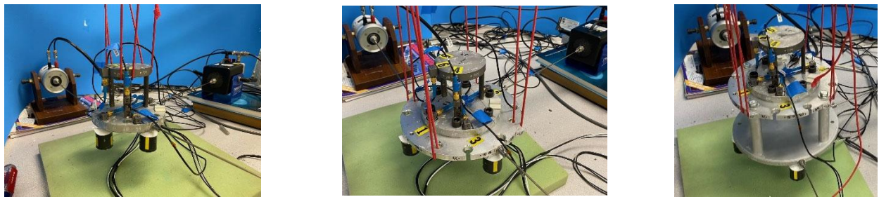
Figure 10: The three assemblies tested are Configuration A with the stool and plate, Configuration B with the stool, plate, and IFP, and Configuration C with the stool, plate, IFP, pillars, and bulkhead
