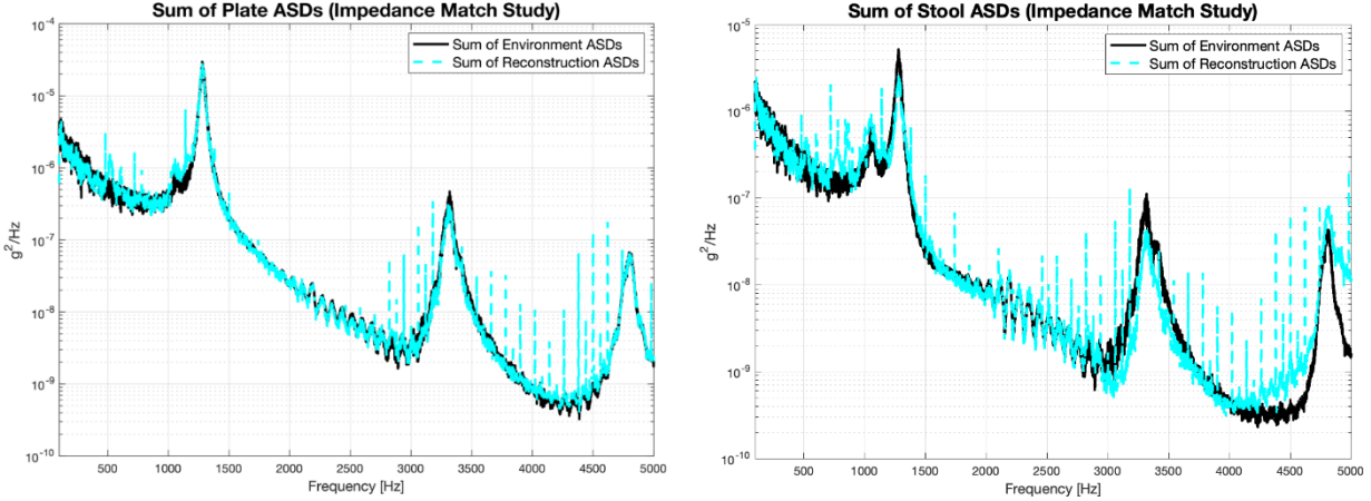
Figure 18: Measured ASDs of the plate (left) and the stool (right) from Configuration A-2, the case study where there is a near perfect impedance match between lab and the true environment.
