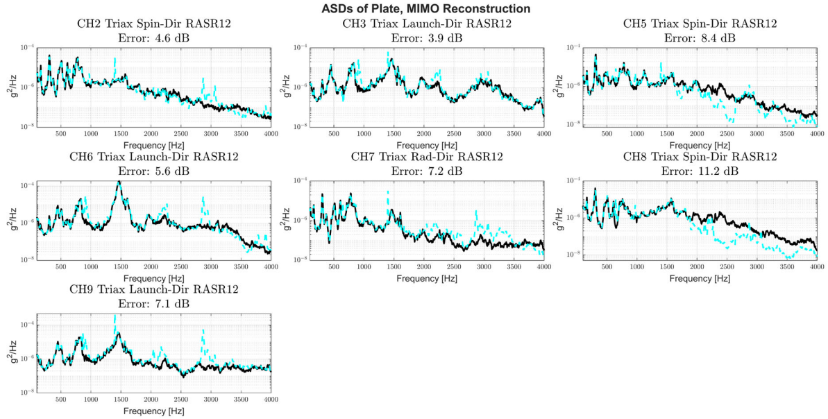
Figure 11: Reconstruction ASDs of the controlled accelerometers on the plate (cyan) along with the control ASDs (black) for Configuration C
