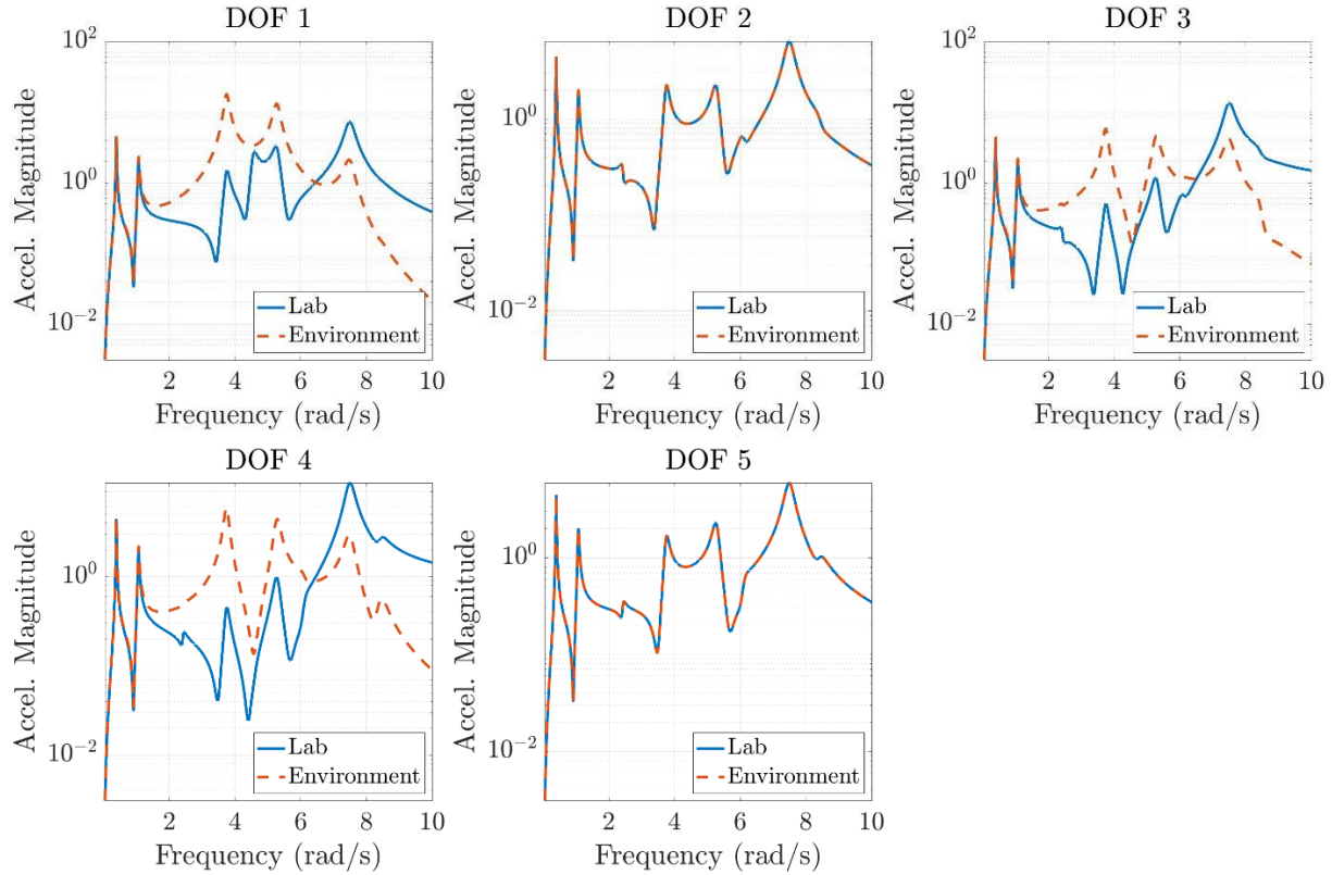
Figure 8: Response of subcomponent and TS for Case Study 2
