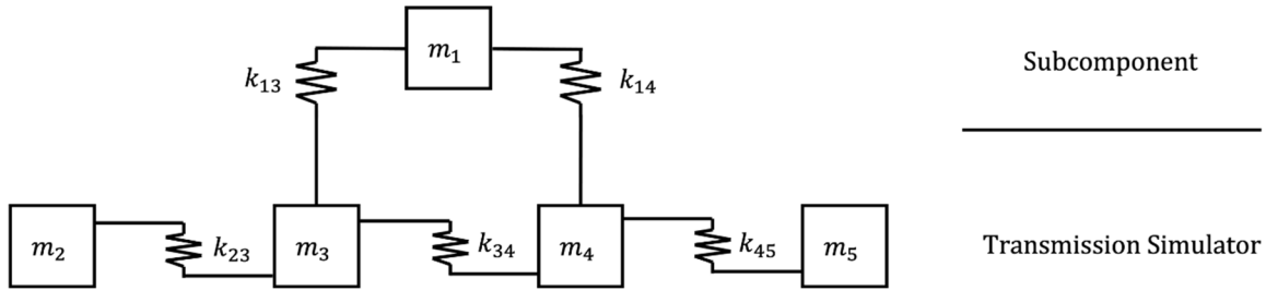
Figure 5: Mass spring system representative of an experimental setup that only includes a TS and subcomponent. This corresponds to the configuration tested in the laboratory.
