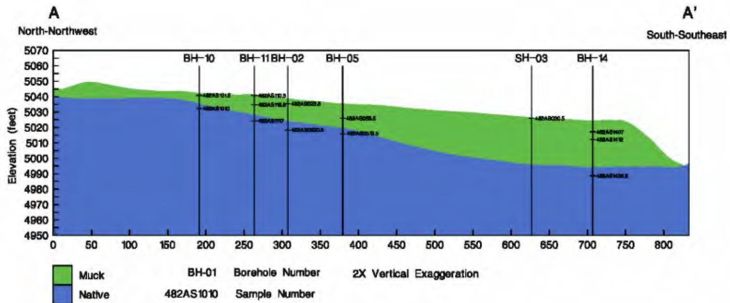
15a/e Muckpiles North-Northwest to South-Southeast Cross Section A-A'
