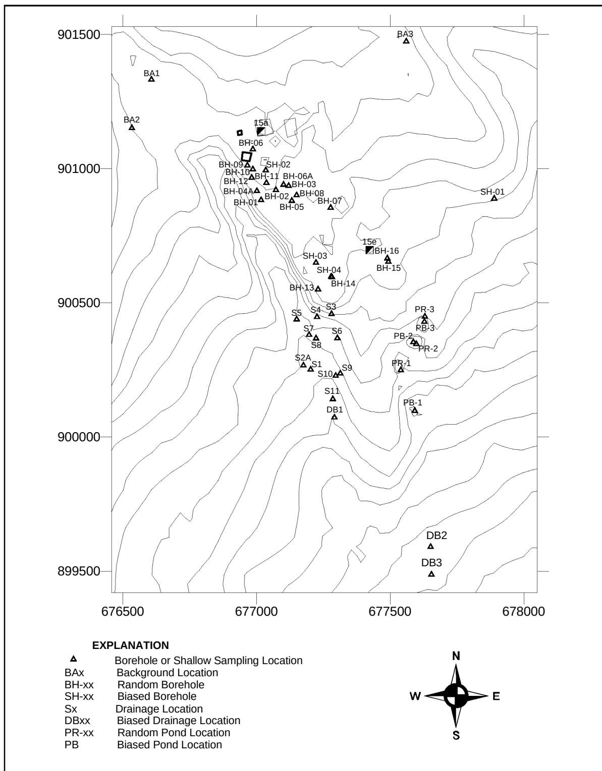
Figure A.3-2 As-Built Borehole and Sampling Locations
