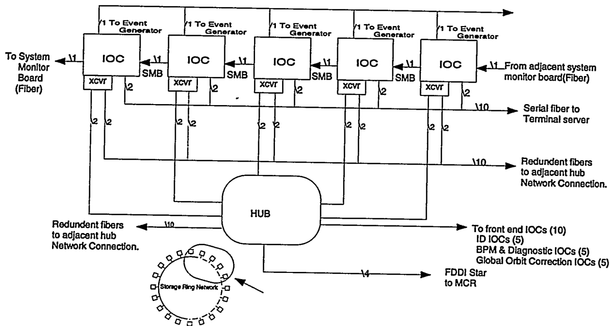
Figure 3 IOC Fiber Plant
