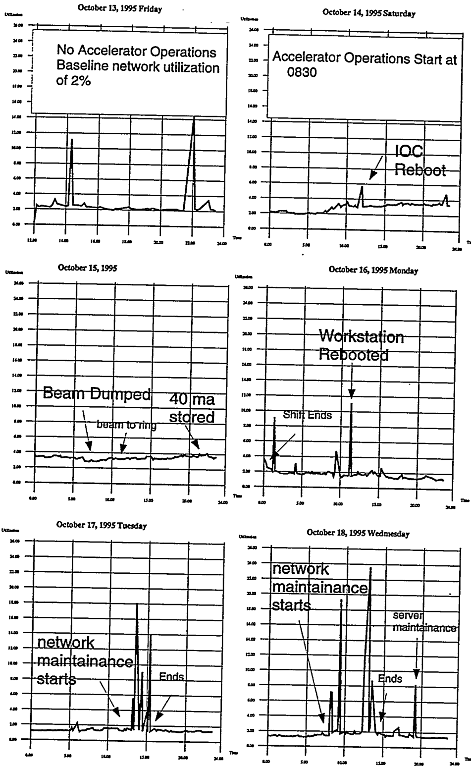
Figure 4. FDDI Performance
