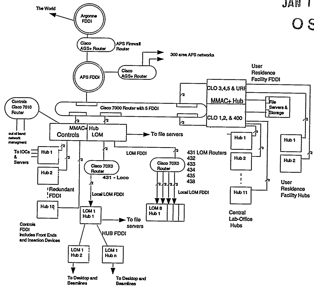
Figure 1 The APS Network
