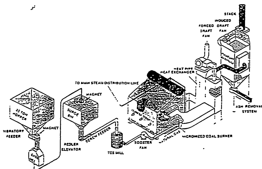
Figure 1 Micronized Coal Combustion System at Penn State
