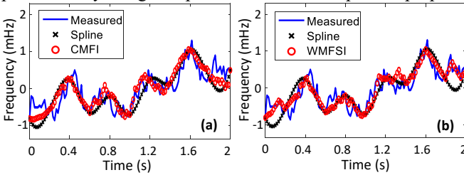
Fig. 3 Interpolation of frequency variations using (a) conventional multifractal interpolation and (b) proposed WMFSI method.
