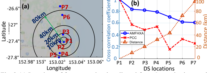
Fig. 2 (a) Locations of frequency signals collected from Queensland network and (b) cross-correlation coefficients between P1 and other six locations.
