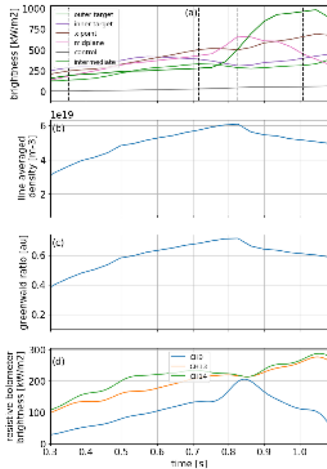
FIG. 25: Comparison of the measurements from different diagnostics for the shot 45401. In (a) is the IRVB brightness averaged inside the regions indicated with dashed lines in Figure 24 while the black lines indicate the time corresponding to the images in Figure 24. In (b) is the core line averaged density, (c) is the Greenwald density ratio and (d) is the brightness from the resistive bolometer core toroidal channel 9, 13 and 14, where the first corresponds to the midplane while the others to the intermediate regions of the IRVB.
