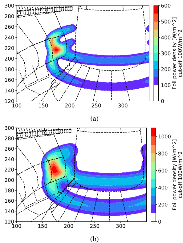
FIG. 6: Radiated power deposited on foil, modeled with CHERAB, of two toruses of 4 cm minor radius separated by 16cm in vertical position with uniform emissivity such as to total 0.5MW of radiated power, located at the expected x-point location. The pinhole size was varied from 4mm (a) to 6mm (b) to illustrate the loss of spatial resolution. The power deposited on the foil below 100W/m^2 is not shown, as that is the minimum desired signal level. Only the relevant section of the foil is shown. In black are overlaid the projection of relevant features of MAST-U structure on the foil for reference.
