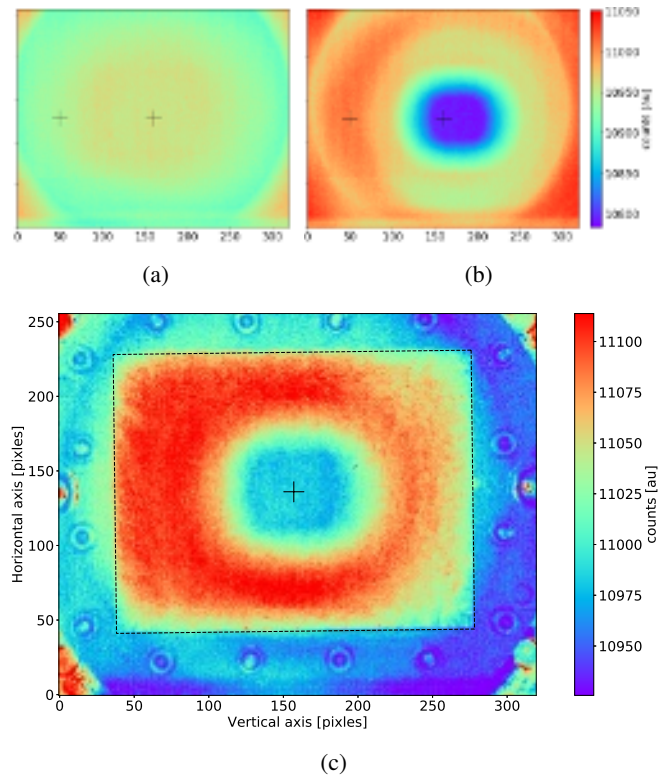
FIG. 11: Example of non uniformity of the counts of the IR camera when aimed at the NUC plate at room temperature. Shown are the images without the view port (a) and with (b). The same scale is applied to both plots and there was a 2ms integration time. The black cross indicates two reference points (inside/outside the narcissus) that will be used in later analysis. c shows the position of the foil (the red square) inside the camera field of view. Around the foil are the bolts that lock the foil in between the two copper plates, that can be used to identify the foil orientation.
