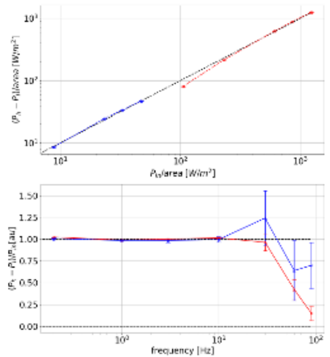
FIG. 17: Variation of the measured power compared to the expected values with laser intensity (top) and frequency (bottom). The blue color indicates the defocused cases while the red the focused ones. P_h and P_l are the inferred high and low power level of the laser square wave, area is the area of the foil receiving laser light, P_{in} is the known peak laser power density.
