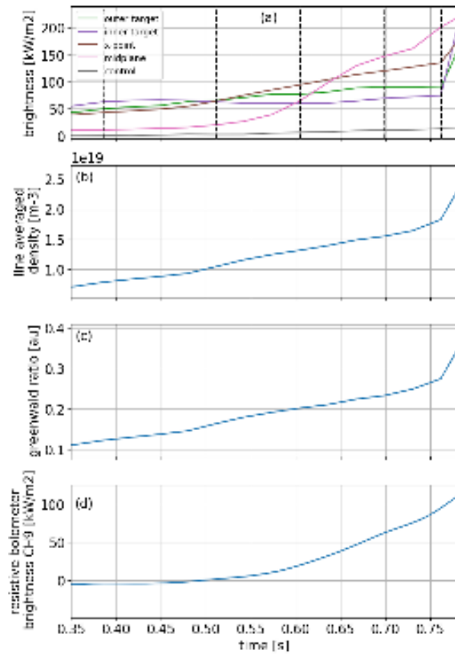
FIG. 23: Comparison of the measurements from different diagnostics for the shot 45473. In (a) is the IRVB brightness averaged inside the regions indicated with dashed lines of matching colors around the x-point and other regions in Figure 22 while the vertical black lines indicate the time corresponding to the images in Figure 22. In (b) is the core line averaged density, (c) is the Greenwald density ratio and (d) is the brightness from the resistive bolometer core toroidal channel 9.
