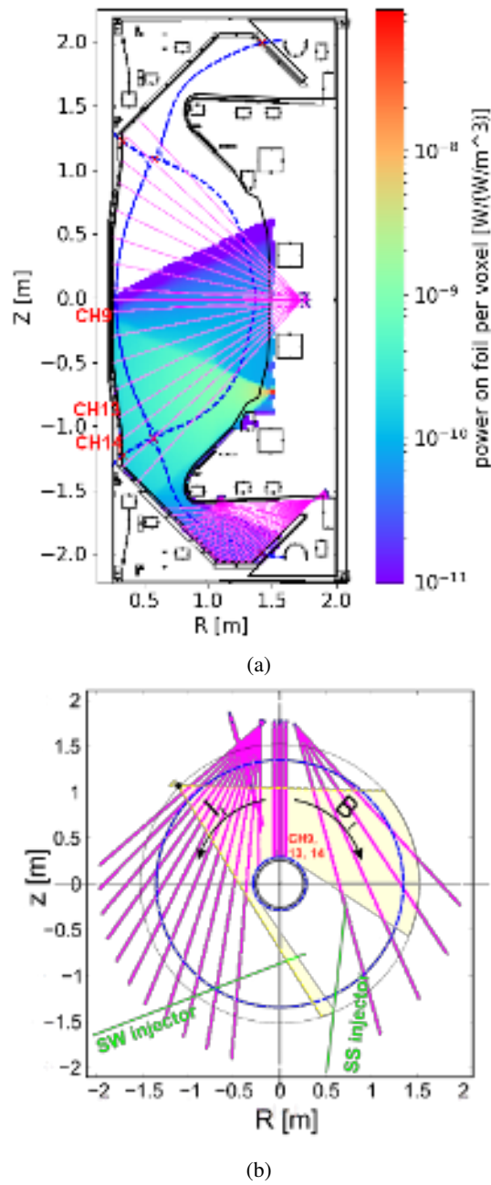
FIG. 8: (a) Poloidal view of MAST-U showing the comparison of the resistive bolometer system LOS (magenta) with a color plot obtained by scanning all the voxels with a 1\text{W}/\text{m}^3 emitter and integrating the power absorbed by the foil, indicating the regions of higher sensitivity of the IRVB. (b) Top view of MAST-U showing the position of neutral beam injectors (NBI, green), of the co- and counter-NBI resistive bolometer LOSs and the IRVB FOV (yellow, mostly counter-NBI). Adapted from 27 . For reference the separatrix of a typical plasma is shown as an overlay of a blue dashed line. The resistive bolometer LOSs that will be used in the later analysis are here identified.
