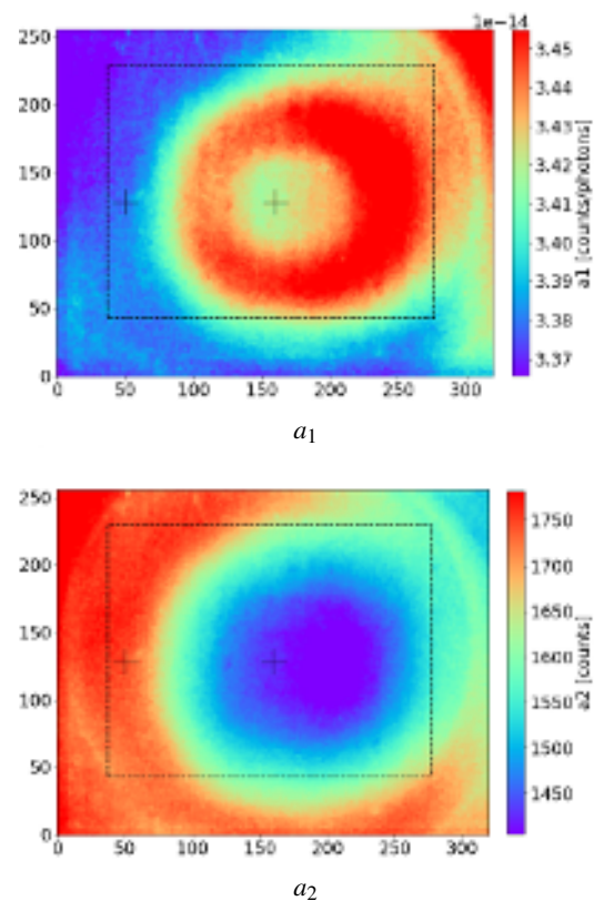
FIG. 14: a_1 and a_2 coefficients of Equation 3 obtained via calibration with the NUC plate. In black is highlighted the region corresponding approximately to the IRVB foil and the two reference points defined in Figure 11. The vertical orientation during this calibration is right to left, with the top on the left.
