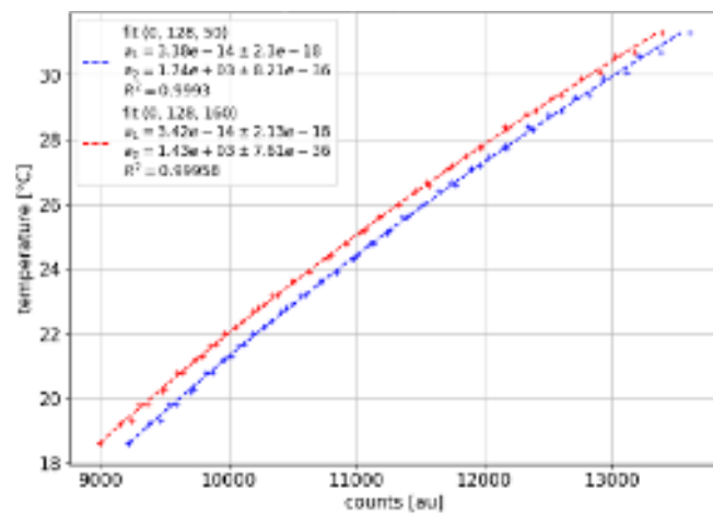
FIG. 13: Comparison of the temperature calibration curves for a pixel at the centre of the narcissus (red) with one on its side (blue). The legend gives the fit parameters ( a_1 proportional and a_2 additive components), their uncertainties, and the coefficient of determination of the fit.
