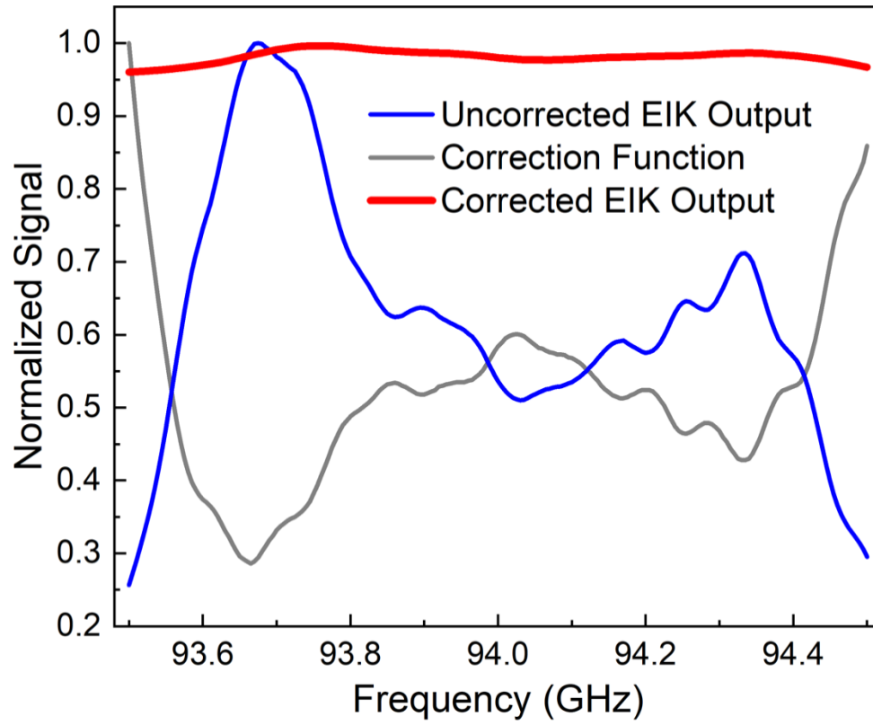
Fig. 3. Uncorrected EIK output power in the 93.5 to 94.5 GHz frequency range, together with the correction function that is used to obtain an approximately frequency-independent (flat) corrected EIK output; all curves are normalized to their maximum values.
