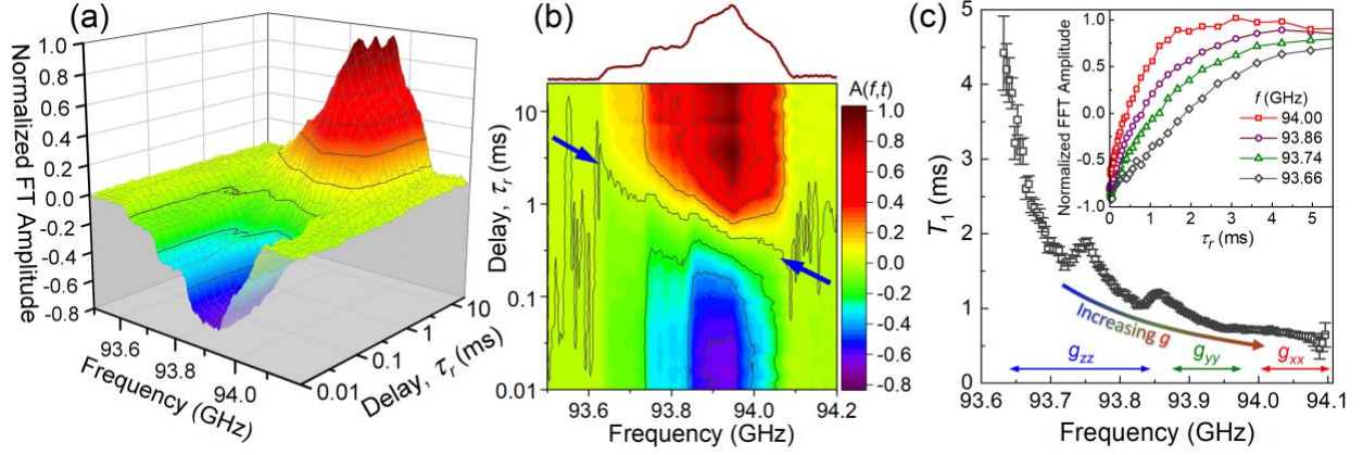
Fig. 5. (a) 3D plot of normalized 50 K FT spectra of a 0.25 mM TEMPOL sample as a function of relaxation delay time, \tau_r , for the inversion recovery pulse sequence depicted in Fig. 1c; the magnetic field was set to B_0 = 3.3445 T, with \tau_{AP180} = 10 \mu s, \tau_{FP90} = 700 ns, \tau_d = 600 ns, 20,000 averages and 45 Hz repetition rate. (b) 2D false color map corresponding to the data in (a), with a representative long delay time spectrum shown at top. The blue arrows indicate the frequency-dependent delay times where the FT amplitude passes through zero. (c) Frequency- (or orientation-) dependence of the spin-lattice relaxation time, T_1 , obtained by performing single exponential fits to the FT amplitude as a function of \tau_r across the full spectrum; representative time traces are shown in the inset, and error bars represent the standard error associated with the exponential fits. A strong ( \sim 5 -fold) variation in T_1 is observed for regions of the spectrum corresponding to different orientational components of the g -tensor (labeled at bottom).
