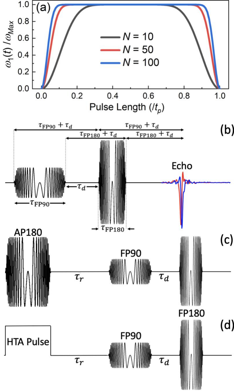
Fig. 1. (a) Amplitude profiles, \omega_1(t) , for the WURST pulse, with different values of N [Eq. (3)]. (b) Bodenhausen spin echo sequence with WURST pulses [ B_1(t) given by Eq. (1)], with the excitation pulse (FP90) being twice long as refocusing pulse (FP180); a typical quadrature detected chirped echo of TEMPOL is shown in blue (I) and red (Q). (c) Inversion recovery pulse sequence, where the spectrum is first inverted with an adiabatic \pi -pulse (AP180), followed by a Bodenhausen detection sequence. (d) CHEESY-detected NMR pulse sequence, where the AP180 pulse in (c) is replaced with a high-turning angle (HTA) saturating pulse. The horizontal axes are not to scale in (c) and (d).
