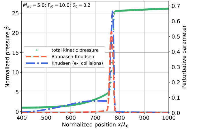
(b) The Bannasch-Knudsen number (protons), the degenerate Knudsen number (electrons), and the total kinetic pressure vs. position for a WDM shock ( \Gamma_{i0} = 10 , \theta_0 \approx 0.2 , and M_{wc} = 5 ).
