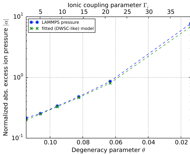
Figure 4: The normalized excess proton pressure, \alpha vs. the ionic coupling parameter, \Gamma_i and the electron degeneracy parameter, \theta . The blue circles are obtained from LAMMPS Yukawa-OCF MD simulations, and the green crosses are from the fit function: \alpha_{\text{fit}} = -0.17651319\Gamma_i + 0.11731267.
