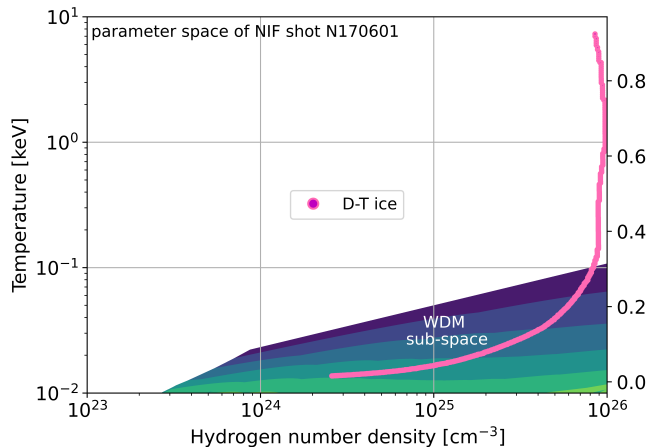
Figure 3: A selection of the range of temperatures and densities visited by a radiation-hydrodynamic simulation of NIF shot N170601. 17 The shaded area represents the sub-space which abides by the WDM orderings from Eq. (7), and the magenta curve is the characteristic path of the D-T ice layer through \rho - T space. The leftmost edge of this curve represents the time of the main shock rebound from the capsule center, and the rightmost edge is near peak thermonuclear reactivity.
