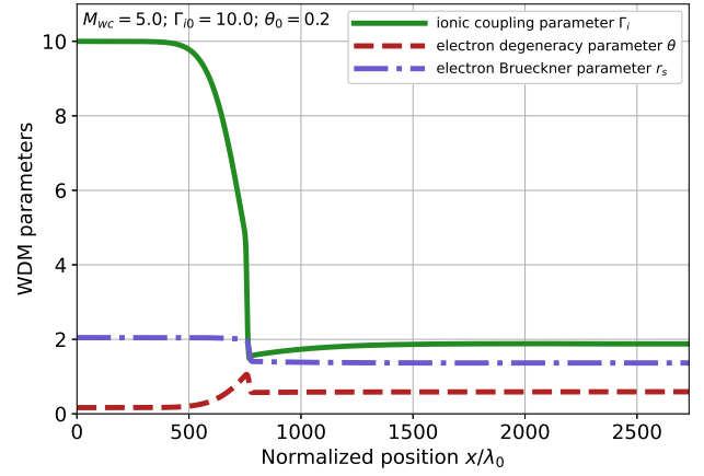
Figure 8: Key WDM parameters vs. position for a WDM shock with \Gamma_{i0} = 10 , \theta_0 \approx 0.2 , and M_{wc} = 5 .
