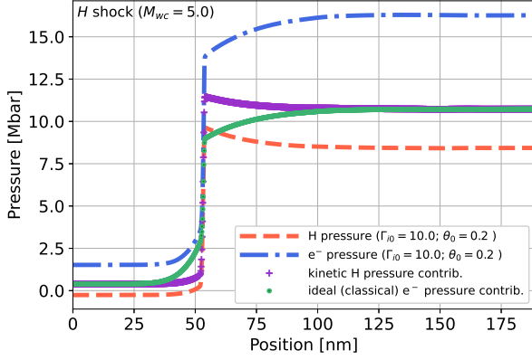
Figure 6: The proton and electron pressures for a WDM shock with \Gamma_{i0} = 10 , \theta_0 \approx 0.2 , and M_{wc} = 5 .
