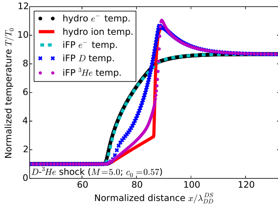
Figure 2: Normalized temperature profiles for a non-degenerate/weakly-coupled, D-^3He , hydrogen plasma shock with M = 5 at steady-state in a planar geometry. Here, the solutions labeled iFP are from a Vlasov-Fokker-Planck code – which is fully kinetic for the ions, but uses a fluid electron model. The hydro curves are obtained from the SHion shock code. Reproduced with permission from Keenan et al. , Phys. Rev. E 96 , 053203 (2017). Copyright 2017 American Physical Society.
