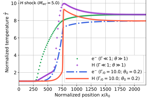
(a) Proton and electron temperatures.
