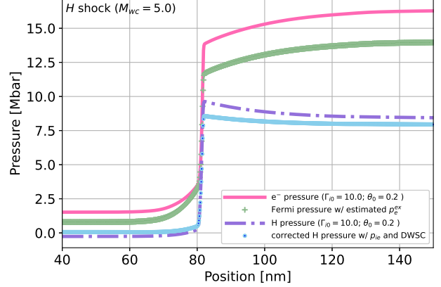
(a) The proton and electron pressures.
