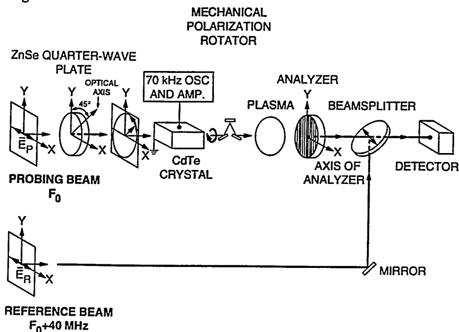
Figure 1. Illustration of the electro-optic polarization-modulation technique used in the CO 2 laser polarimeter on Alcator C-Mod.
