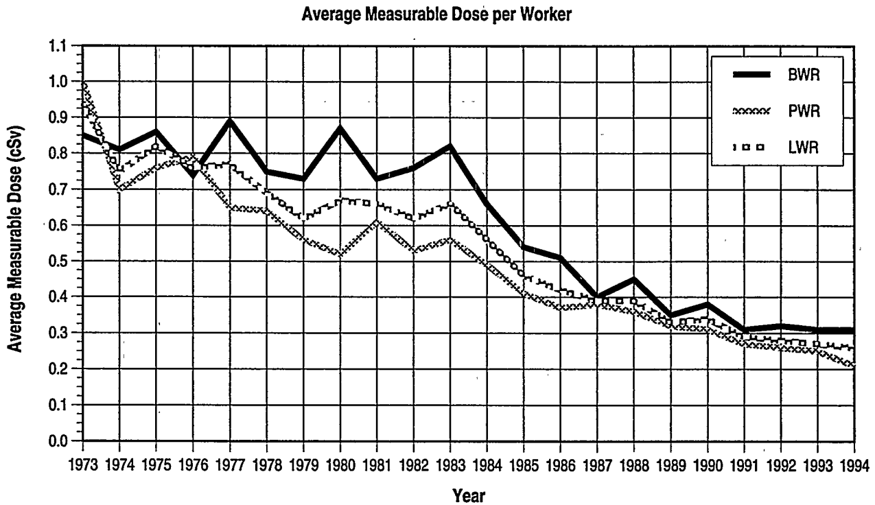
Figure 4.3 Average Measurable Dose per Worker and Collective Dose per Megawatt-Year 1973 – 1994
