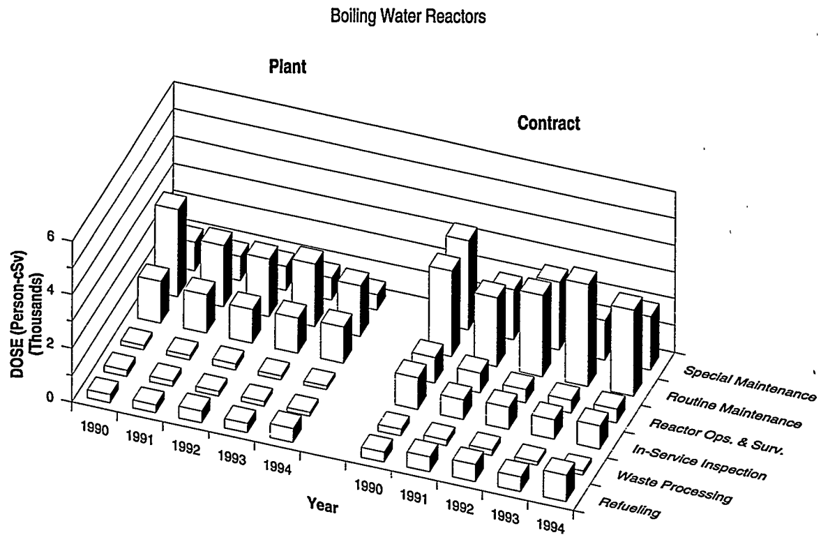
Figure 4.6 Collective Dose by Work Function and Personnel Type 1990 – 1994
