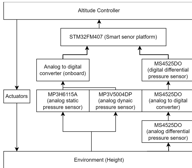
Figure 17. Approximate control block diagram for the VCU smart sensor and interaction with controller.
