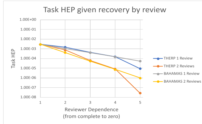
Figure 45. Comparison of BAHAMAS and THERP predictions of human error while considering the quality of review activities. X-axis = step increase in review quality quality.
