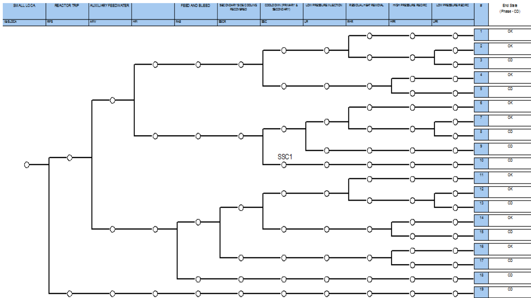
Figure 60. Generic PWR ET for small-break LOCA (INT-SLOCA).
