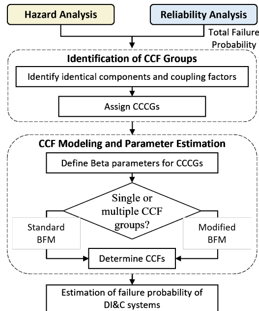
Figure 47. Flowchart for Software CCF Modeling and Estimation.
