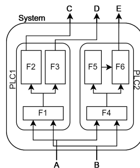
Figure 28. Mock DI&C control block diagram with two PLCs, each with three identified relevant modules.
