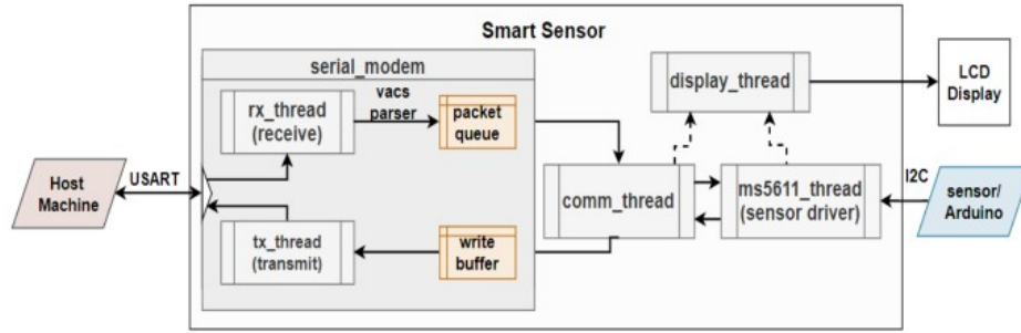
Figure 35. High-level block diagram of the VCU smart sensor device [33].
