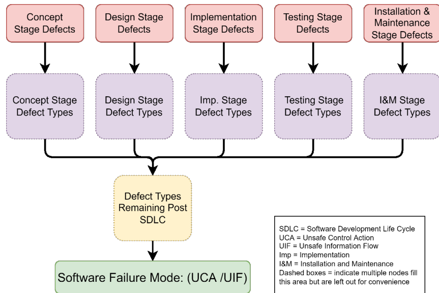
Figure 40. A conceptual BBN.
