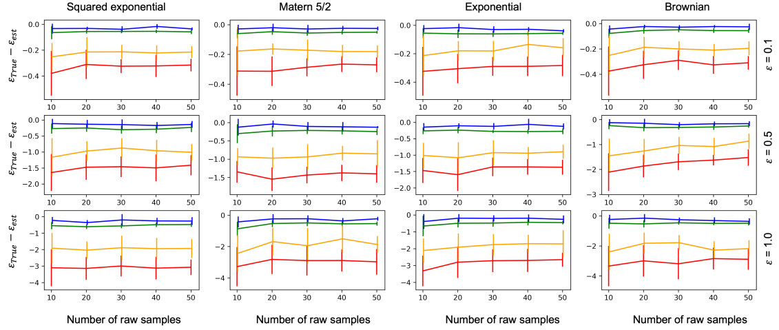
Figure 2: Figure 2. Robustness to Bayesian-inference-based parameter determination. The deviation in identifying the correct value of \epsilon under each case. Red, orange, green, and blue indicating L(m_i|D(m_j)) for L(Lap|D(Lap)) , L(Gaus|D(Lap)) , L(Lap|D(Gaus)) and L(Gaus|D(Gaus)) respectively. A greater \epsilon increases the difficulty in identifying \epsilon . The most difficulty is shown with L(Lap|D(Lap)) , while the greatest ease is shown with L(Gaus|D(Gaus)) . There also appears to be a subtle reduction estimate error with increasing number of data points. Error bars are slightly shifted for visibility.
