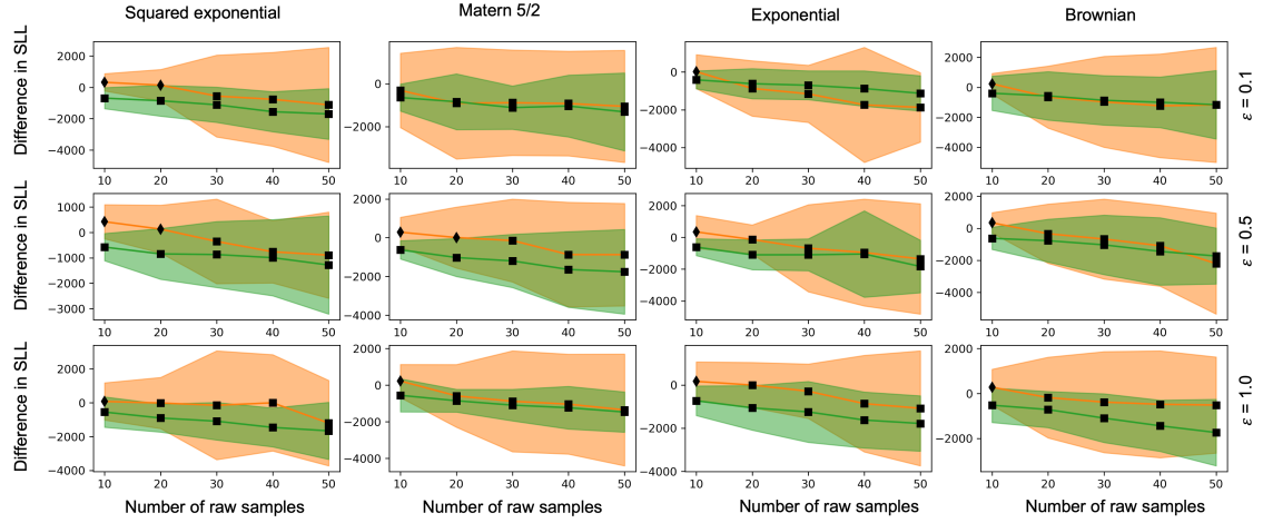
Figure 1: Figure 1. Robustness to Bayesian inference-based model determination. The difference in sum log likelihood (SLL) \Delta_{ij} = L_{ij} - L_{ij} for each investigated case. \Delta_{Laplace} is plotted in orange and \Delta_{Gaussian} is plotted in green with the mean indicated by a solid line and standard deviation indicated by the colored region. Diamond markers indicate a positive mean value and squares indicate a negative mean value - these correspond to the wrong and right policy having greater likelihood, respectively.
