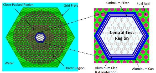
Fig. 1. Cross sectional view of the assembly core.
