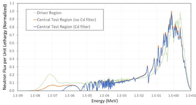
Fig. 4. Neutron spectra in the Ta rods.
