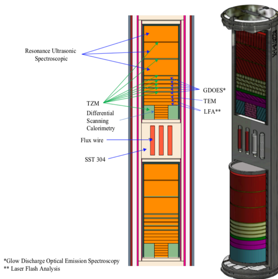
Figure 7.3. Hydride specimens located in a single ATR fixture basket. Two TZM inner capsules containing the hydride fit within a single ATR fixture, along with passive temperature and fluence monitors.
