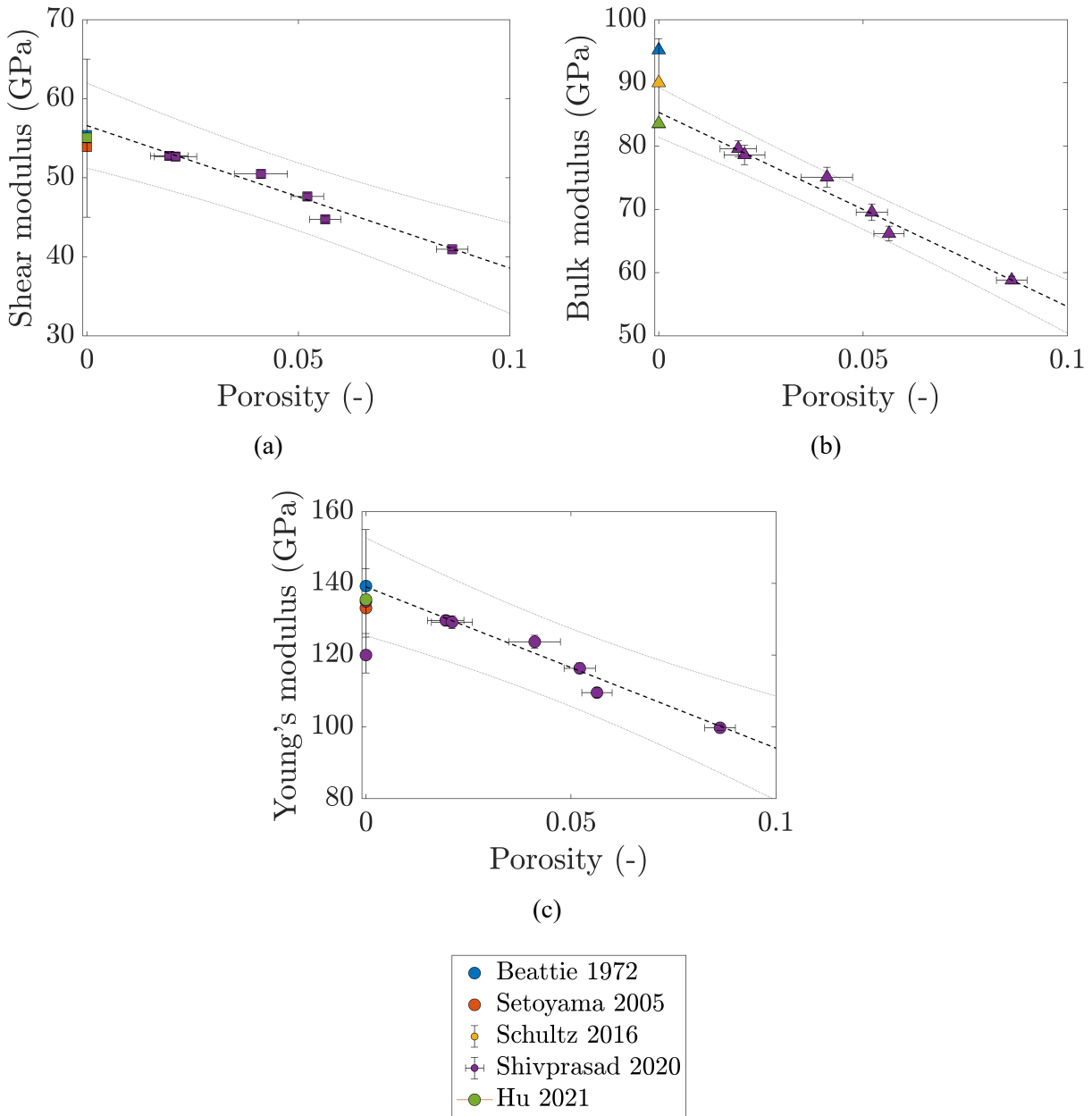
Figure 4.9: (a) Shear, (b) bulk, and (c) Young's moduli of yttrium dihydride as a function of porosity. Data from [2], [14], [36], [83], [85].
