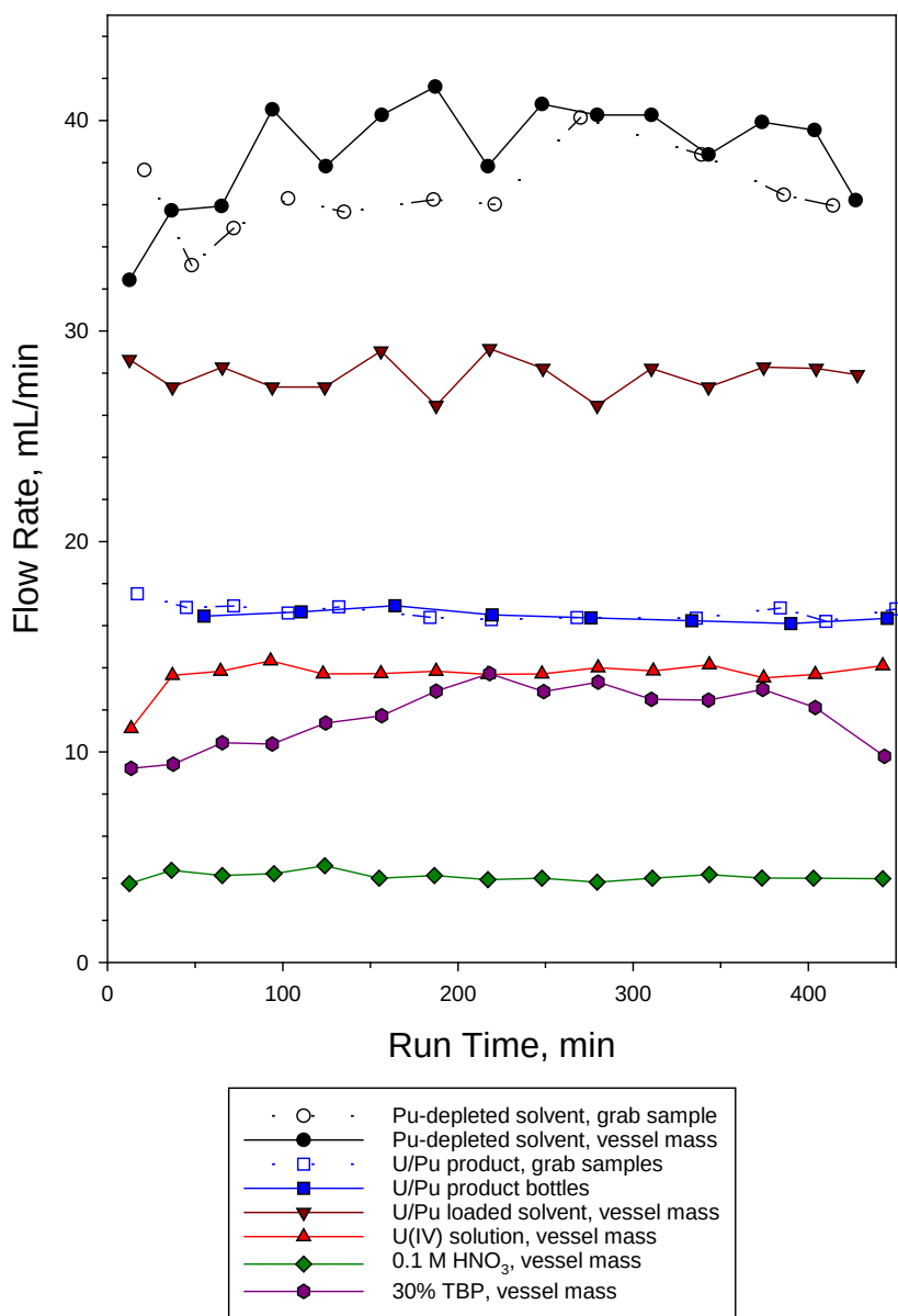
Figure 4.5. Flowrate data obtained during Run 4 reductive stripping.
