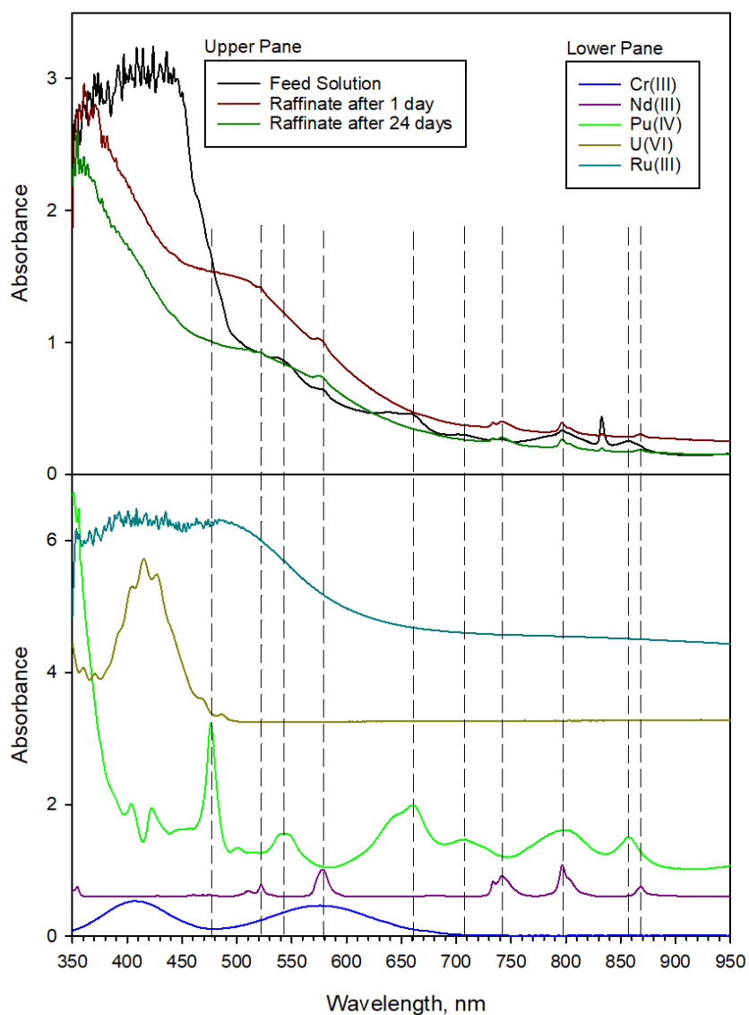
Figure 4.4. UV-vis spectra of the aqueous feed and raffinate from the Run 4 solvent loading (upper pane), and of Cr(III), Pu(IV), U(VI), and [Ru(NO)(NO 3 ) 3 ] in 3 M HNO 3 , and Nd(III) in 6 M HNO 3 (lower pane).
