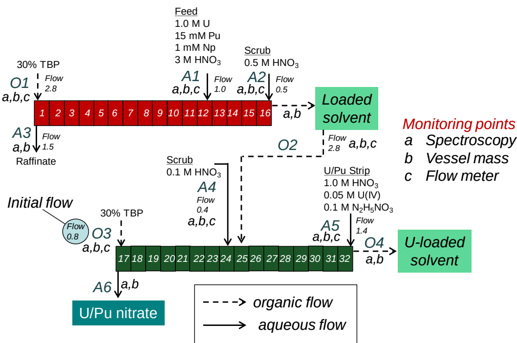
Figure 4.1. CoDCon flowsheet tested in Run 4.
