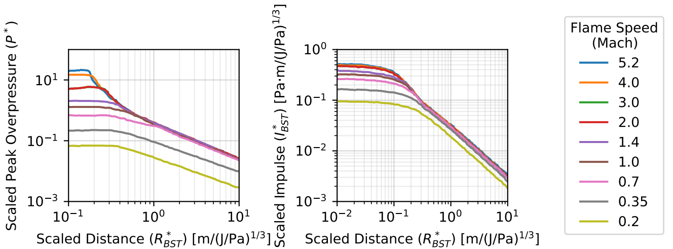
Figure 3-4 Mapping of scaled distance to scaled overpressure (left) and scaled impulse (right) for the BST unconfined overpressure model [2].
