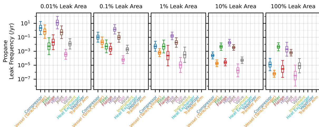
Figure 2-5 Box and whisker plot of propane (same default values for both gaseous and liquid) leak frequencies for the different components and each leak size. The thick central line is the median leak frequency, the boxes show the 25 th and 75 th percentiles of the distribution and the whiskers show the 5 th and 95 th percentiles.
