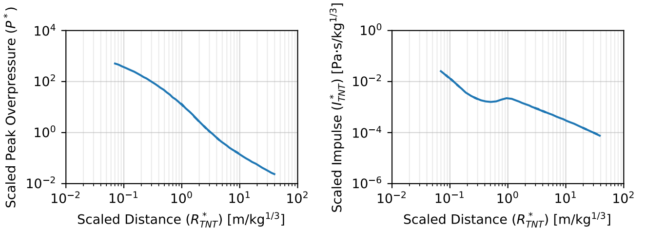
Figure 3-5 Mapping of scaled distance to scaled overpressure (left) and scaled impulse (right) for the TNT equivalence unconfined overpressure model [2].
