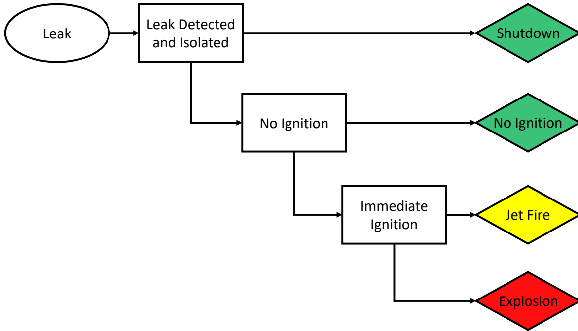
Figure 2-1 Event sequence diagram used by HyRAM+ for flammable gas releases [4].
