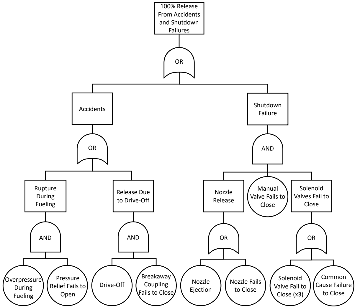
Figure 2-6 Fault tree for Other Releases from a dispenser [4].
