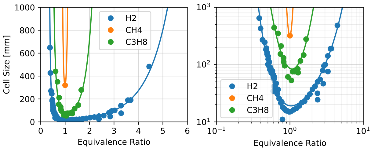
Figure 3-6 Detonation cell size data (points) from the detonation database [69] and fits to the data (lines) on a linear (left) and logarithmic (right) scale.
