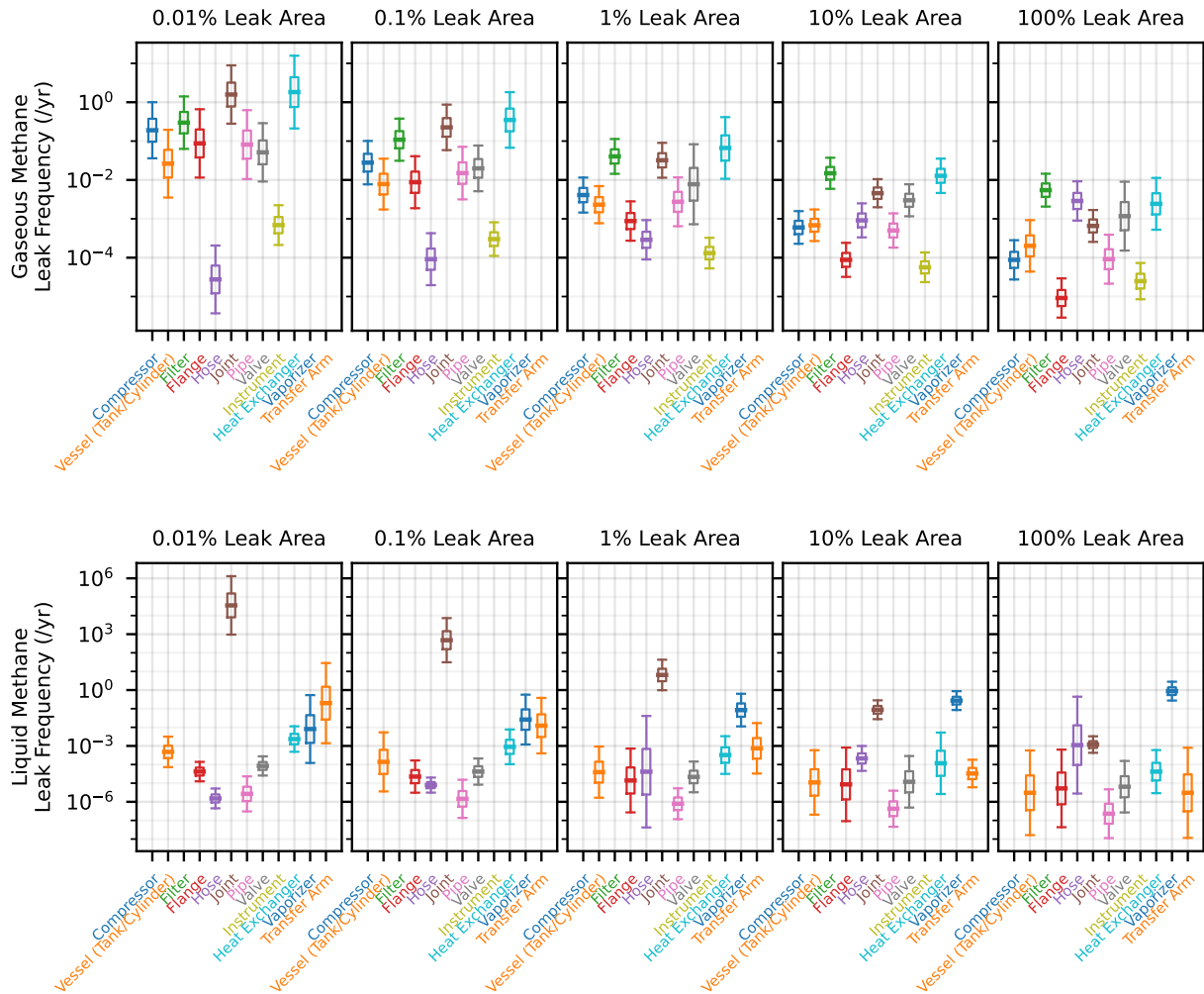
Figure 2-4 Box and whisker plots of gaseous methane (top) and liquid methane (bottom) leak frequencies for the different components and each leak size. The thick central line is the median leak frequency, the boxes show the 25 th and 75 th percentiles of the distribution and the whiskers show the 5 th and 95 th percentiles.
