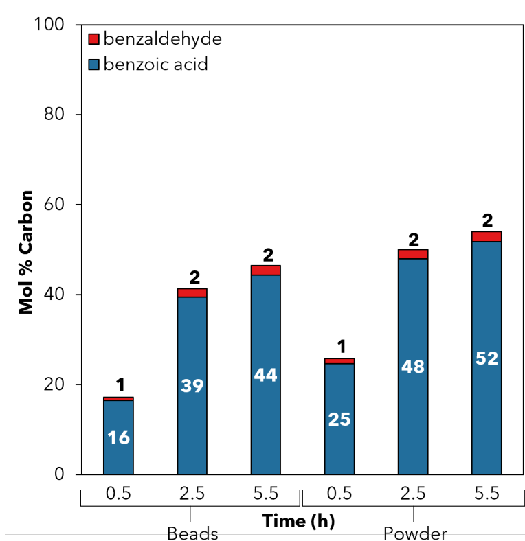
Figure S4. Oxidation of commercial resin PS and powder.
