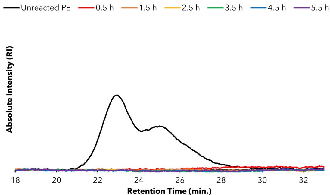
Figure S12. GPC chromatograms for deconstruction of HDPE at different reaction times.
