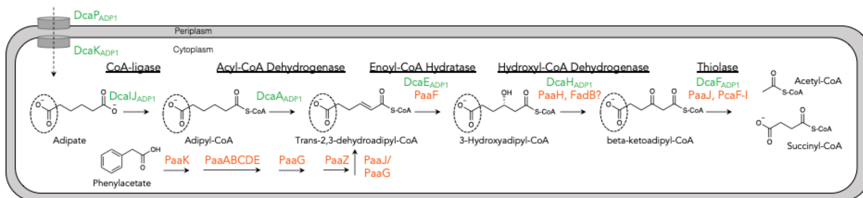
Figure S25. Proposed metabolic pathway for catabolism of adipate and phenylacetate by a metabolically engineered P. putida strain.
