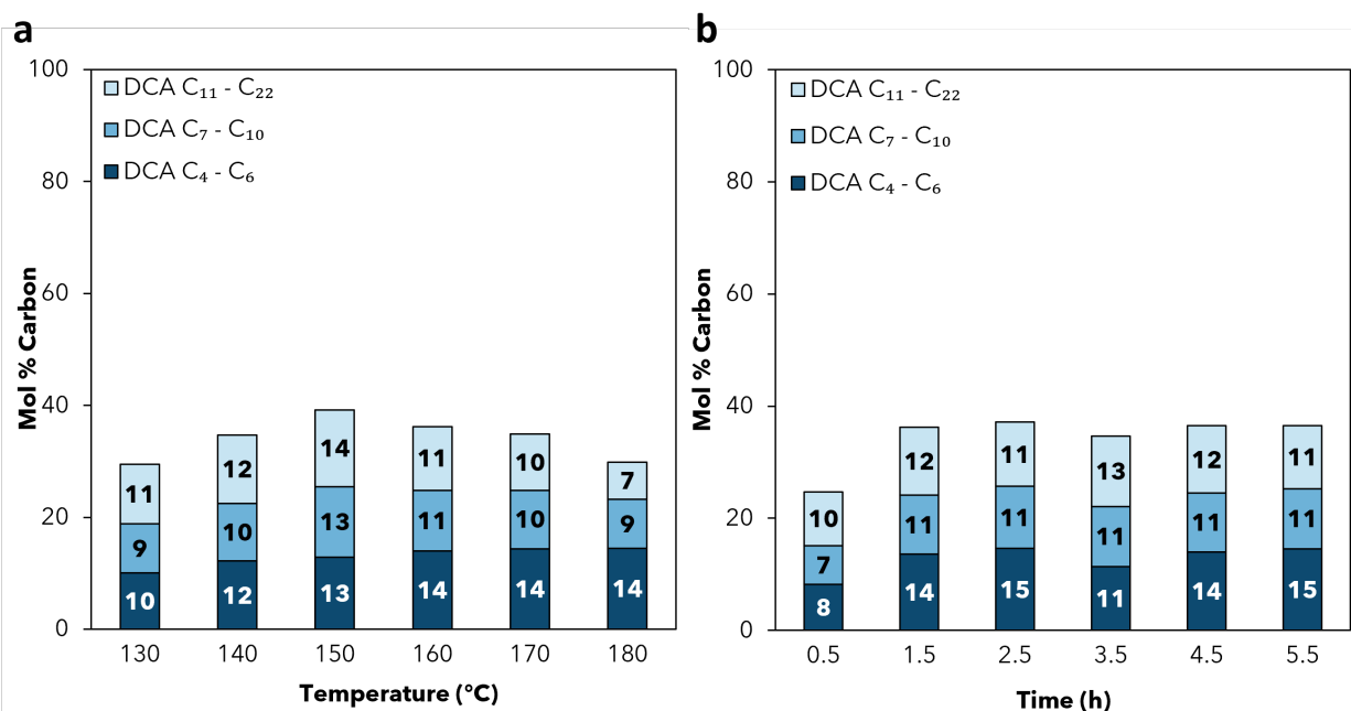
Figure S6. Effect of (a) temperature and (b) time on deconstruction of HDPE beads. Dicarboxylic acid (DCA) product concentrations (C 4 -C 22 ) determined using UHPLC-MS/MS. Mol% carbon yields are calculated as a percentage of carbon in the quantified products relative to the carbon present in the repeating unit of the polymer starting material. Conditions: (a) Temperature screen: 54 kDa HDPE bead (350 mg, 1250 mM repeating ethylene unit), Co(OAc) 2 (9.7 wt%, 9.6 mM), Mn(OAc) 2 (9.5 wt%, 9.6 mM), NHPI (22.4 wt%, 24.0 mM), 8 bar O 2 /72 bar He, 2.5 hr, 130-180 °C. (b) Time screen: 54 kDa HDPE bead (350 mg, 1250 mM repeating ethylene unit), Co(OAc) 2 (9.7 wt%, 9.6 mM), Mn(OAc) 2 (9.5 wt%, 9.6 mM), NHPI (22.4 wt%, 24.0 mM), 8 bar O 2 /72 bar He, 0.5-5.5 hr, 160 °C.
