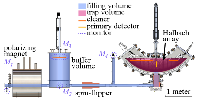
FIG. 1. The UCN \tau apparatus configuration for the 2018 campaign, with the volumes occupied by UCNs, cleaner surfaces, primary detector, and monitors highlighted. The polarizing magnet selects the high-field-seeking UCNs. UCNs are then “precleaned” in the buffer volume, spin-flipped to the trappable low-field-seeking spin state, and loaded into the trap. The 2017 configuration was the same as that of Ref. [29].
