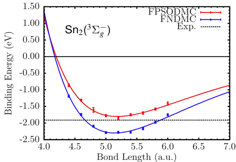
Binding energy of \text{Sn}_2 impact of SOC
