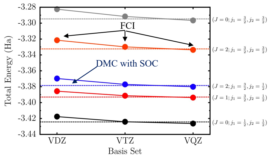
Total Energies of Pb with Large Core REP
