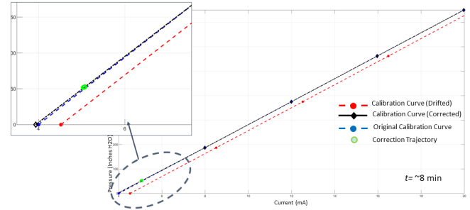
Figure 4. Online recalibration at t \approx 8 min, corresponding to normal (no drift) case.
