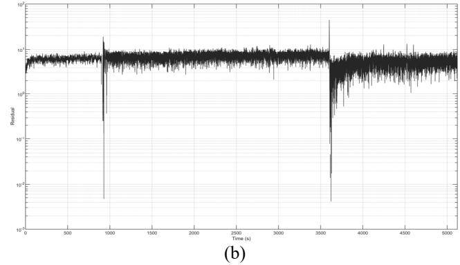
Figure 8. Drift detection and online automated recalibration for DP sensor with sensing line blockage on the low-pressure side. (a) Measured data and autocalibration (b) Residual between measured and predicted values.
