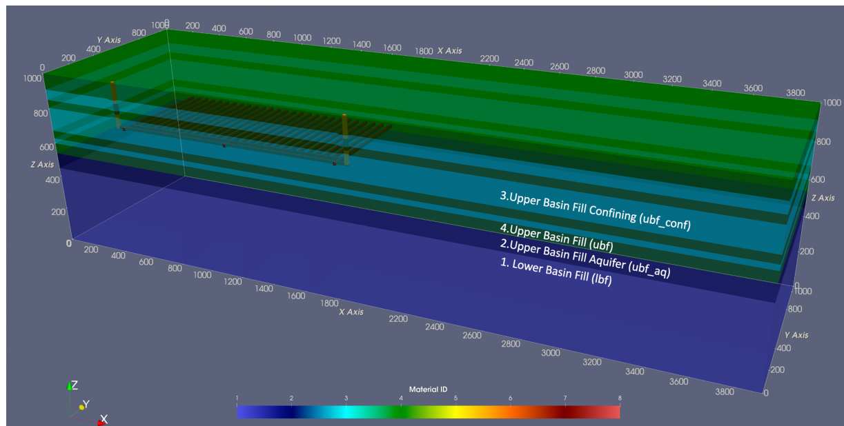
Figure 5-3. Configuration of the repository and natural barrier system generated using Cubit, simulated in PFLOTRAN and visualized on ParaView. Turquoise color (material ID 3) represents the ubf_conf units (the centermost contains the repository as seen there), green (material ID 4) represents UBF, dark blue (material ID 2) represents the UBF aquifer, and blue (material ID 1) represents LBF. Distances along the axes are in meters, where 1000 m is land surface and 0 m is the bottom of the model domain. The left side of the figure represents a western direction.
