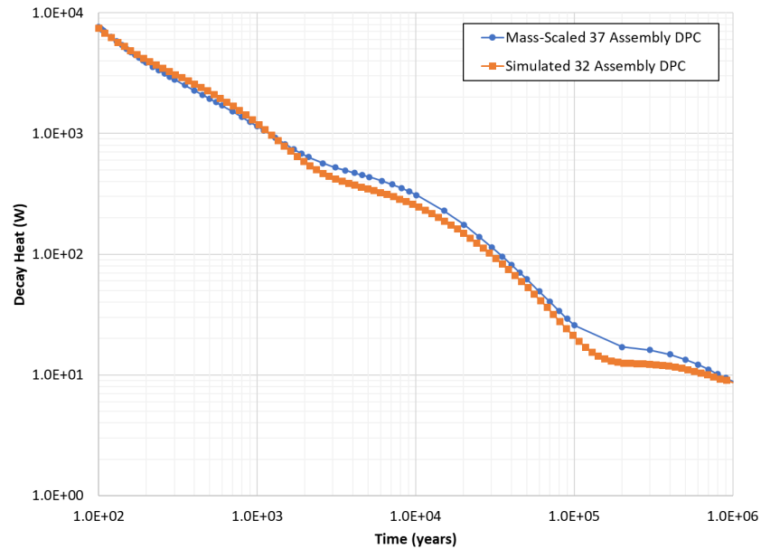
Figure 6-4. Comparison of the decay heats of the simulated 32 assembly DPC and the hypothetical 37 assembly DPC used in previous PA simulations scaled to 32 assemblies.
