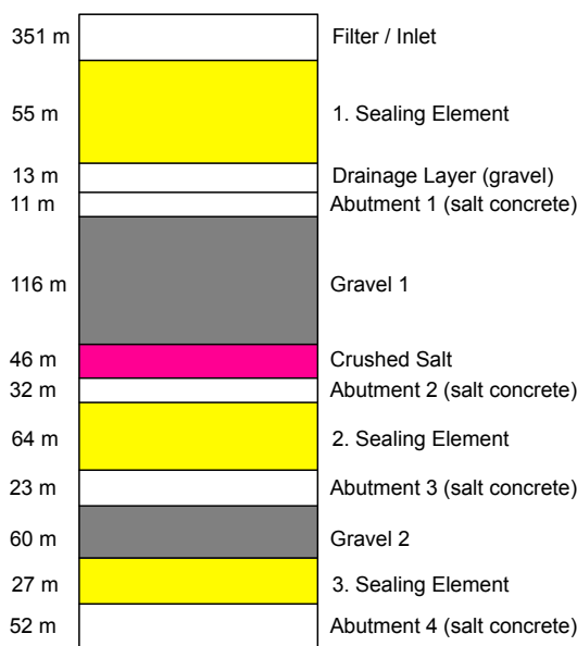
Figure 2-25. Shaft seal for generic salt dome repository (modified from Rübél et al. (2016) by Richard Jayne).
