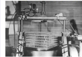
Figure 2. Array of 6.5-in. Cubes Prior to Insertion.
