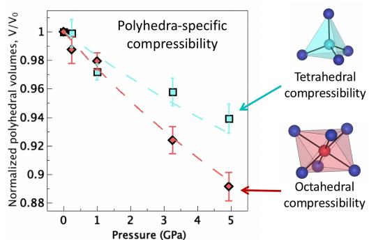
Octahedral Mg-Sb bonds are significantly more compressible than the tetrahedral Mg-Sb bonds in Mg_3Sb_2
