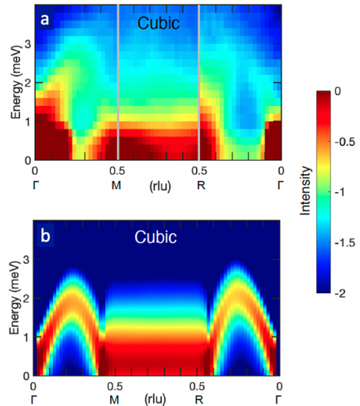
Overdamping of phonon modes along M-R in the cubic phase of CsPbBr 3 . (a) INS measurements (b) first-principles simulations of anharmonic damping.
