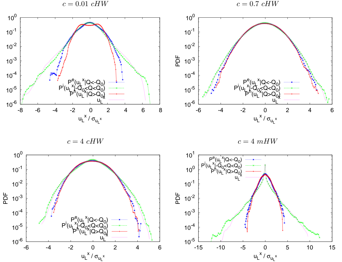
FIG. 9. PDFs (normalized by the corresponding standard deviation) of Lagrangian conditional x -component velocity with respect to three-level Lagrangian Weiss value for cHW with c = 0.01 (top, left), c = 0.7 (top, right), c = 4 (bottom, left) and mHW with c = 4 (bottom, right). The superscripts e , h and i correspond to elliptic, hyperbolic and intermediate regions, respectively.
