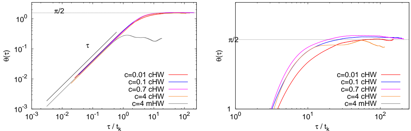
FIG. 13. Mean curvature angle \theta(\tau) as a function of \tau/t_k for the different flow regimes. A corresponding zoom for large increments \tau/t_k is shown on the right.
