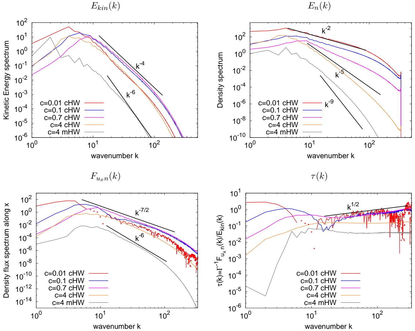
FIG. 3. Top: Eulerian kinetic spectra E_{kin}(k) (left) and Eulerian spectra E_n(k) of density fluctuations (right). Bottom : Density flux spectra F_{u_x n}(k) (left) and spectral timescale \tau(k) = \Gamma^{-1} |F_{u_x n}(k)| / E_{kin}(k) (right). All the spectra are obtained using time-averaging with 75 snapshots taken at regular time intervals in the statistically stationary regimes. Dots in the spectra indicate negative values, plotted by taking the absolute value.
