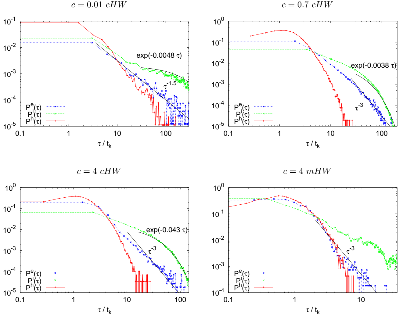
FIG. 8. PDFs (normalized by the mean eddy turn over time) of residence time conditioned with respect to the three-level Lagrangian Weiss value for cHW with c = 0.01 (top, left), c = 0.7 (top, right), c = 4 (bottom, left) and mHW with c = 4 (bottom, right). The superscripts e , h and i correspond to elliptic, hyperbolic and intermediate regions, respectively.
