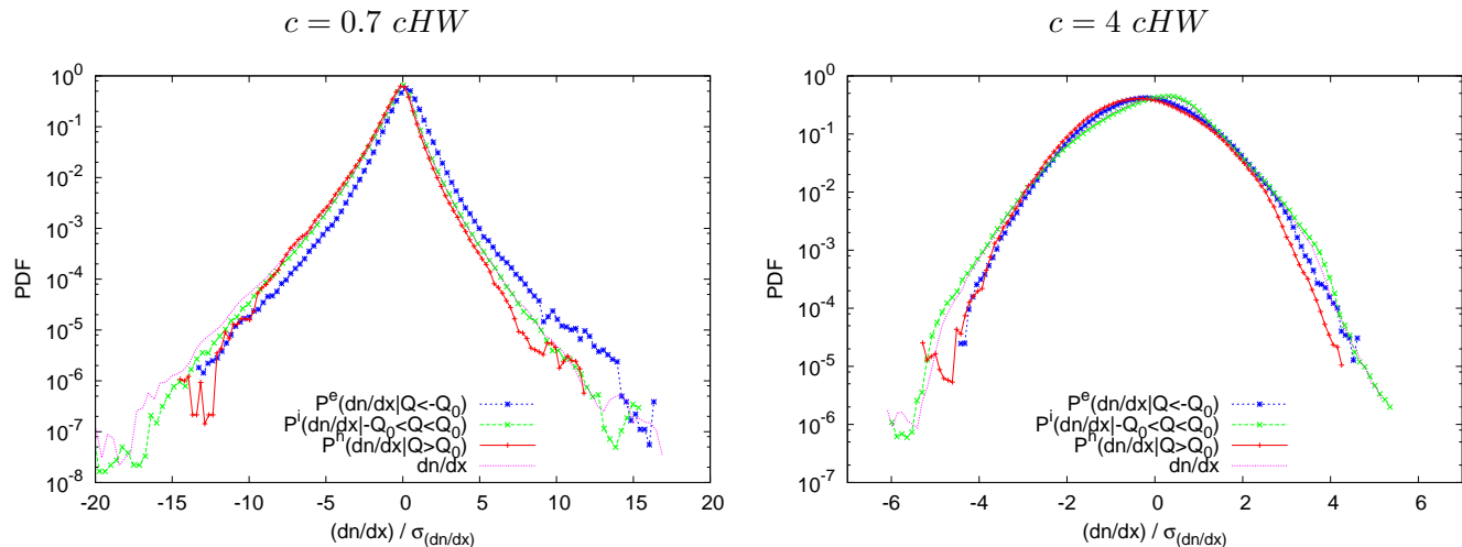
FIG. 12. PDFs (normalized by the corresponding standard deviation) of Lagrangian conditional density gradient in the x -direction with respect to three level Weiss value for cHW with c = 0.7 (left) and c = 4 (right). The superscripts e , h and i correspond to elliptic, hyperbolic and intermediate regions, respectively.
