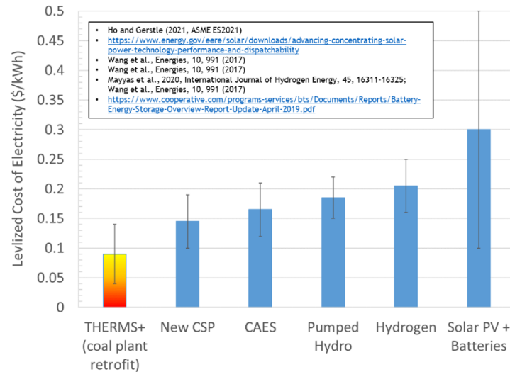
FIGURE 3: Levelized cost of electricity of THERMS+ compared to other technologies
