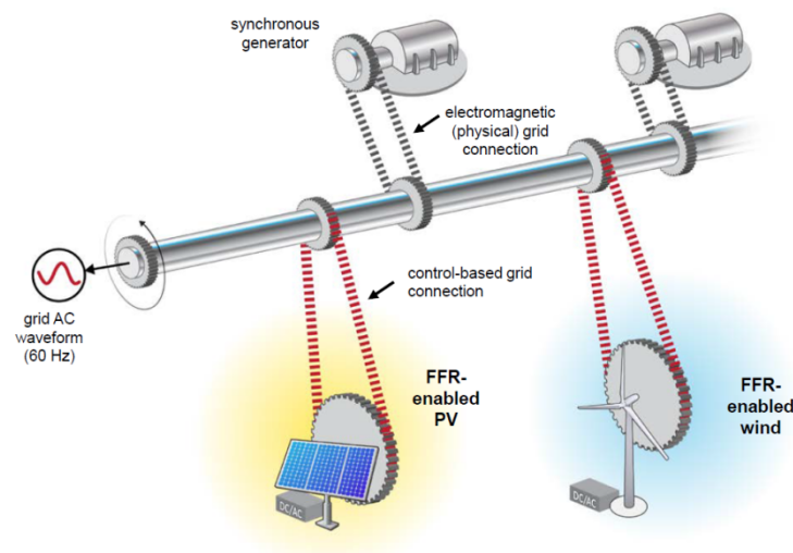
FIGURE 4: Wind and solar providing frequency response through inverter-based (control-based) grid connection [15]
