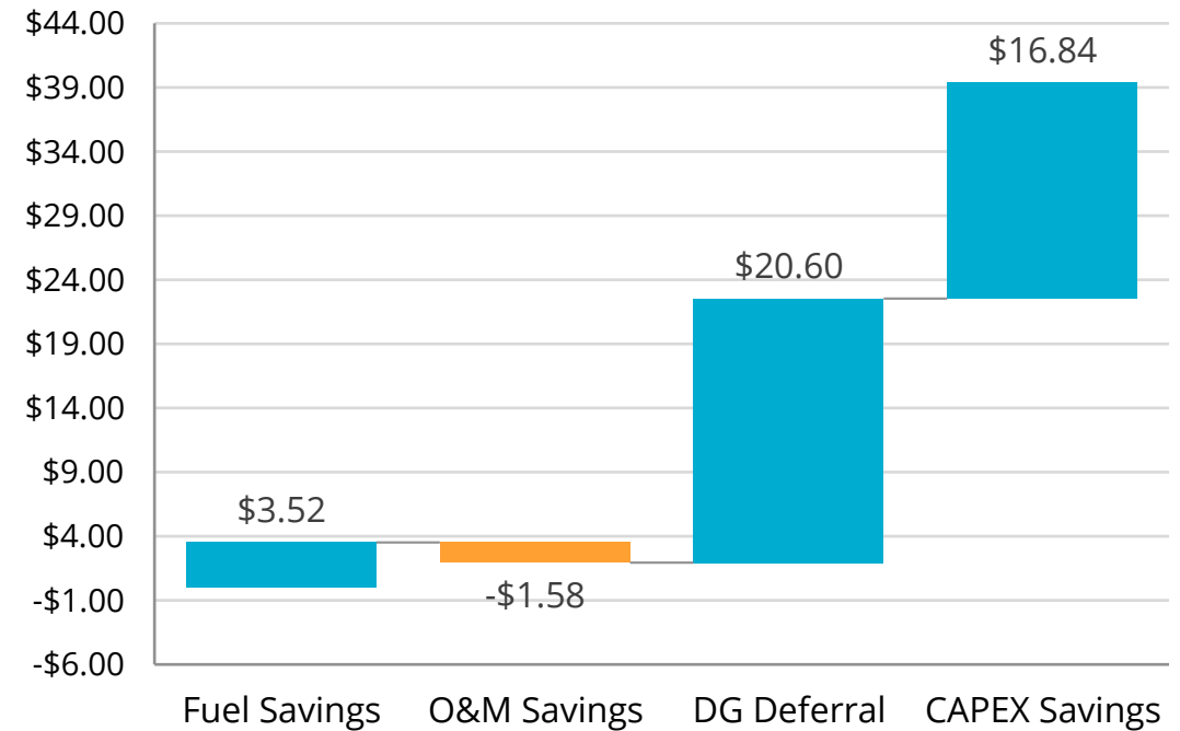
PV of 2 DG, 50 kW/25kWh system versus 3 DG system, 50 kW solar (EOR = 0.57, LPOR = 0.086)
