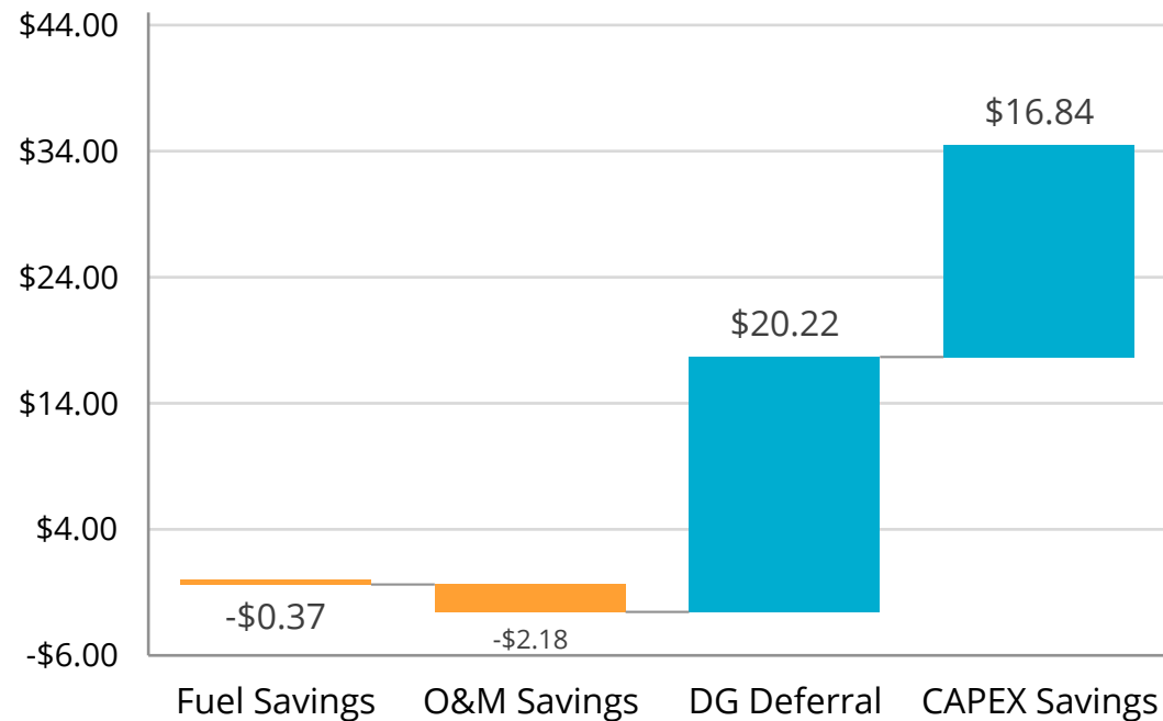
PV of 2 DG, 50 kW/25kWh system versus 3 DG system, no solar (EOR = 0.29, LPOR = 0.0001)
