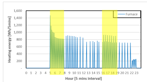
Figure 9 Heating energy consumption pattern of the gas furnace on the winter representative day (on-peak hours)
