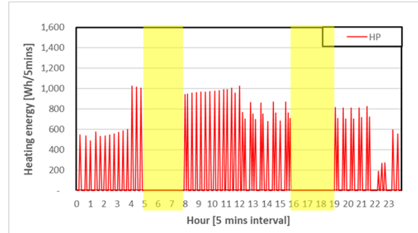
Figure 8 Heating energy consumption pattern of the HP on the winter representative day (on-peak hours)
