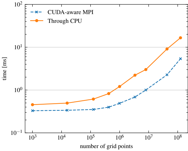
Figure 3.2: Comparing performance of halo exchange for 7-point stencil using CUDA-aware MPI and passing through CPU on 512 GPUs on Lassen.
