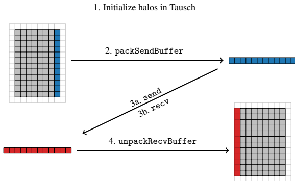
Figure 2.2: High-level overview of Tausch.
