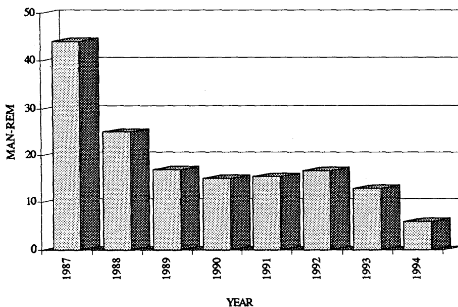
Figure 4.6 Population Dose From Airborne Radioactive Emissions
