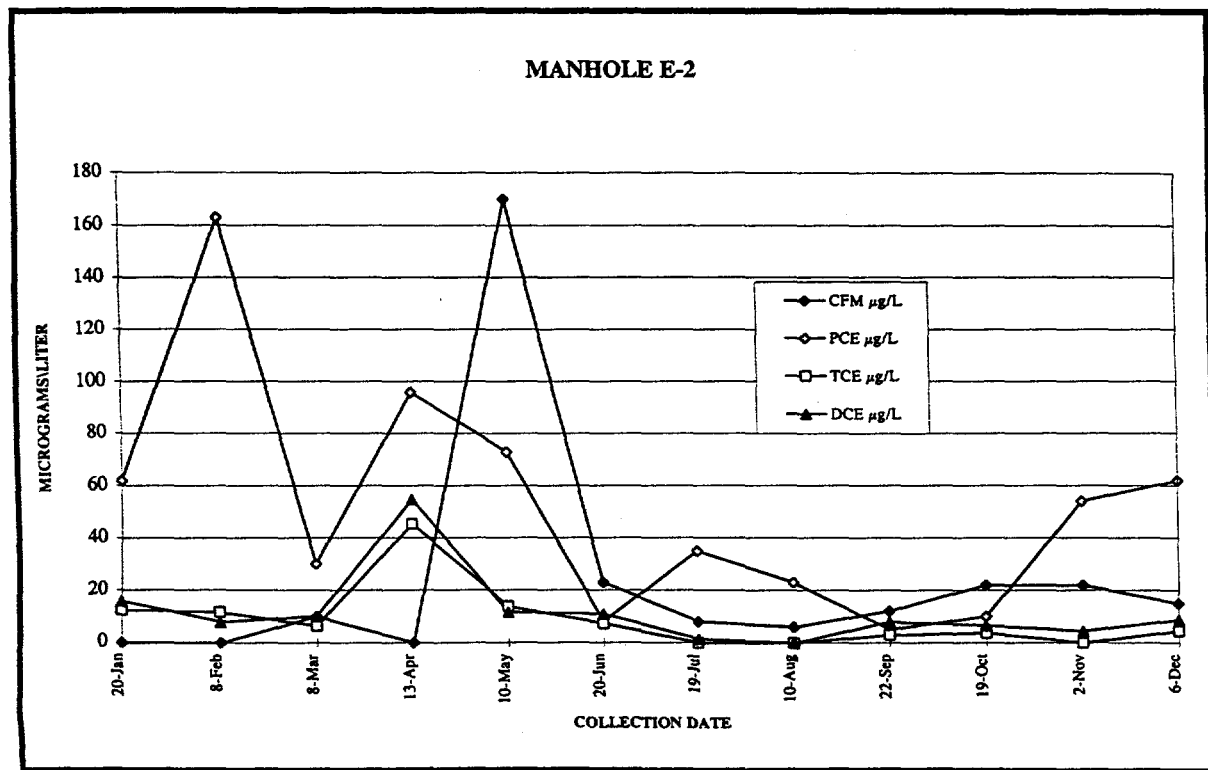
Figure 6.5 Trends of Selected Organics in 317 Area Manholes, 1994
