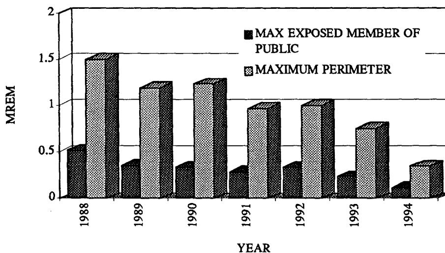
Figure 4.5 Individual and Perimeter Doses From Airborne Radioactive Emissions
