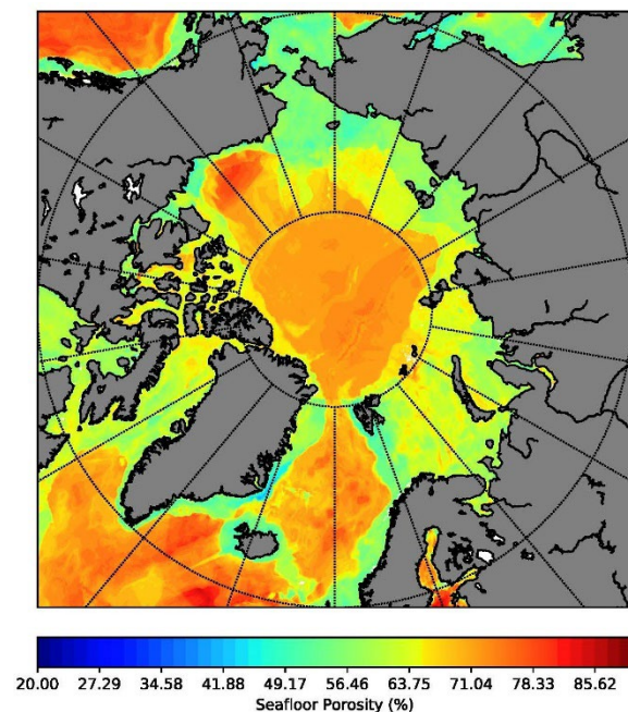
Figure 2. Seafloor porosity predicted by GPSM using geospatial machine learning. (Martin et al., 2015)
