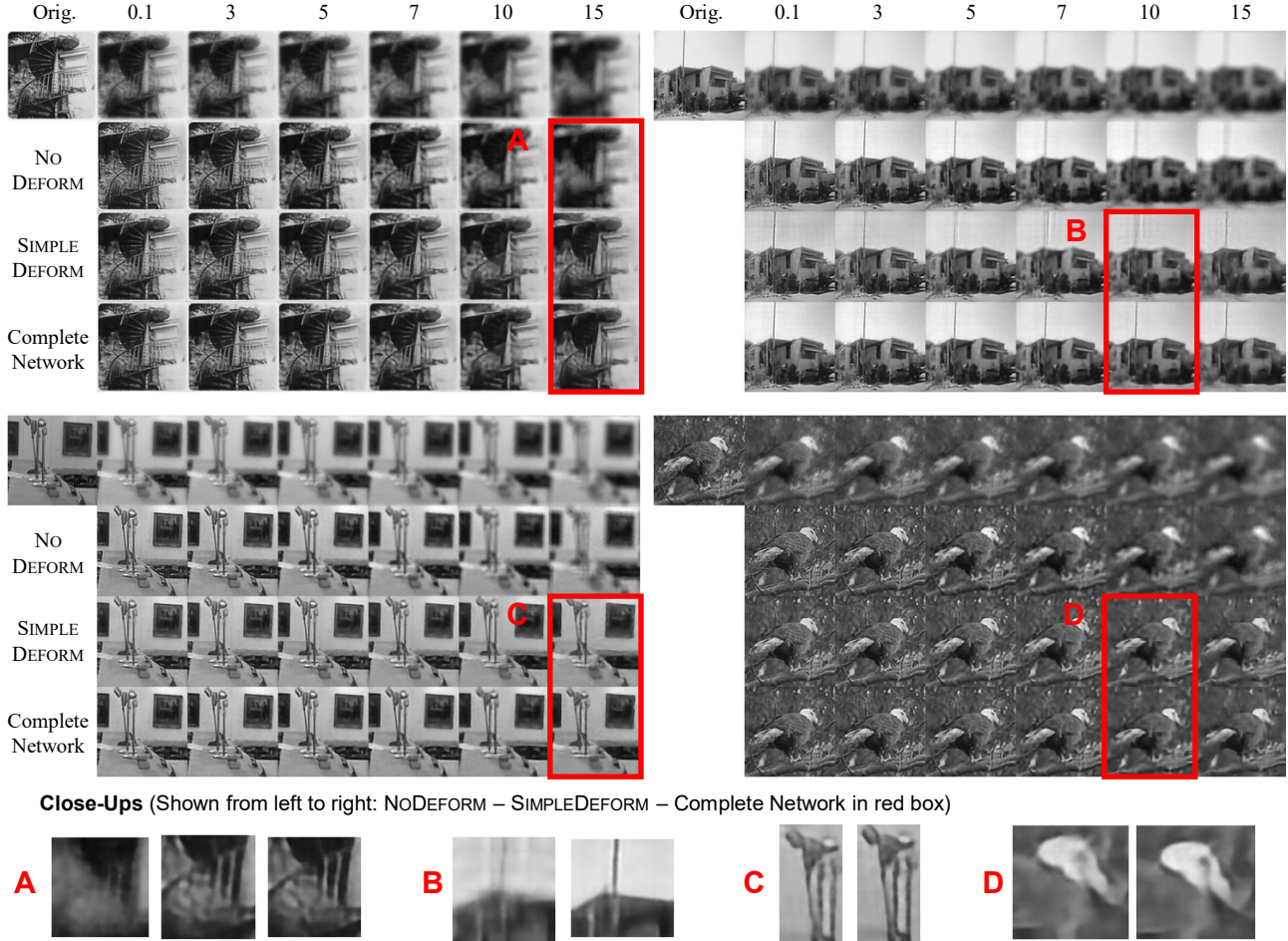
Figure 5. Comparison of NODEFORM, SIMPLEDEFORM and the complete deformation network.
