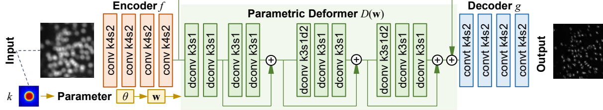
Figure 1. Architecture of the latent space deformation network. For brevity, nonlinear activations, batch normalizations, and hidden layers to encode the parameter w are not shown. conv, convt and dconv stand for convolution layer, convolution transpose layer, and dynamic convolution, respectively. k3s1d2 means kernel size 3, stride 1, dilation 2. All convolutions are 1-dilated unless otherwise noted.
