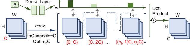
Figure 4. Structure of a dynamic convolution. The middle tensor in brackets [\dots] has n_b C channels as a result of the convolution, which are spread out as n_b groups to take the dot product as described in Eqn. 8.
