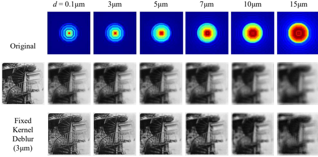
Figure 2. An example set of NBDs with varying kernels. Top: six kernels with different defocal distances. All kernels are scalar real-valued intensity maps, colored with false color for visualization purposes. Center: the original clean image and the blurred images from the kernels above. Bottom: an encoder-decoder deblurring network trained with the 3\mu\text{m} kernel fails to deblur images from other kernels.
