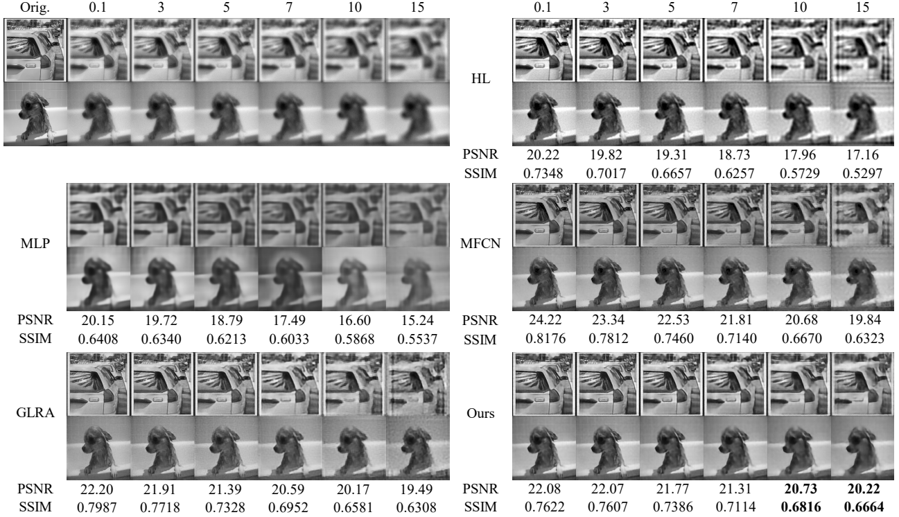
Figure 6. Comparisons of different NBD methods. Here we report the mean PSNR and mean SSIM per kernel on the testing set.
