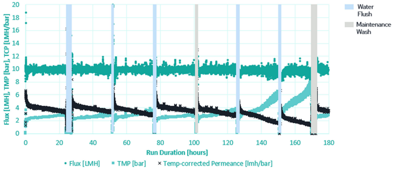
Figure 2: 168-hour continuous run at 10 lmh, 99% recovery, and uptime of >95%
