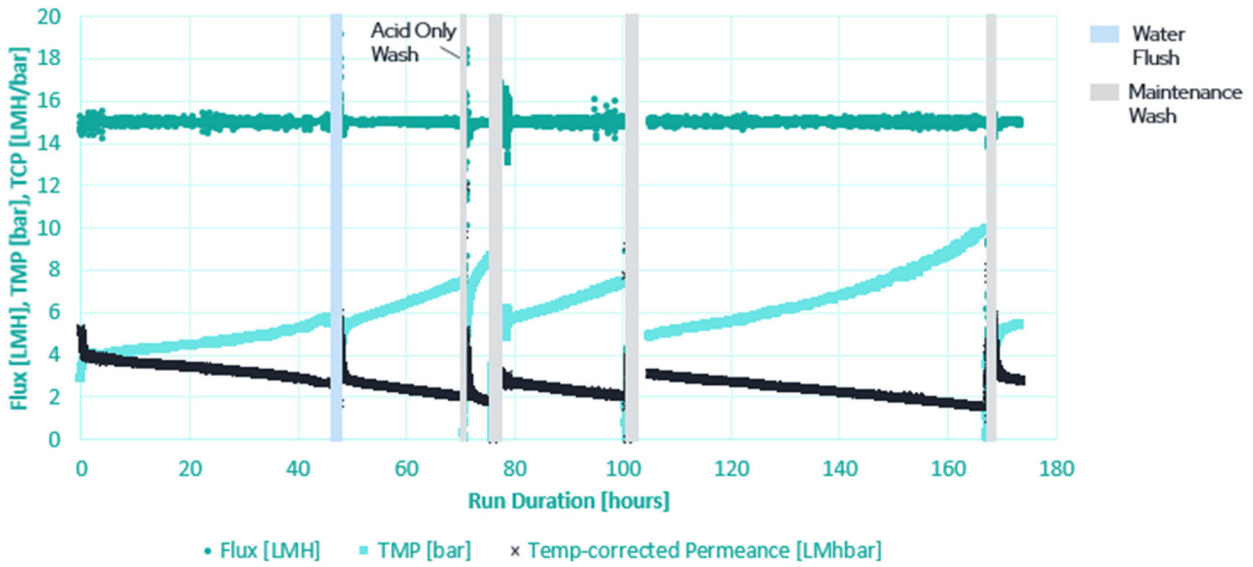
Figure 3: 168-hour continuous run at 15 lmh, 95% recovery, and uptime of >95%
