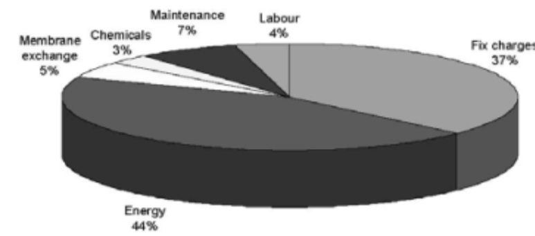
Fig. 50. Water distribution cost in an SWRO plant
