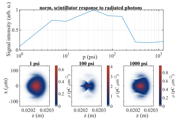
Figure 7: Scan of backing pressure to the hydrogen gas jet potentially showed a reduction in signal at gamma diagnostics at higher pressures.
