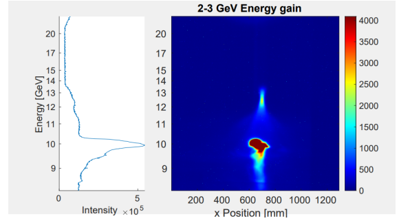
Figure 6: Electron energy gain from 10 GeV up to 13 GeV with 2 m-long hydrogen plasma
