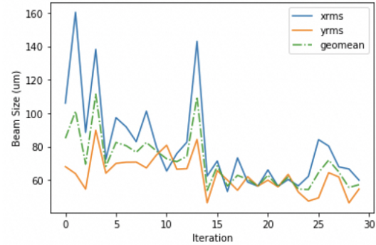
Figure 3: Machine learning applied to sextupole adjustments for beam size optimisation at a wire scanner in the interaction area.
