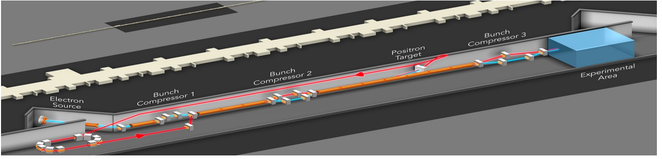
Figure 1: Layout of FACET-II. The facility is 1 km long comprising a photo-cathode injector, three accelerating sections, three bunch compression sections and a final section where experiments are staged. The current installation is compatible with a possible future upgrade to deliver positrons.
