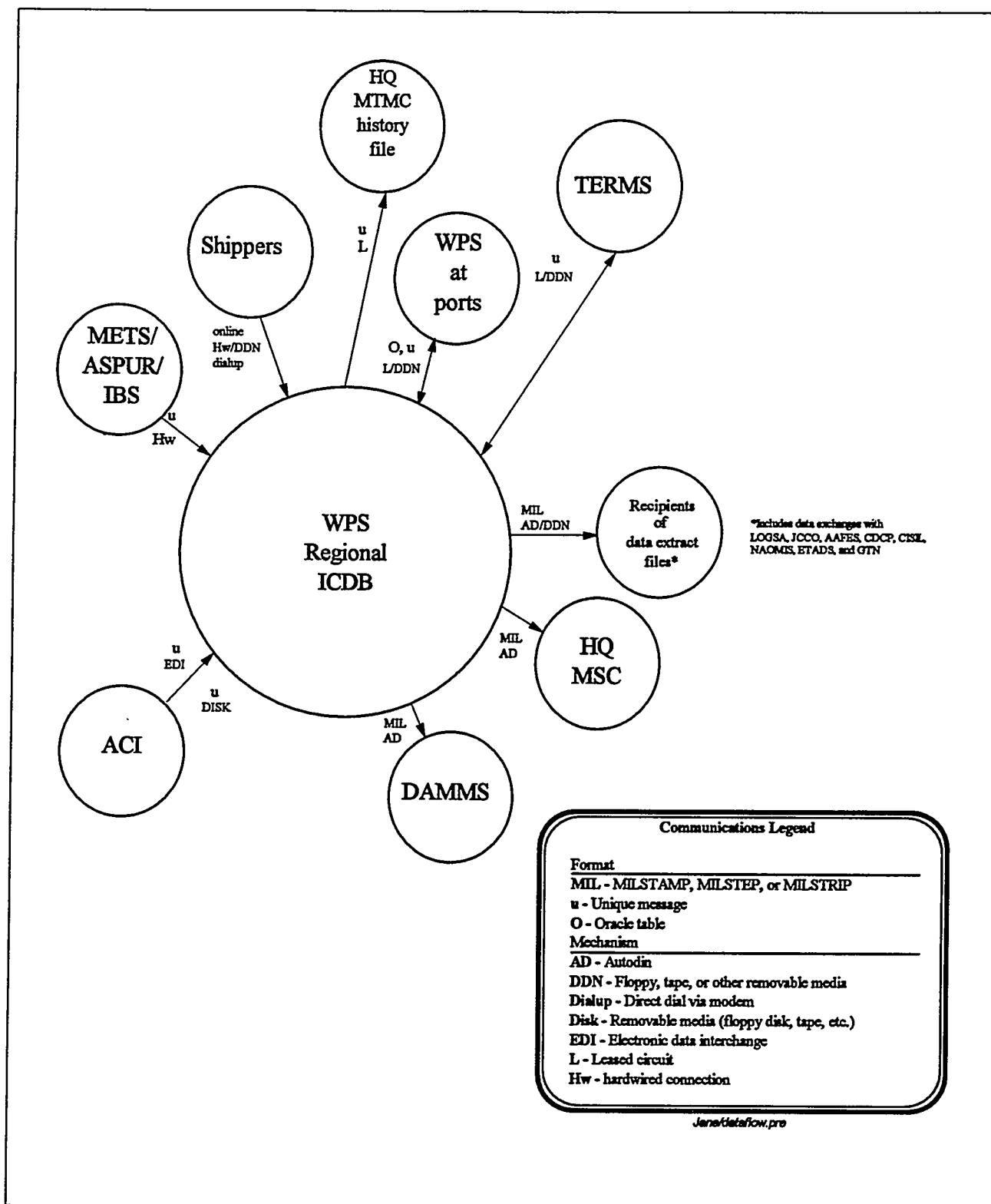
Figure 3.3. The systems and organizations with which ICDB interfaces.
