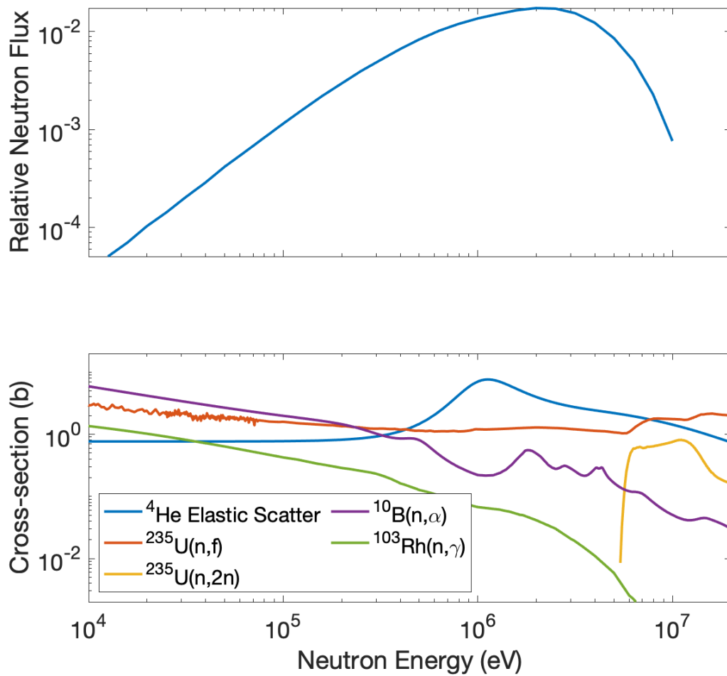
Figure 1: Typical fission neutron energy spectrum (above). Cross-sections of several reactions of interest for fast neutron detection (below). [3]
