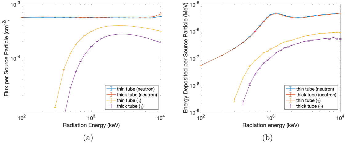
Figure 2: (a) Simulated neutron and gamma-ray flux inside each tube as a function of source radiation energy. (b) Simulated neutron and gamma-ray energy deposition in the active volume as a function of source radiation energy.
