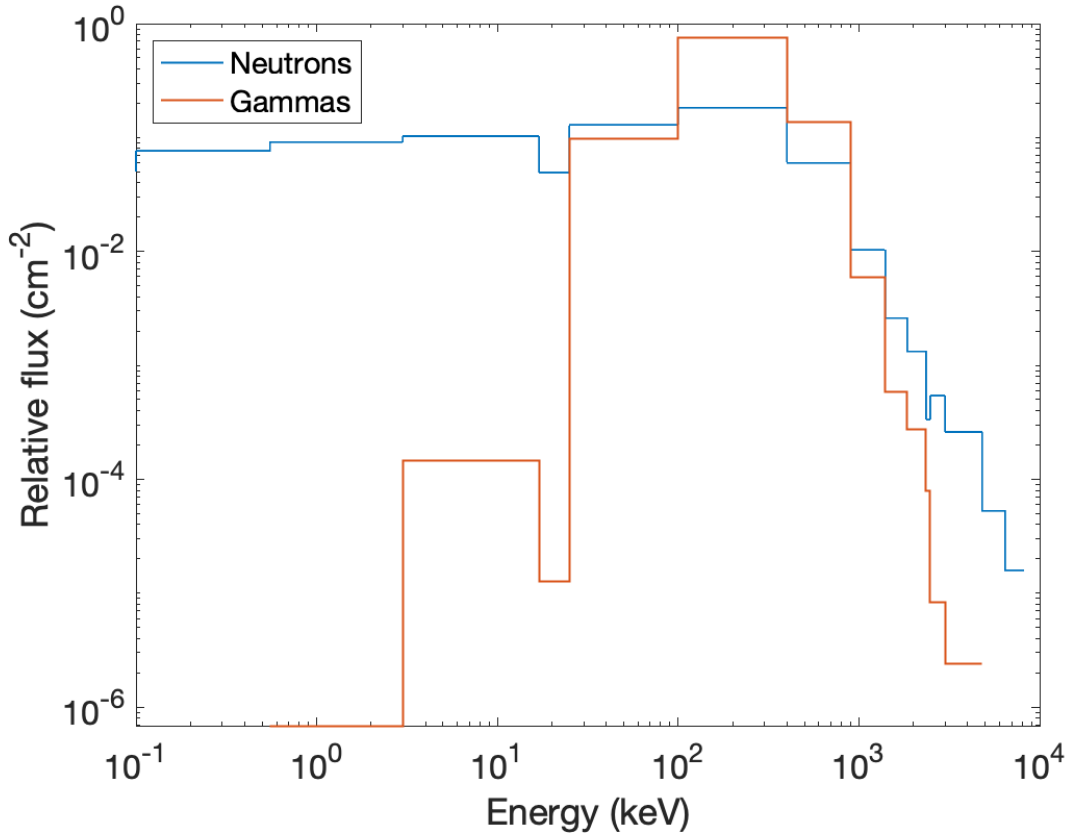
Figure 3: The simulated relative neutron and gamma-ray flux in the air gap of the SNF cask
