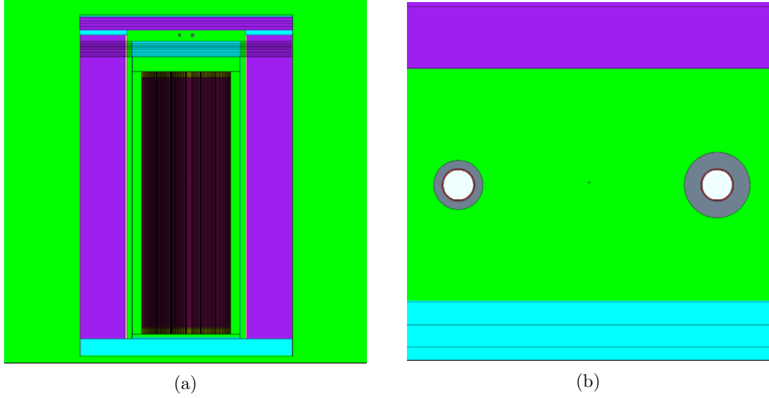
Figure 4: (a) MCNP-generated image of the SNF cask with the ^4\text{He} detector prototype. (b) Magnified view on the ^4\text{He} detector prototype modeled in the air gap between the MPC and concrete cask lid.
