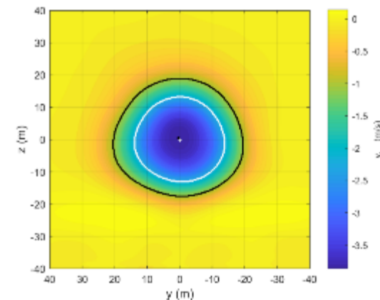
Average over 10 minutes for the simulated wake data 5D downwind, sampled to match the experimental lidar data.
