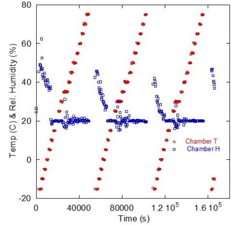
Fig. 7. Environmental chamber conditions versus time for the data shown in Fig. 8
