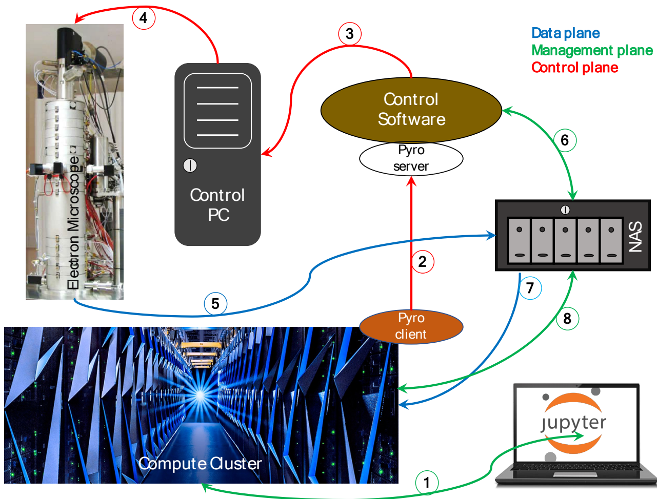
Figure 1. Interconnectivity workflow between the microscope and the computational facilities. The connectivity can be split into three distinct planes – data (moving around the microscope data), management , and control (commands to the microscope for operation).
