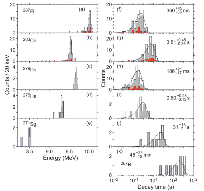
FIG. 1. \alpha -particle energy spectra (a)–(e) and decay-time distributions on a logarithmic scale (f)–(k) for ^{287}\text{Fl} , ^{283}\text{Cn} , and descendant nuclei. The data observed in this work and a summary of known results are shown by gray and open histograms, respectively. \alpha -particle energies and decay times of ^{287}\text{Fl} and ^{283}\text{Cn} followed by \alpha decay of ^{279}\text{Ds} as well as lifetimes of \alpha decays of ^{279}\text{Ds} are shown in red. The smooth curves are the time distributions for exponential decays calculated with the half-lives T_{1/2} shown in the figures.
