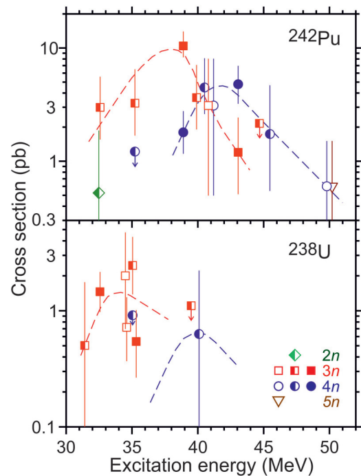
FIG. 3. Cross sections for the 2n - to 5n -evaporation channels for the ^{242}\text{Pu} + ^{48}\text{Ca} and ^{238}\text{U} + ^{48}\text{Ca} reactions. Vertical error bars correspond to total uncertainties. Symbols with arrows show upper cross-section limits. Data shown by open, half-closed, and closed symbols are from [11,15,18], [7], and this work, respectively. The dashed lines through the data are drawn to guide the eye.
