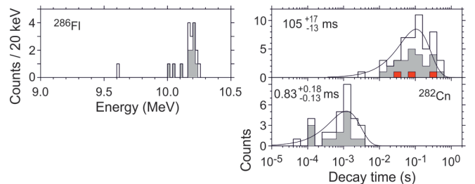
FIG. 2. The same as in Fig. 1 but for ^{286}\text{Fl} . Decay times of the three low- E_\alpha events of ^{286}\text{Fl} are shown in red.
